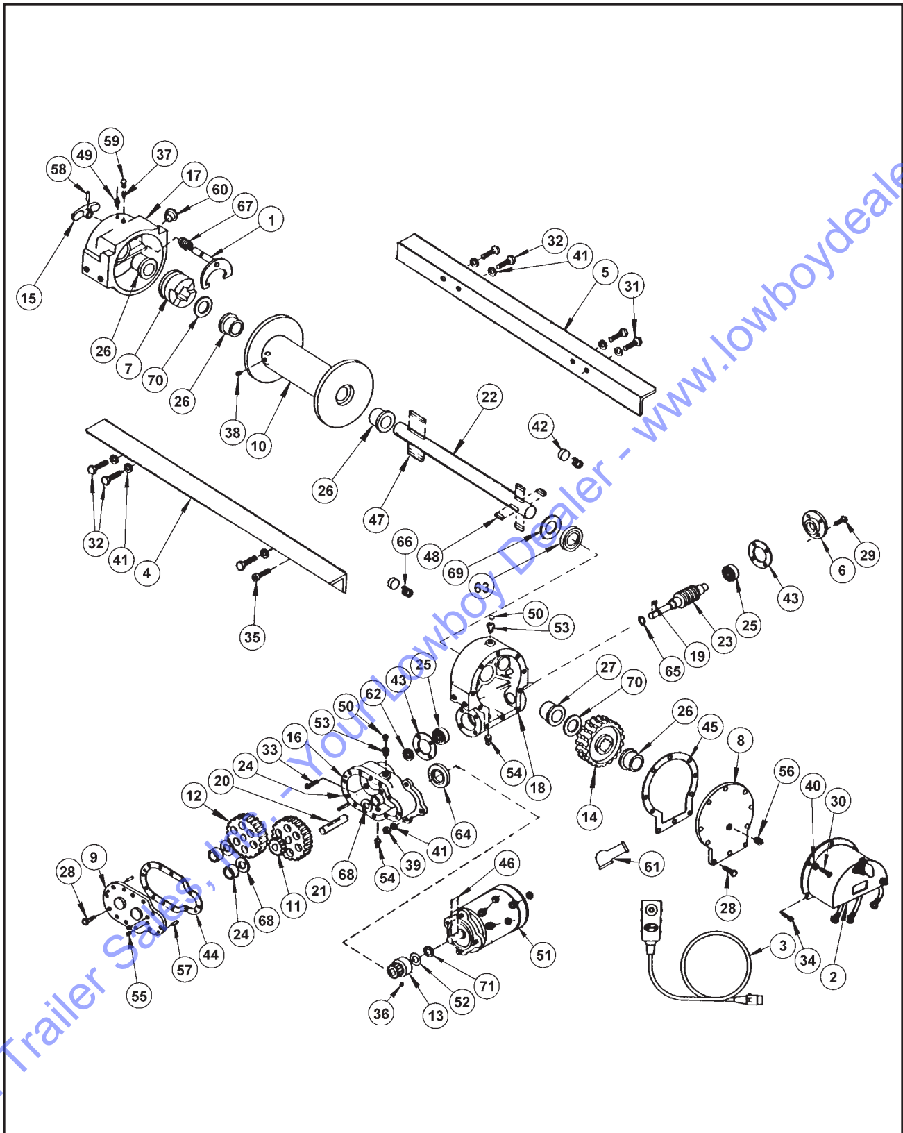
Figure 1-26 Winch Assembly
