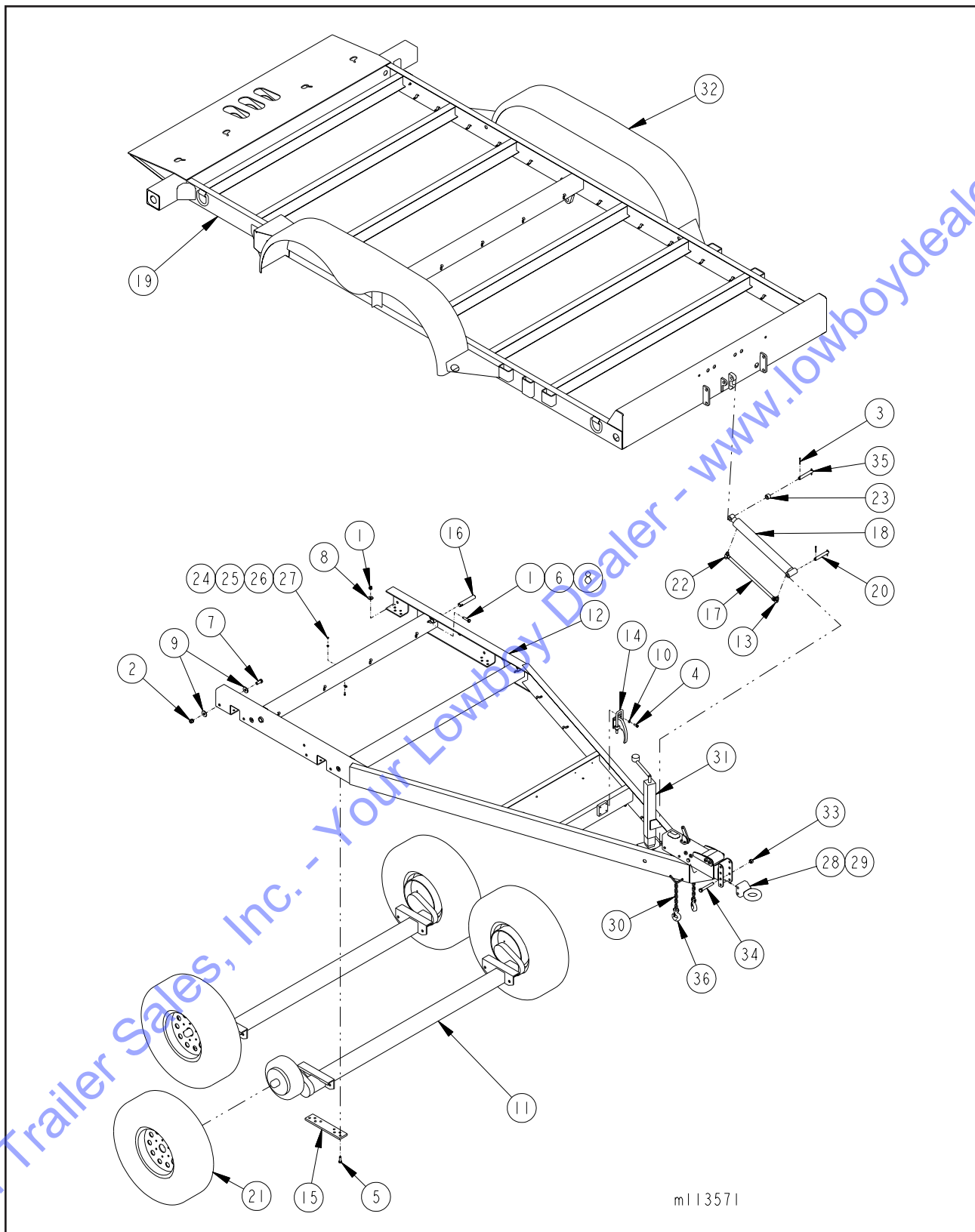
Figure 1-7 Trailer Assembly (Surge Brakes) (LT816 & LT1016) (1 of 2)
