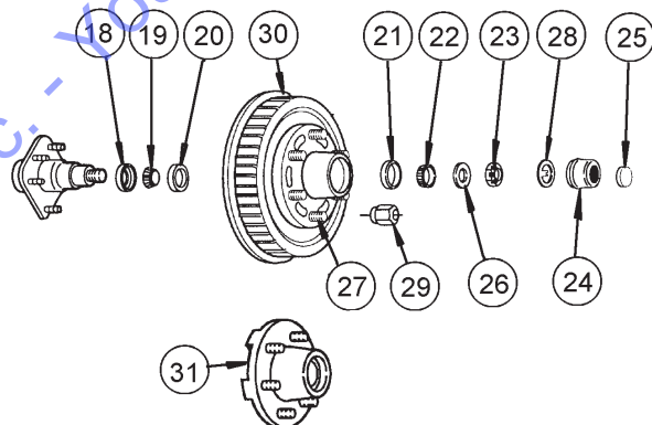
HUB AND DRUM ASSEMBLY, 6 BOLT
