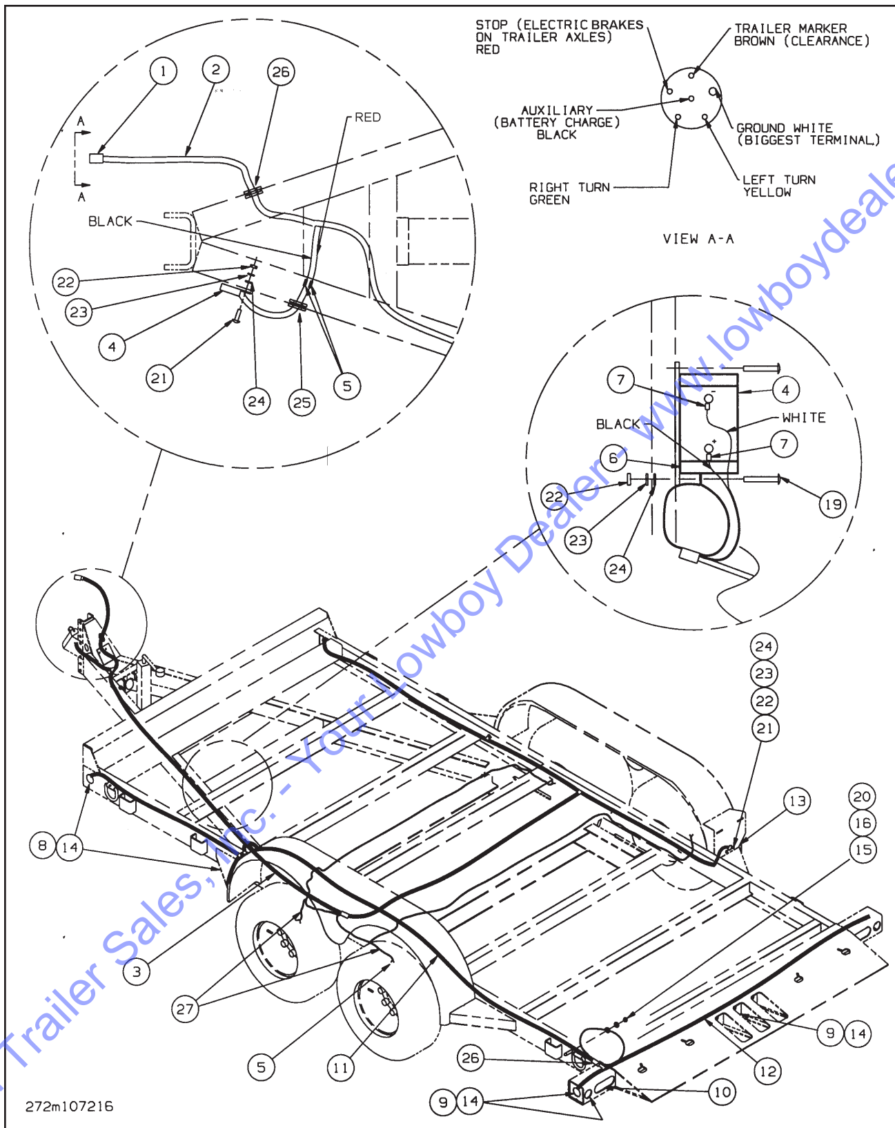
Figure 1-18 Electrical Assembly w/ Pintle Hitch
