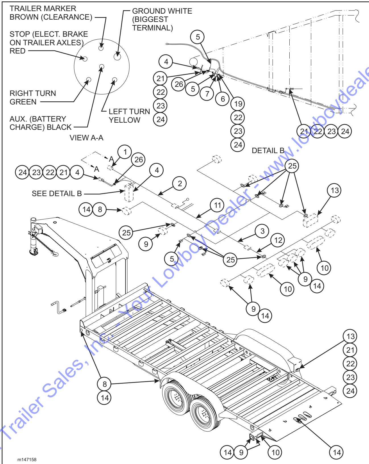
Figure 1-19 Electrical Assembly w/ Gooseneck Hitch
