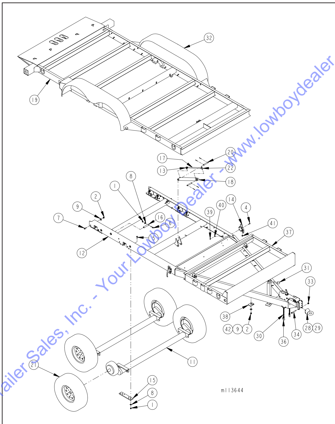
Figure 1-8 Trailer Assembly (Surge Brakes) (LT1016-4 & LT1216-4) (2 of 2)
