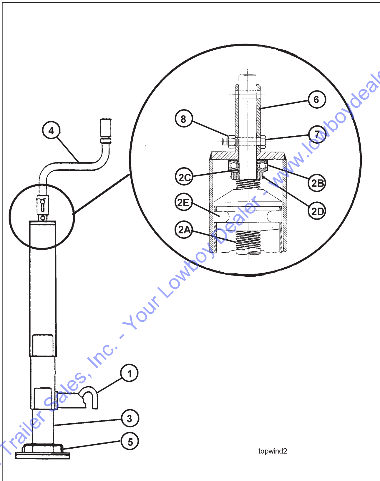
Figure 1-28 Jackstand Assembly (Pintle Hitch)
