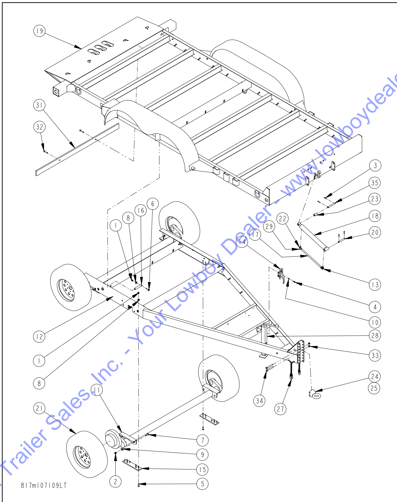
Figure 1-2 Trailer Assembly w/ Pintle Hitch (Electric Brakes) (LT816, LT1016, LT1020, & LT1220) (1 of 3)
