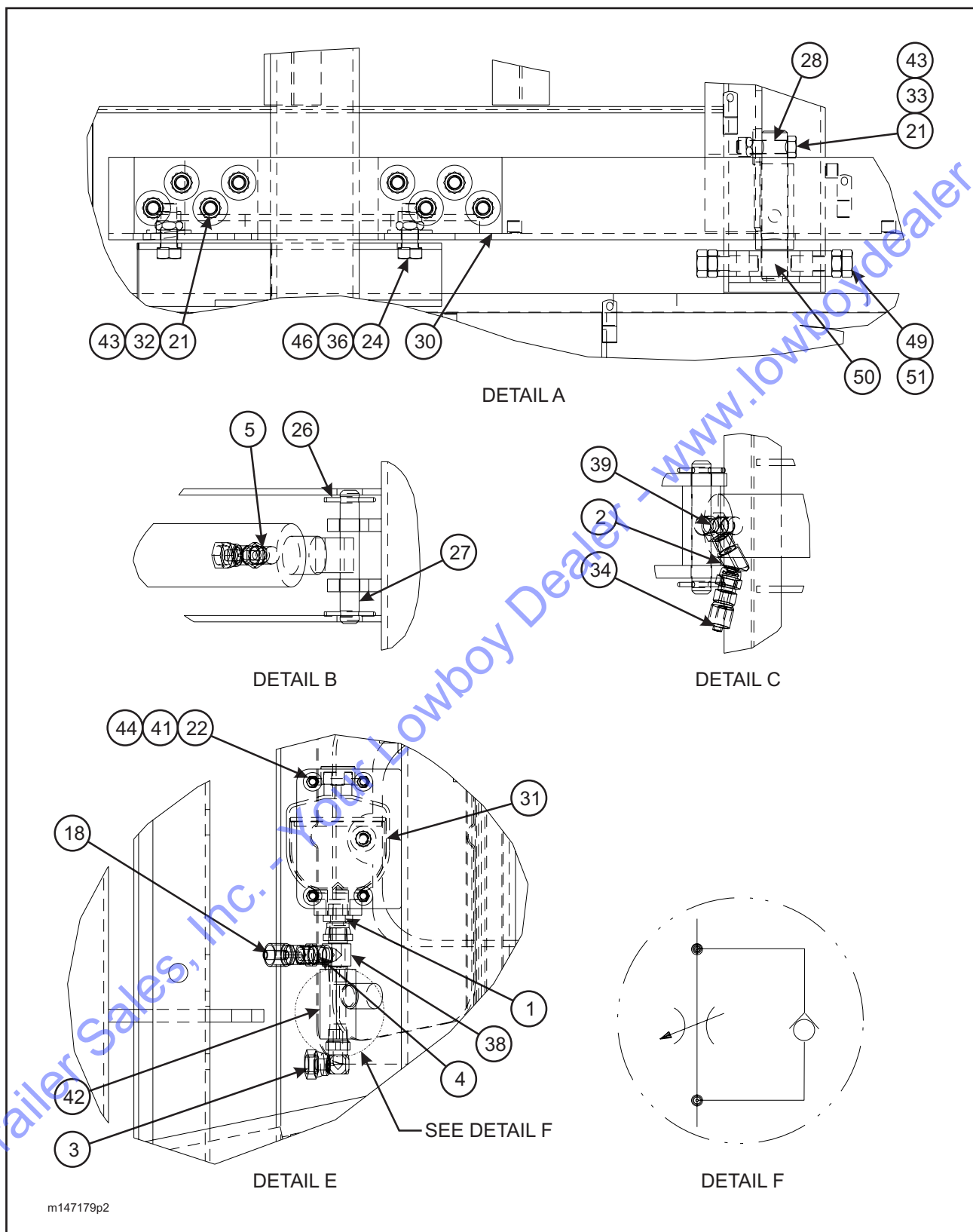
Figure 1-6 Trailer Assembly w/ Gooseneck Hitch (Electric Brakes) (LT1220 and LT1420) (2 of 2)
