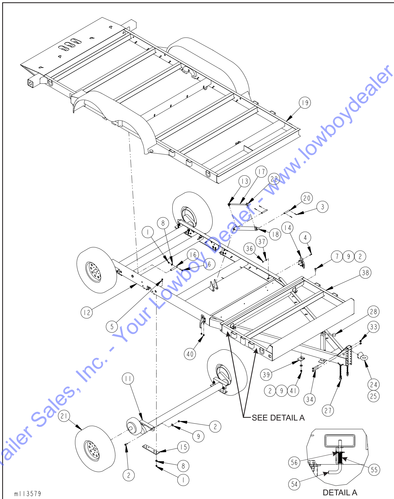
Figure 1-3 Trailer Assembly w/ Pintle Hitch (Electric Brakes) (LT1016-4) (2 of 3)
