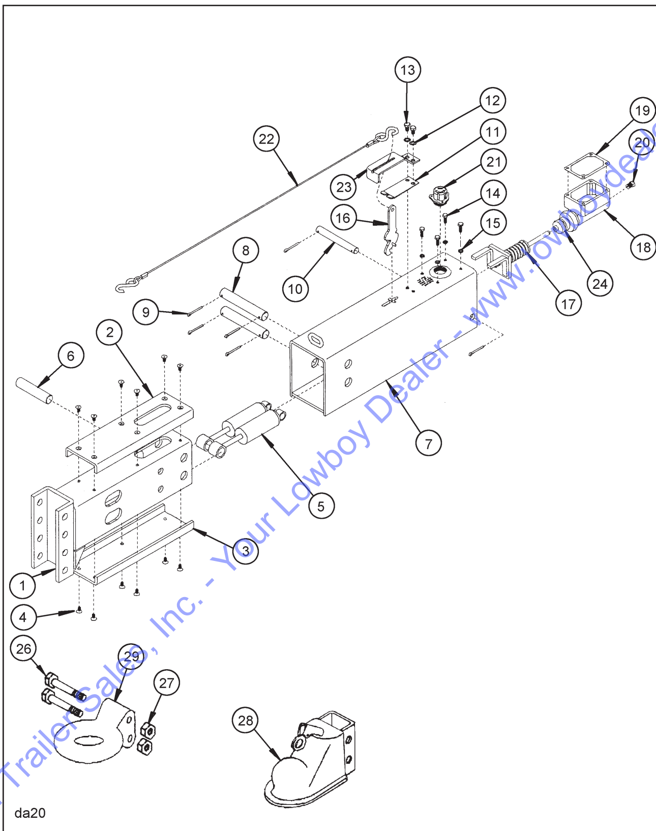
Figure 1-16 Surge Brake Actuator Assembly
