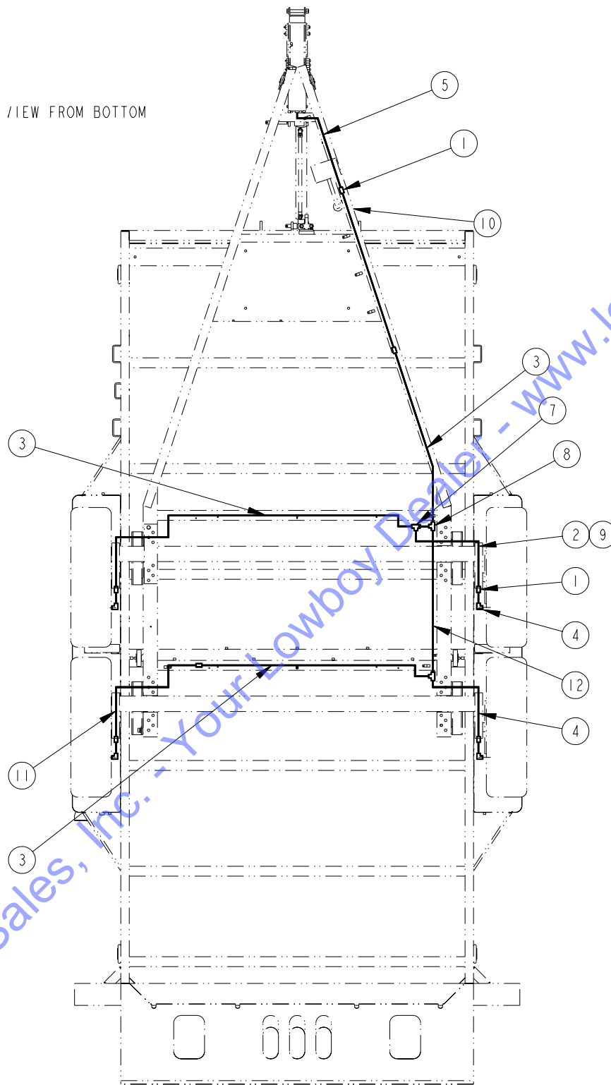
Figure 1-9 Surge Brake Line Schematic
