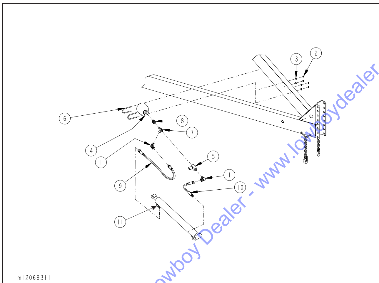
Figure 1-24 Tilt Lock Assembly (Option) (Used on Models LT816 and LT1016 )
