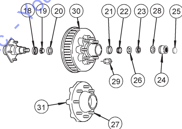
HUB AND DRUM ASSEMBLY, 8 BOLT
