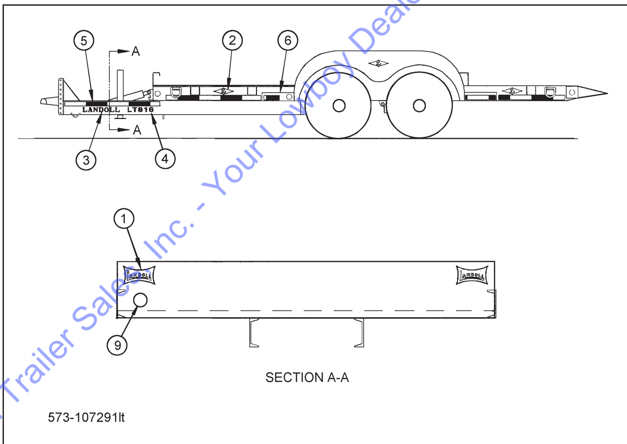
Figure 1-21 Decal Assembly
