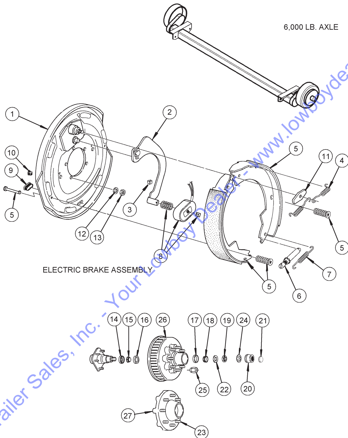
Figure 1-11 6000# E-Z Lube Axle Assy 8 Bolt
