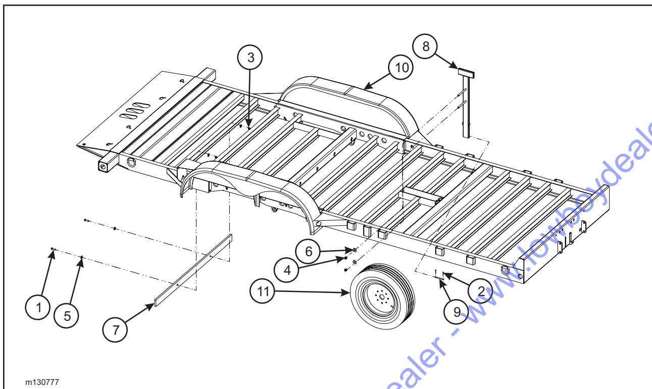
Figure 1-30 Spare Tire Mounting Kit (Option)
