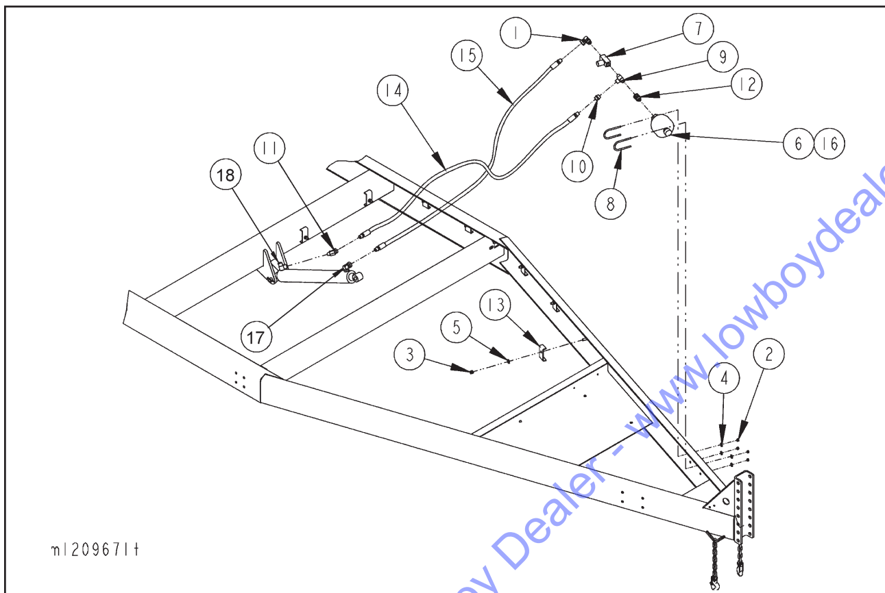
Figure 1-23 Tilt Lock Assembly (Option) (Used on Models LT1016-4, LT1020, LT1216-4, LT1220 & LT1420)
