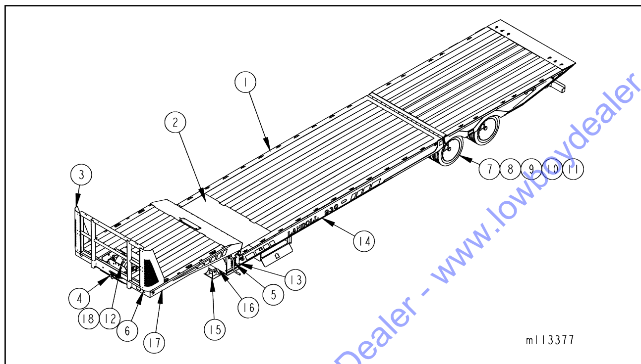
Figure 1-1 General Assembly
