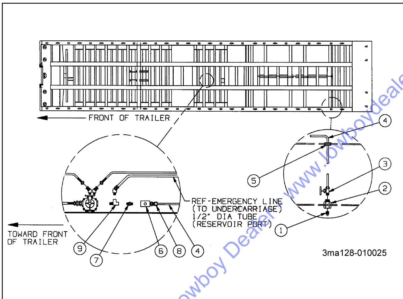
Figure 1-59 Air Outlet Assembly (Optional)
