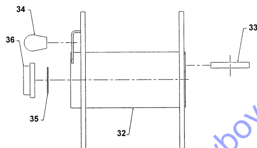
DRUM INSTALLATION
