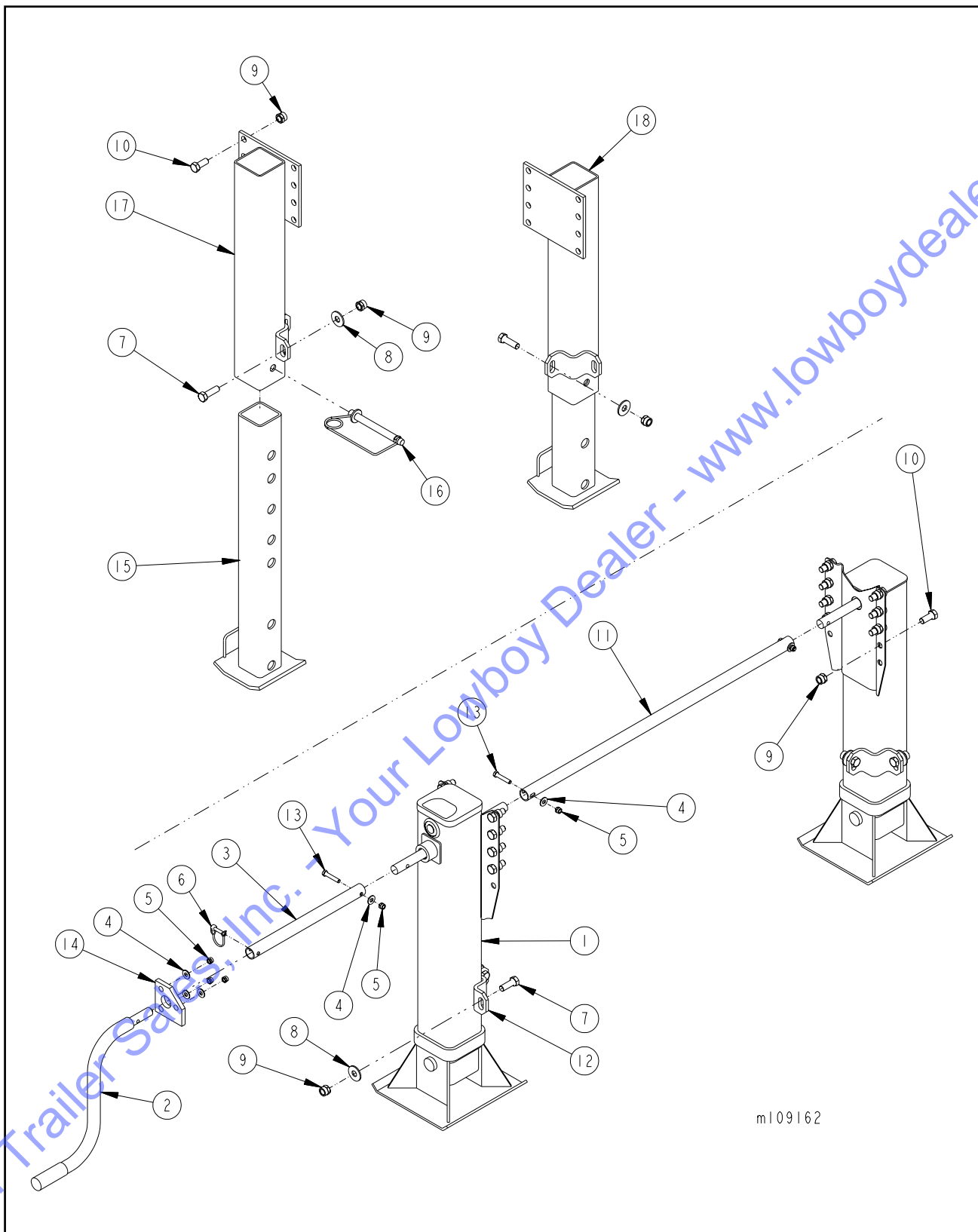
Figure 1-48 Landing Gear
