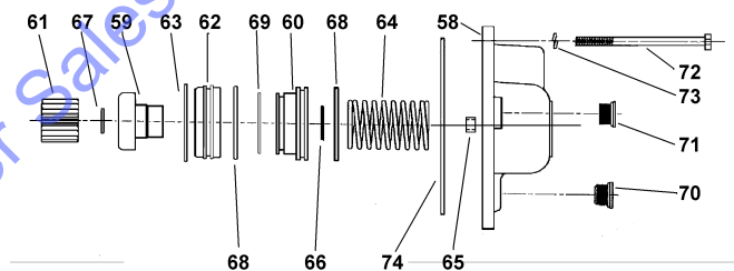
BASE INSTALLATION
