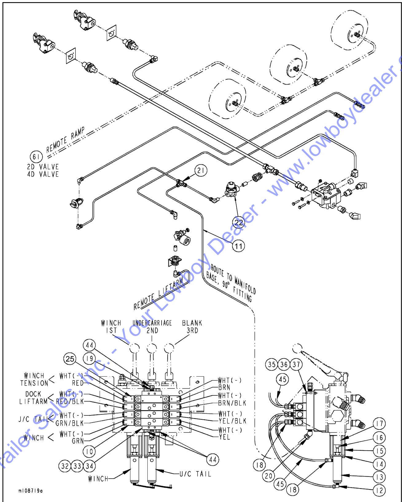
Figure 1-42 Remote Control Items (2 of 2)
