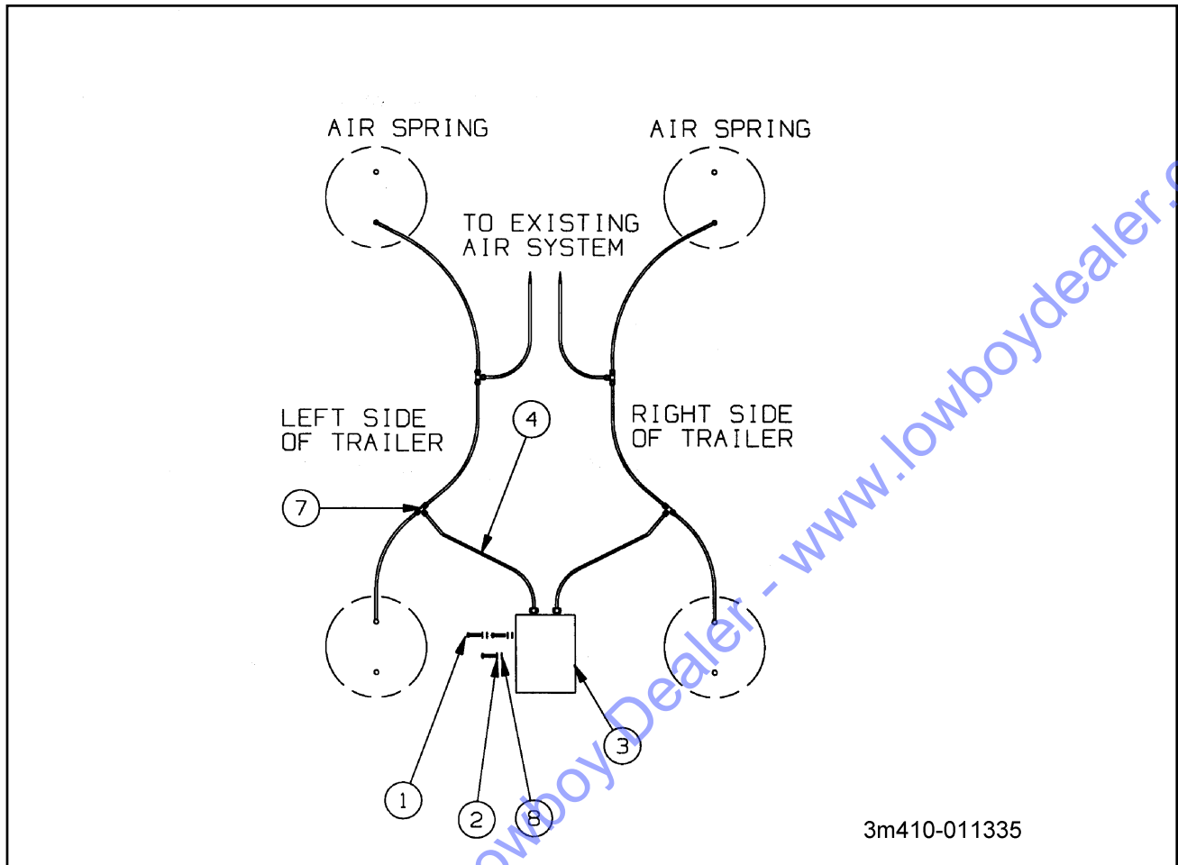
Figure 1-60 Scale-o-matic Installation (Optional)
