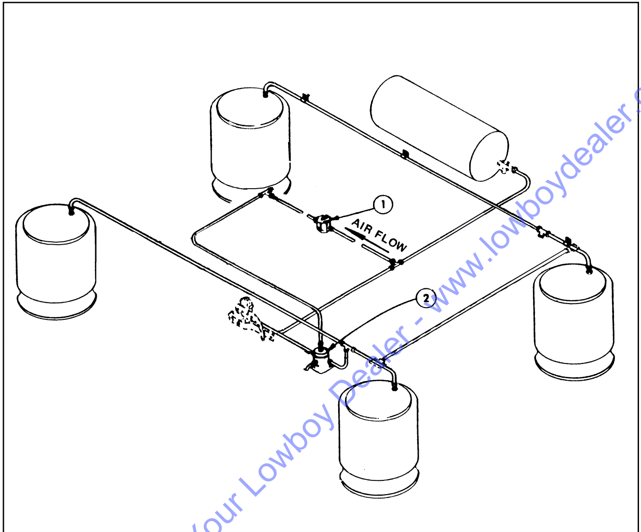
Figure 1-16 Air Control Kit
