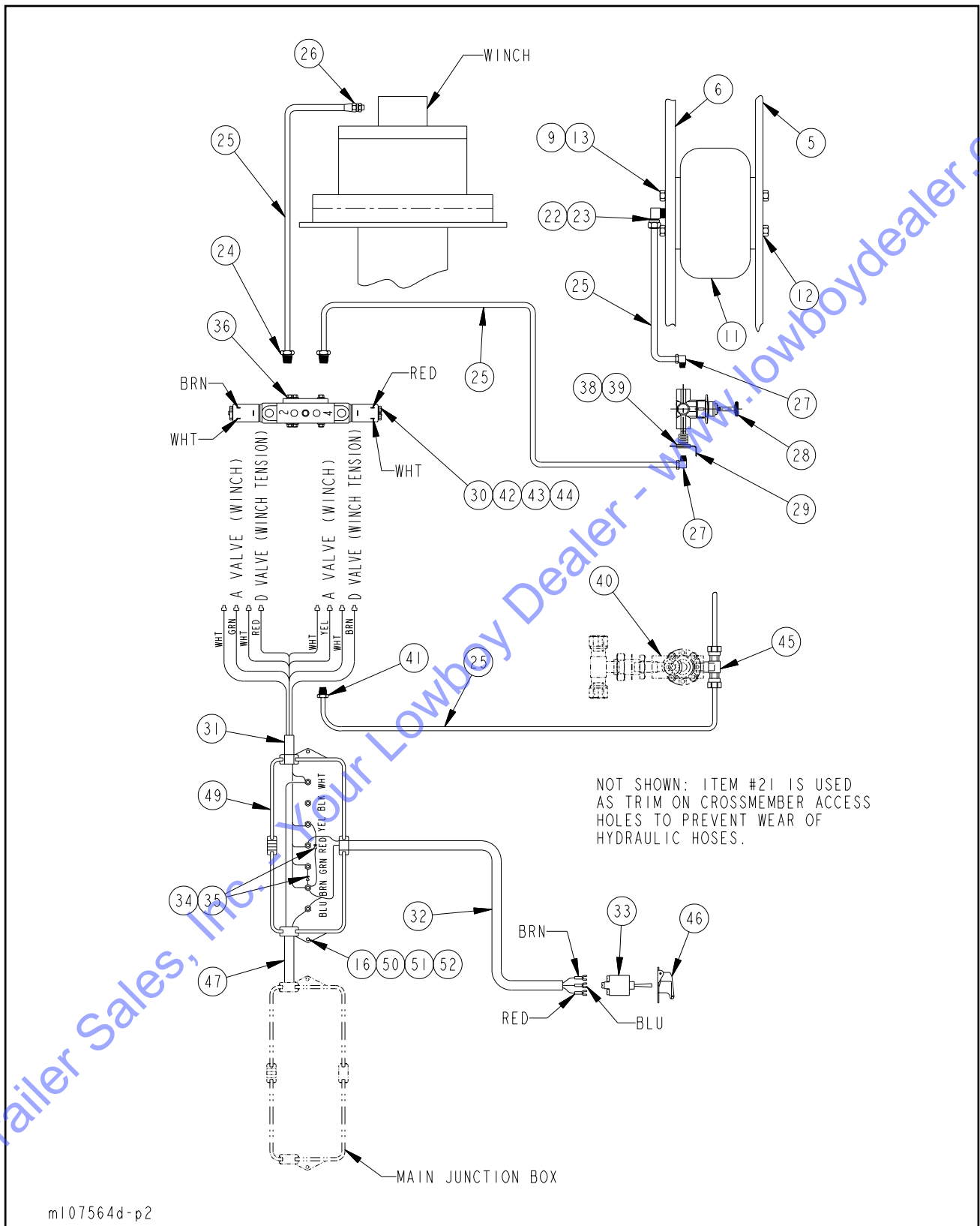
Figure 1-39 12K, 15K, & 20K Upper Deck Winch (DP) (2 of 2)
