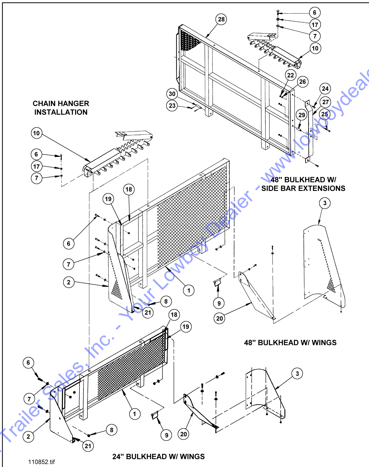
Figure 1-5 Bulkhead Assembly
