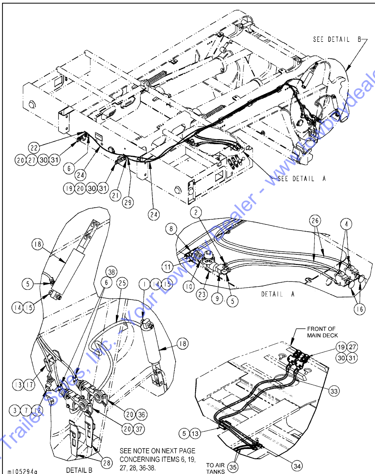
Figure 1-18 Air System
