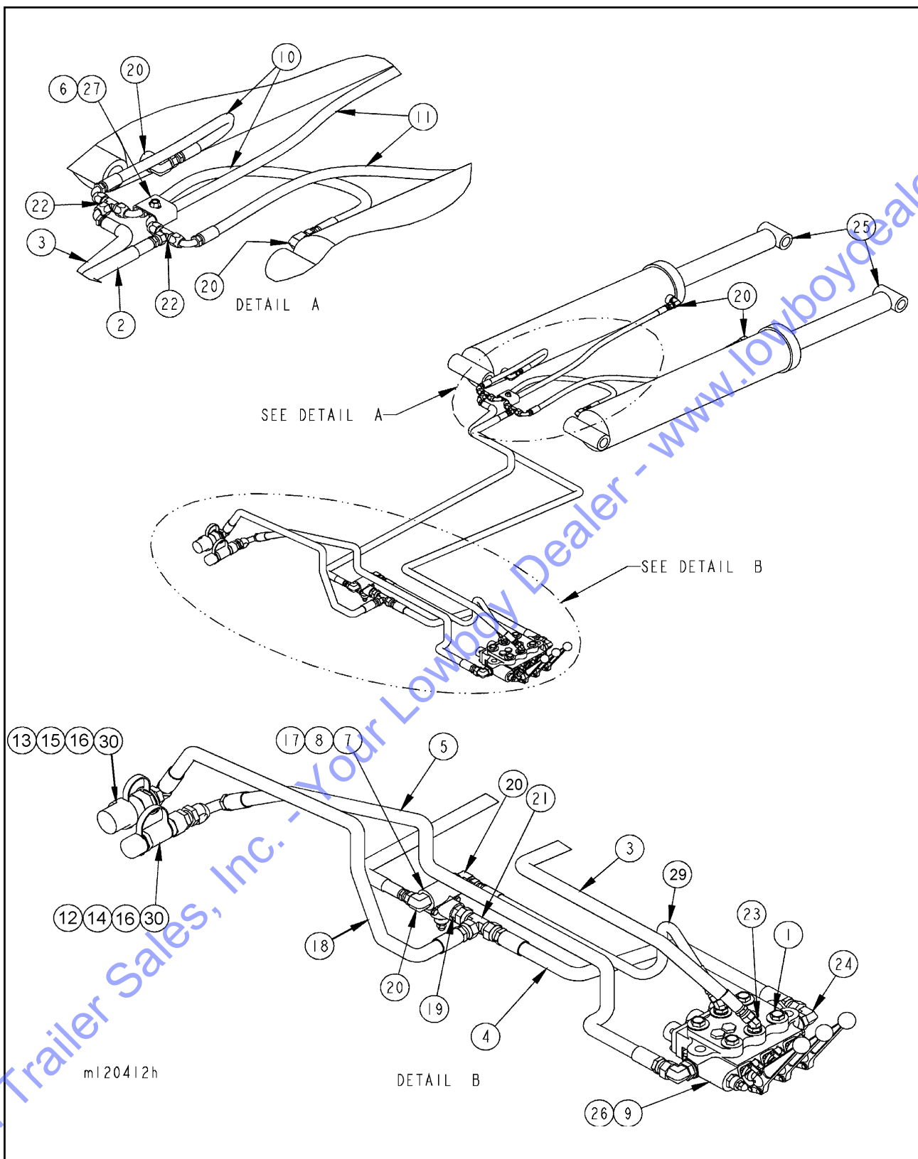
Figure 1-9 Hydraulic System (835)
