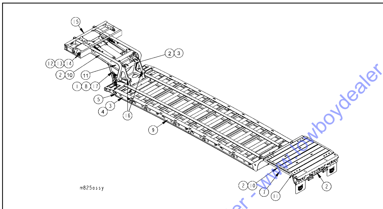
Figure 1-32 Decal Placement
