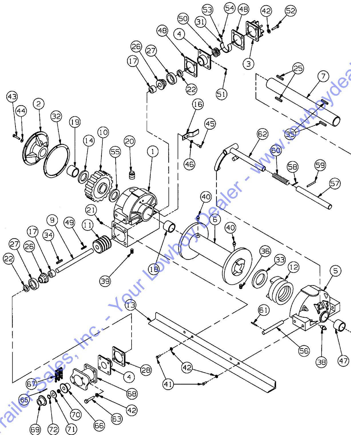
Figure 1-27 12,000# Winch Assembly
