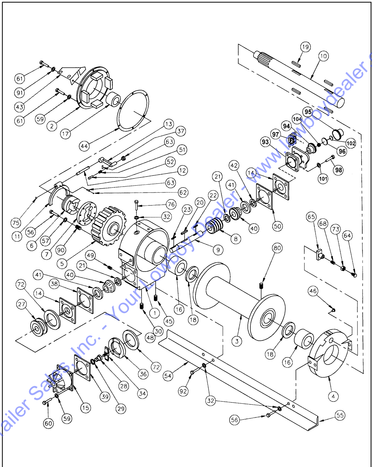
Figure 1-28 20,000# Winch Assembly
