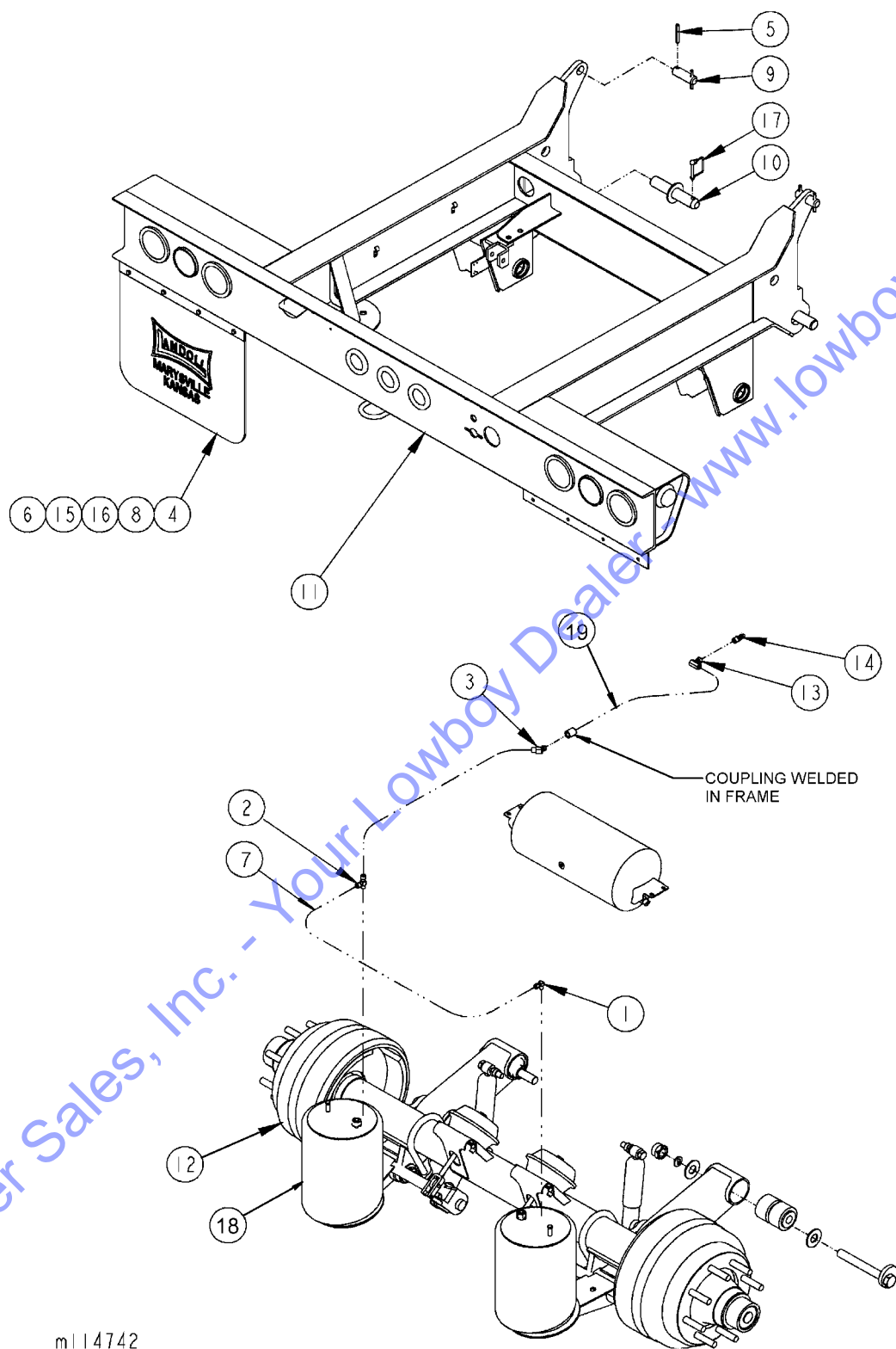
Figure 1-7 Flip Assembly - Air Ride Suspension
