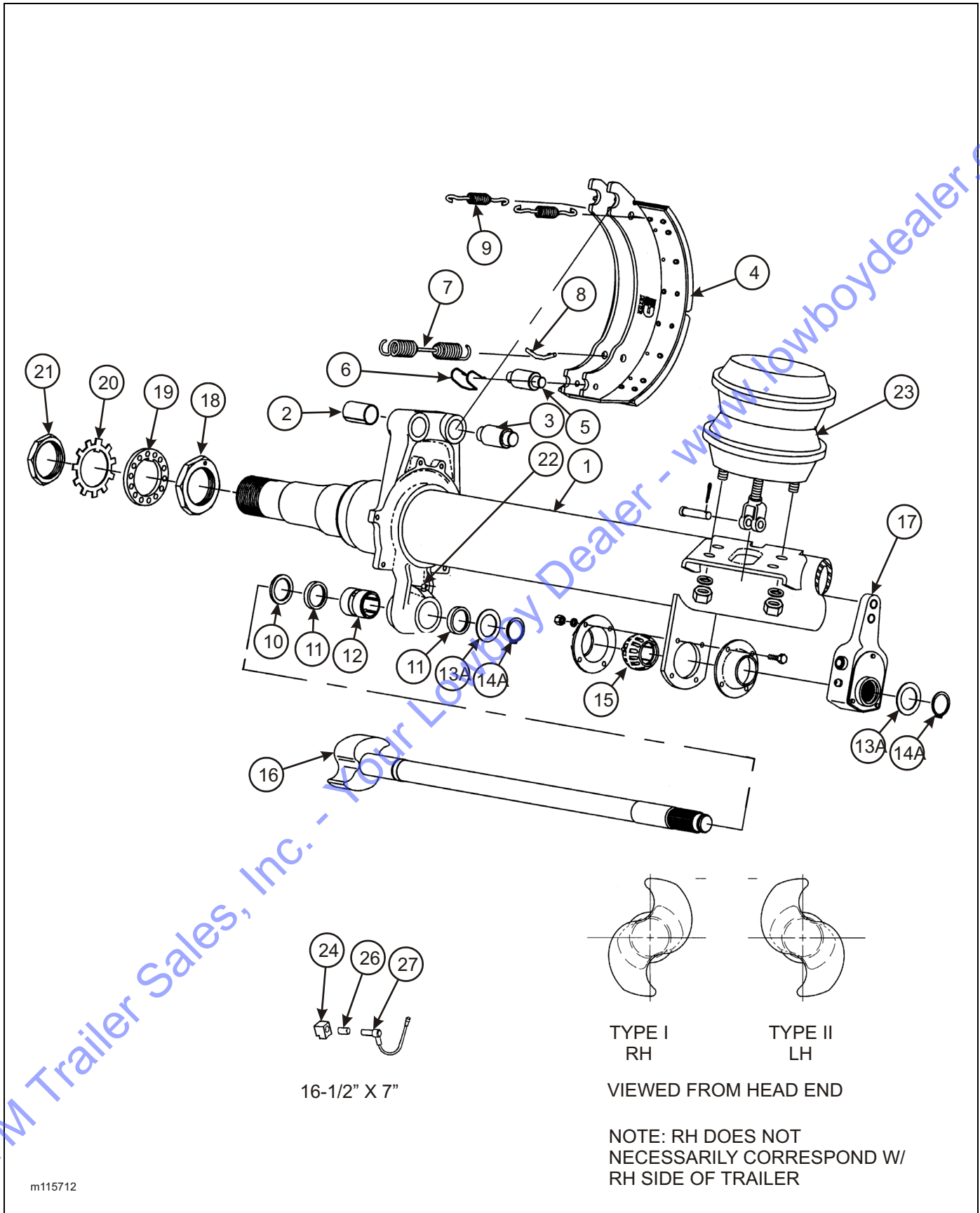
Figure 1-16 Axle and Brake Assembly
