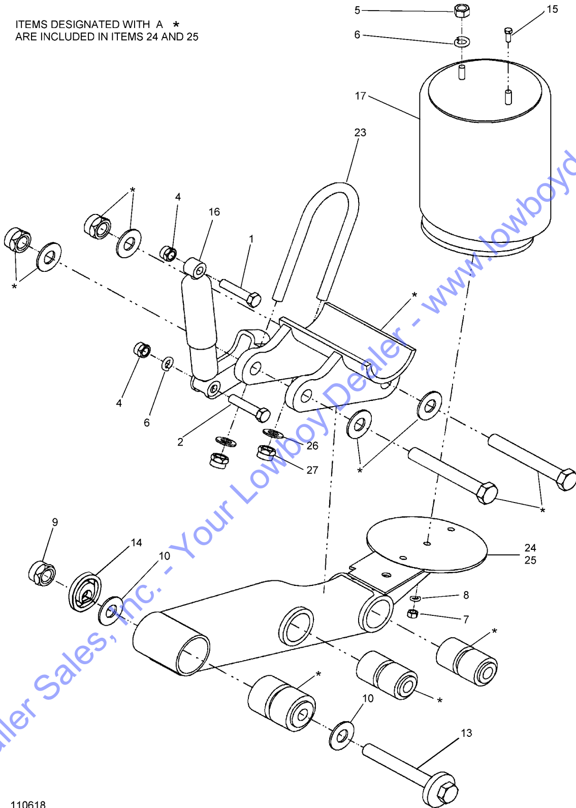
Figure 1-14 Suspension, Fastener RLU-250-9-4
