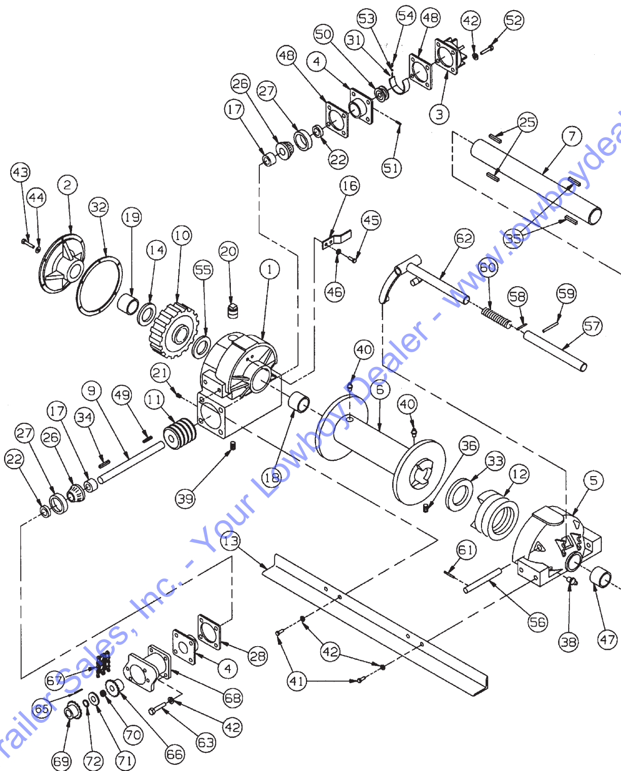
Figure 1-47 12,000# Winch Assembly
