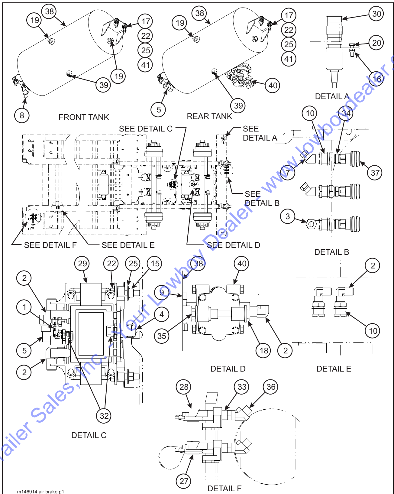
Figure 1-35 Air Brake System (835B)
