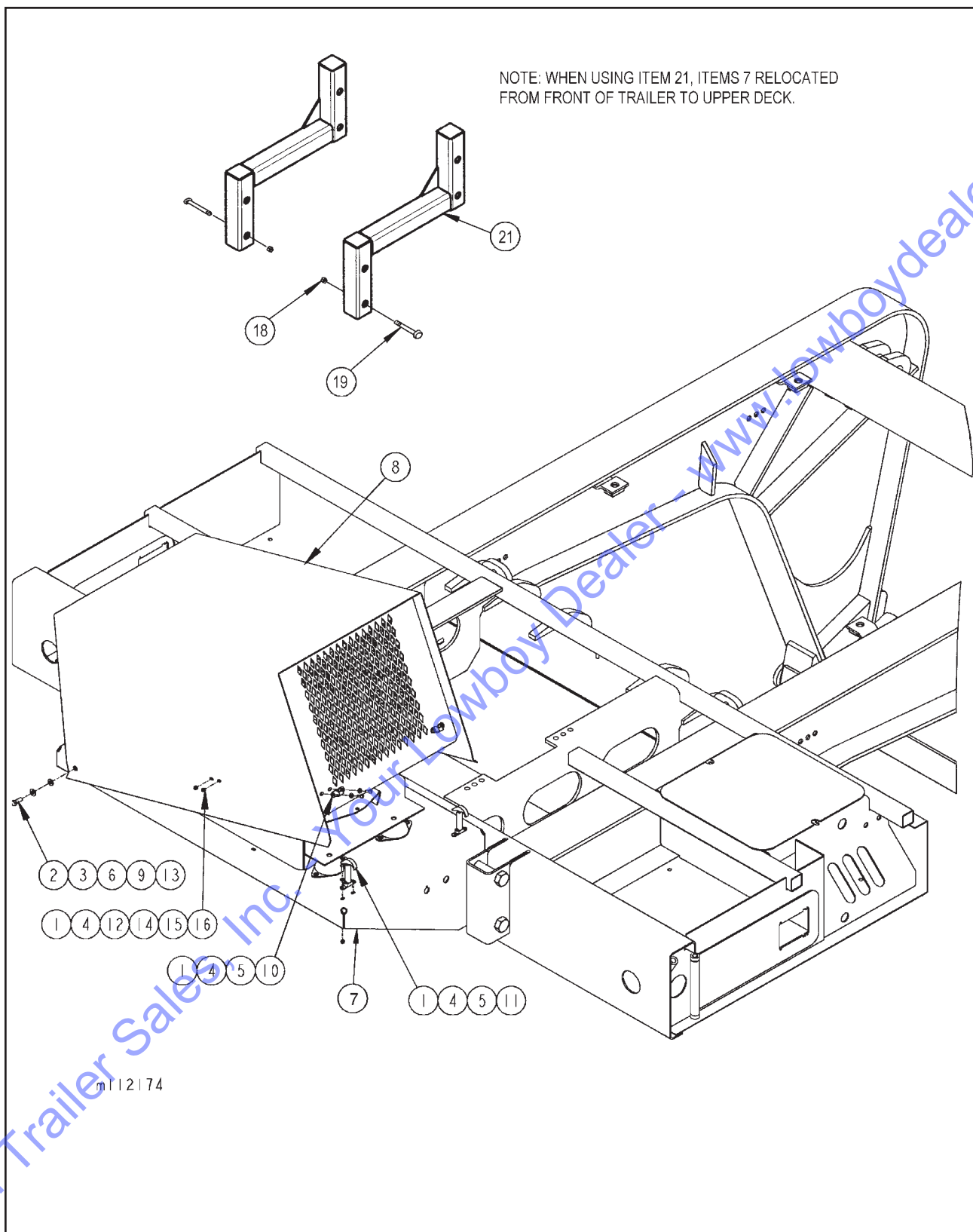
Figure 1-60 Front Mount Engine Cover Installation (Option)
