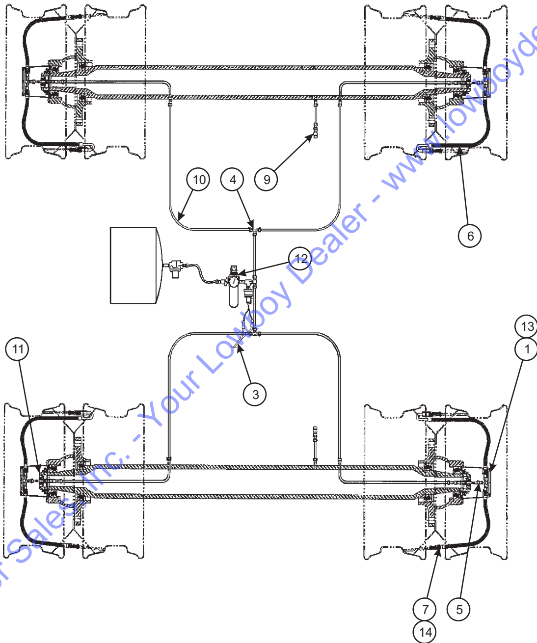
Figure 1-78 Tire Inflation System (Option)
