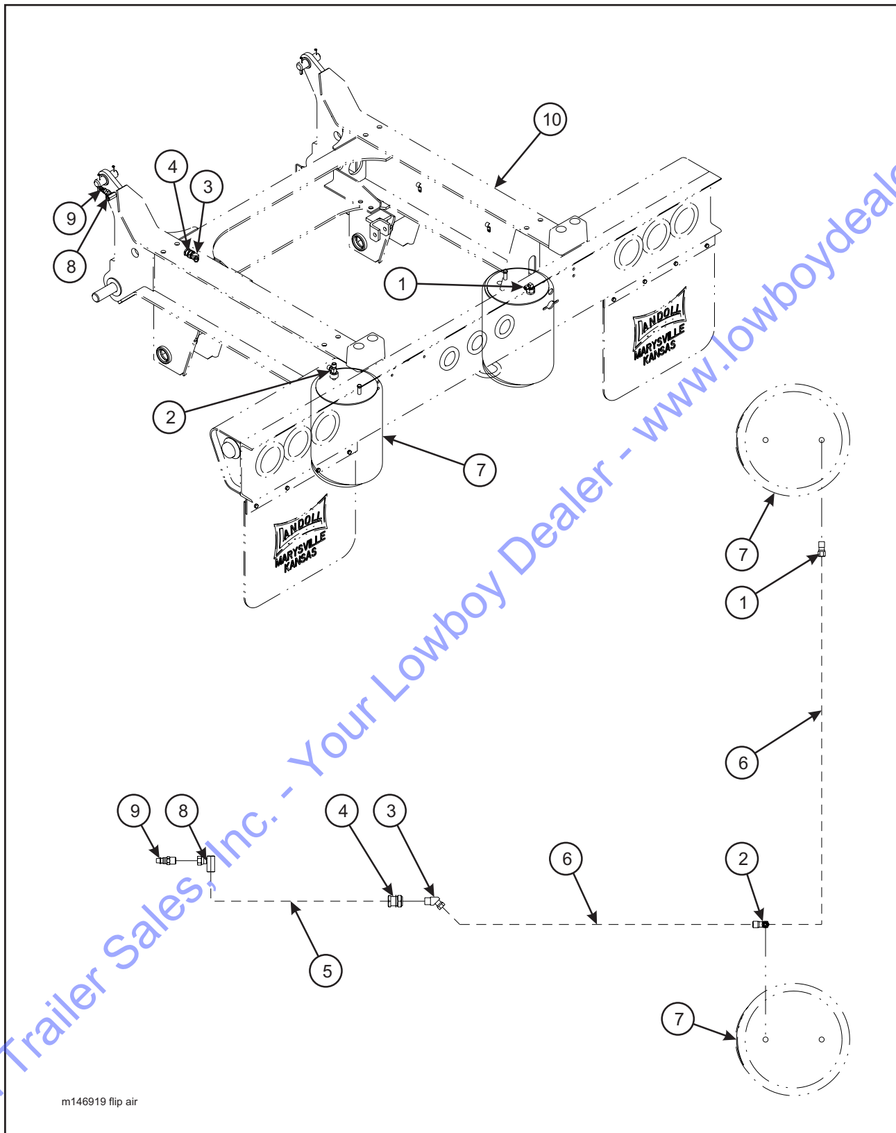
Figure 1-19 Flip Assembly - Air Ride Suspension
