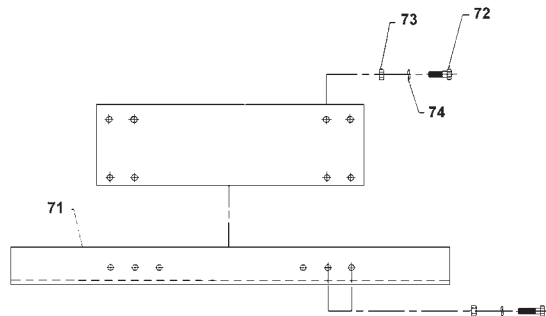
AIR/HYDRAULIC KICKOUT GEAR END COVER INSTALLATION
