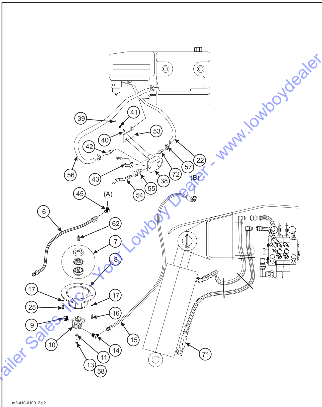
Figure 1-59 42-11 HP Honda Engine Drive Installation (Option) (2 of 2)
