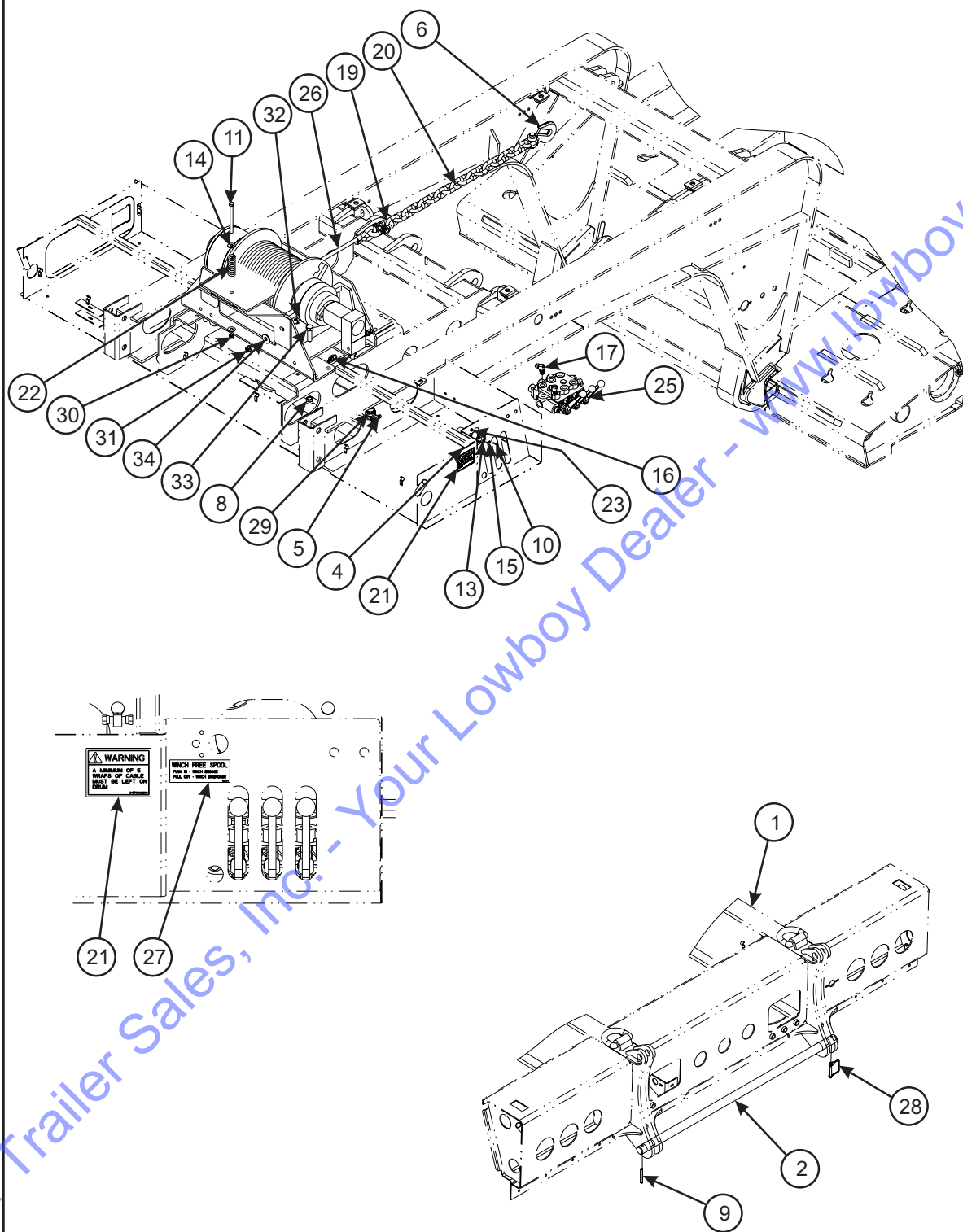
Figure 1-52 30K DP Winch Installation
