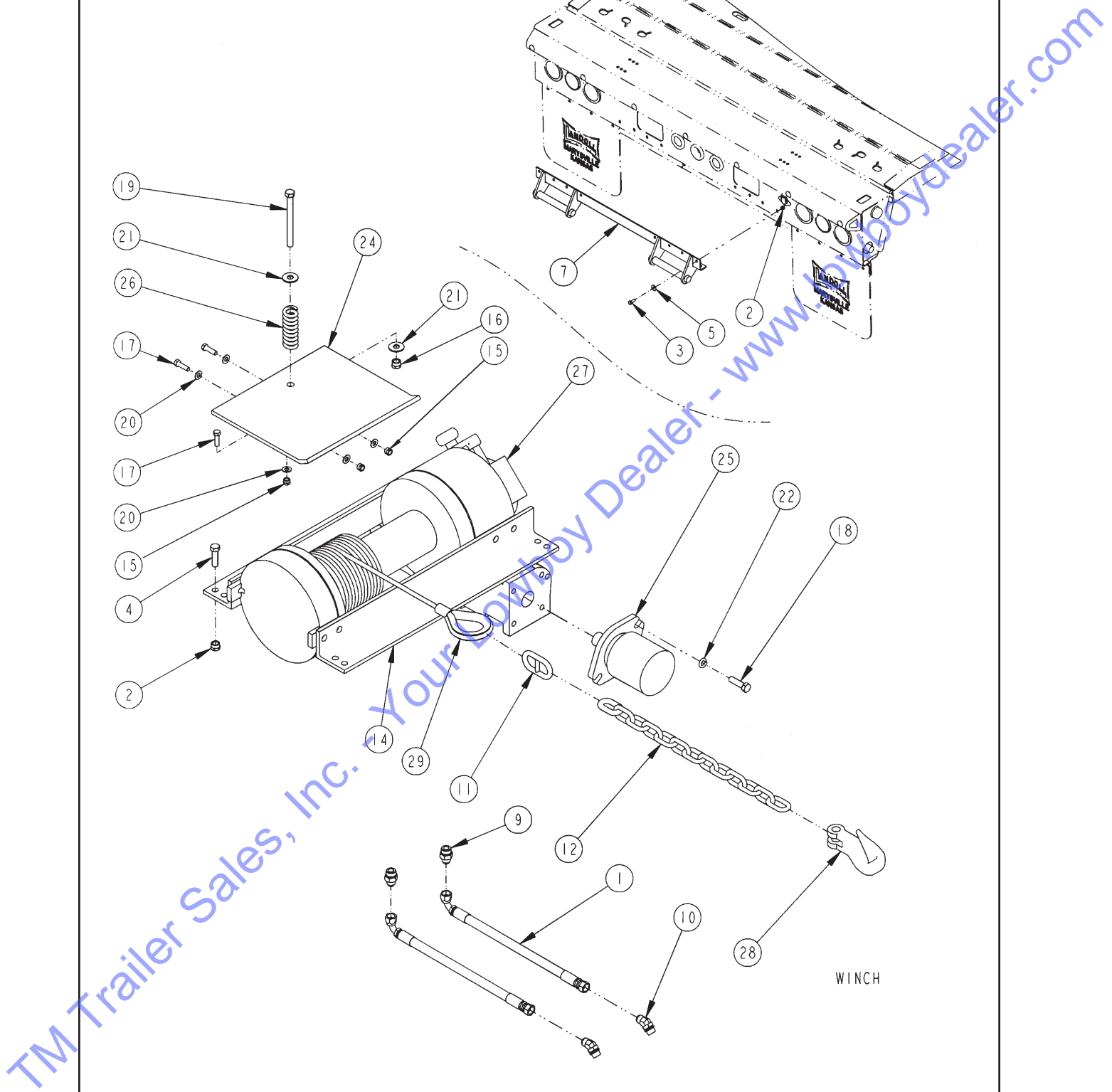
Figure 1-46 Winch Installation
