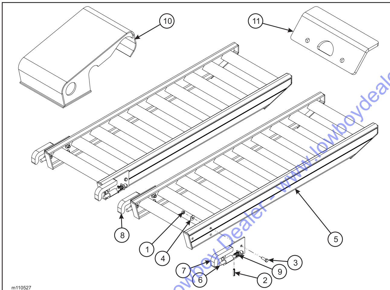
Figure 1-65 Aluminum Beavertail Ramp Assembly (Option)
