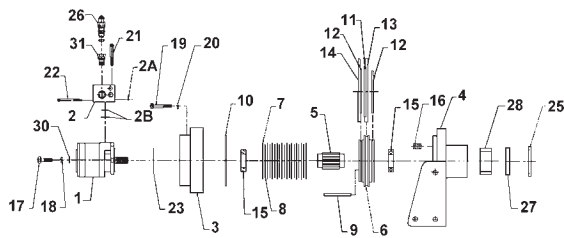
MOTOR END INSTALLATION
