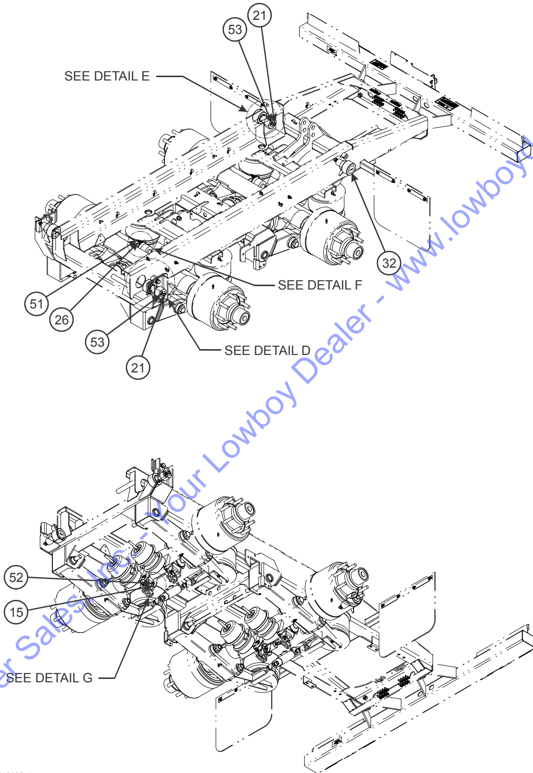
Figure 2-27: U/C Assembly, Air Ride Suspension (425 & 435) (2 of 4)
