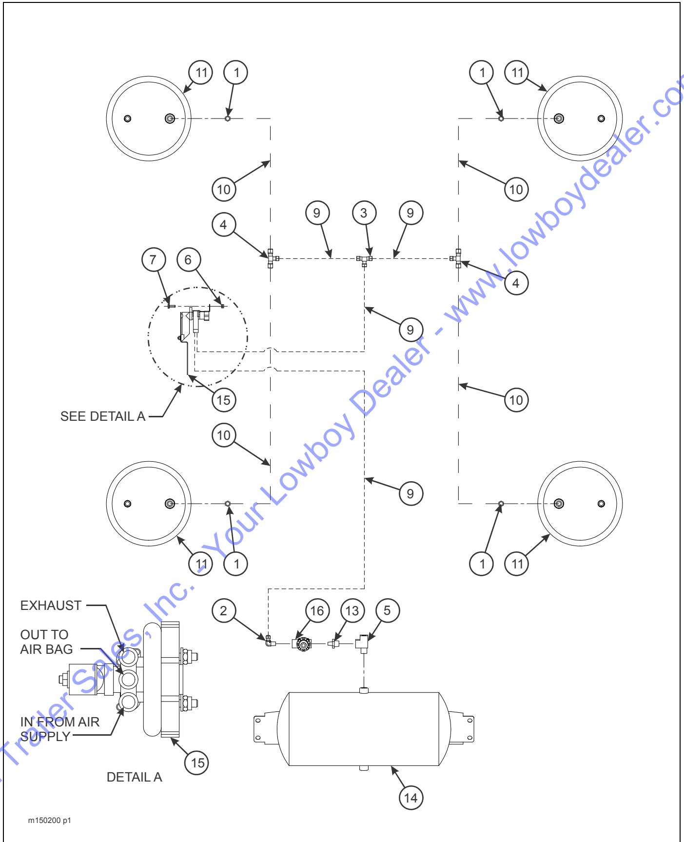
Figure 2-30: Air Ride Suspension, Air System (Tandem)
