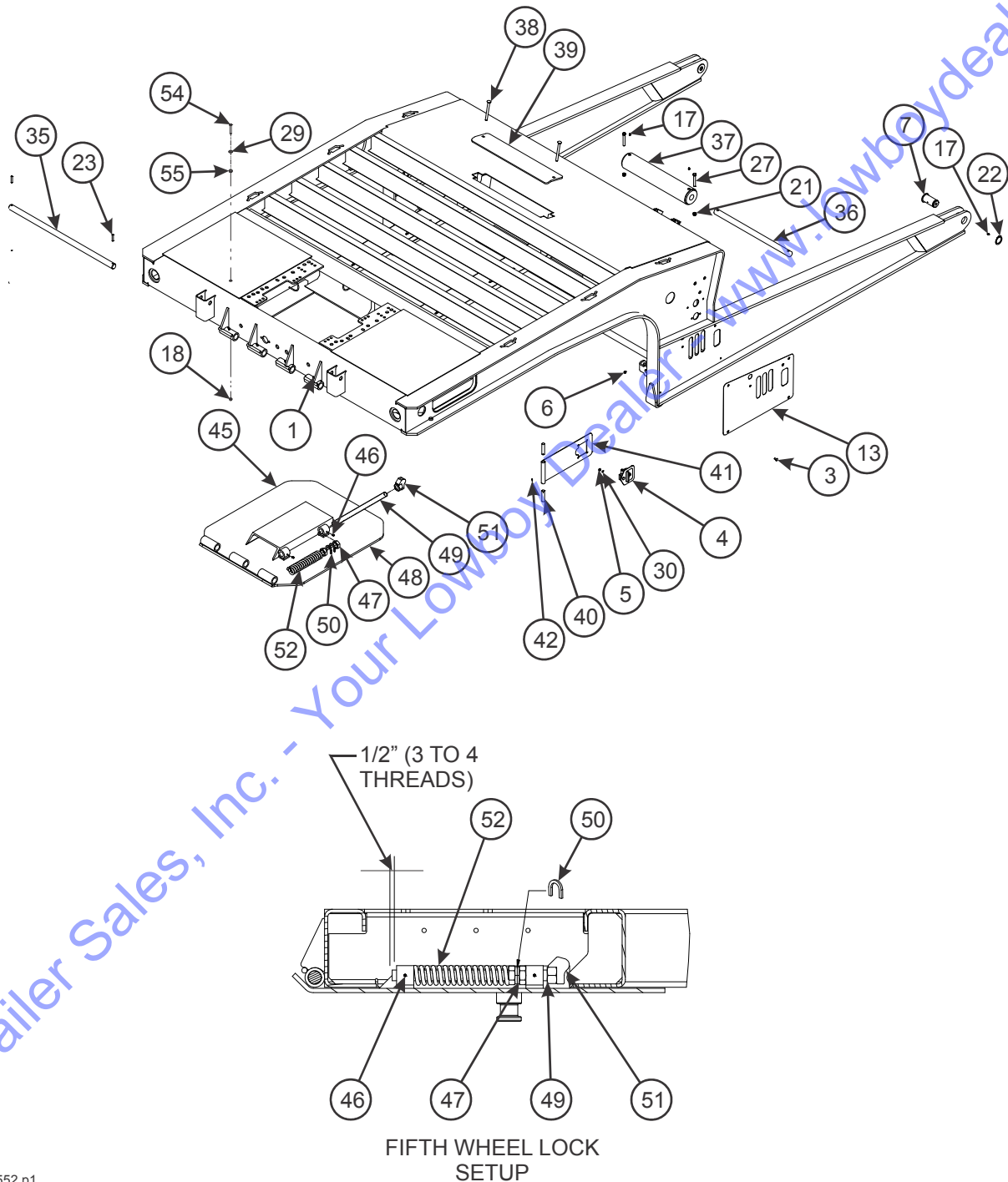
Figure 2-2: Upper Deck Assembly (1 of 2)
