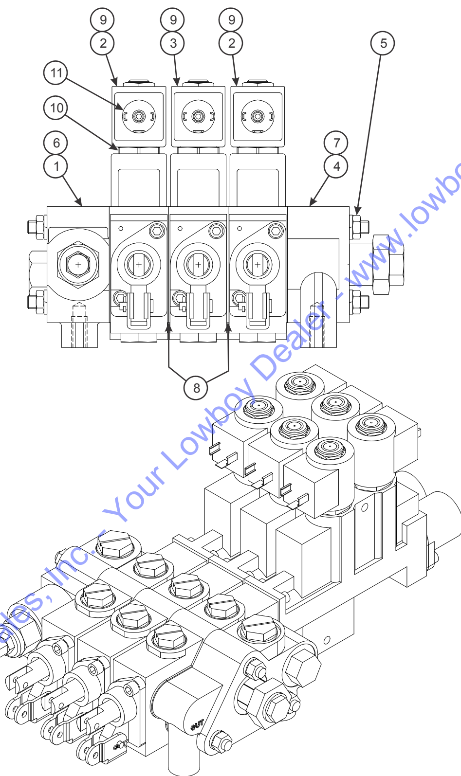
Figure 2-10: Three Spool Valve
