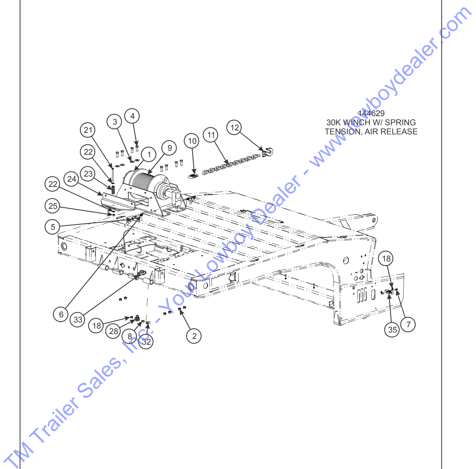
Figure 2-50: 30,000 Lb. Upper Deck Winch Installation (2 of 3)
