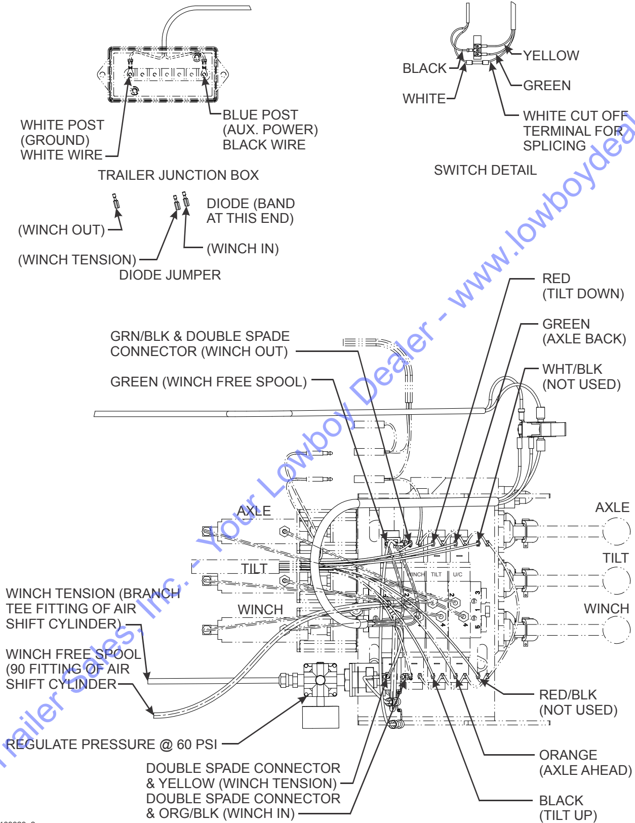
Figure 2-43: Winch Installation (2 of 2)
