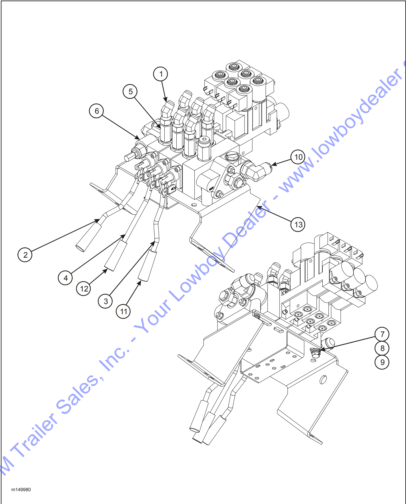
Figure 2-9: Valve Assembly - 3 Spool, Remote
