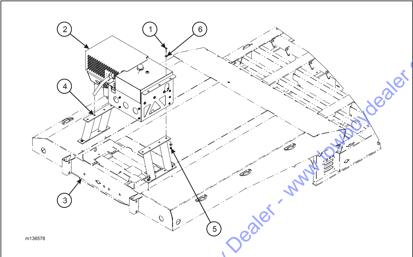
Figure 2-54: Engine Package Stand Installation (Option)
