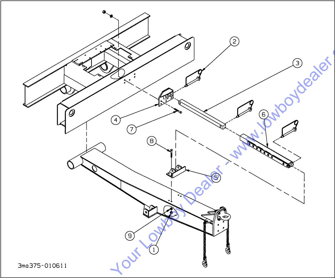
Figure 2-56: Hitch Lock Installation (Option)
