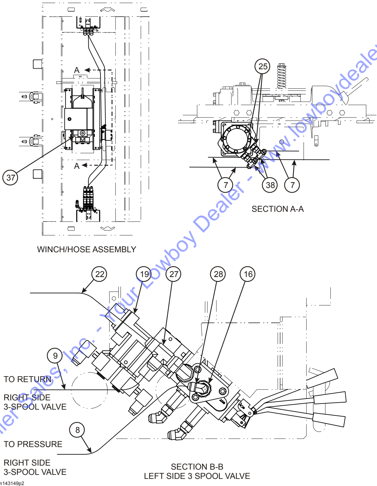
Figure 2-4: Hydraulic Assembly (2 of 3)
