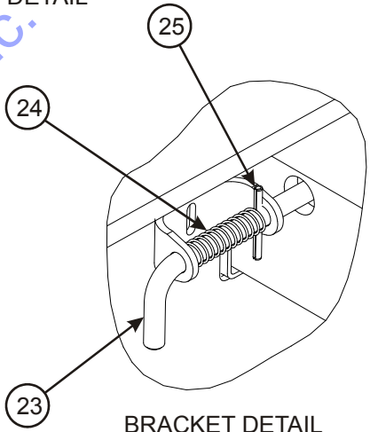
BRACKET DETAIL
