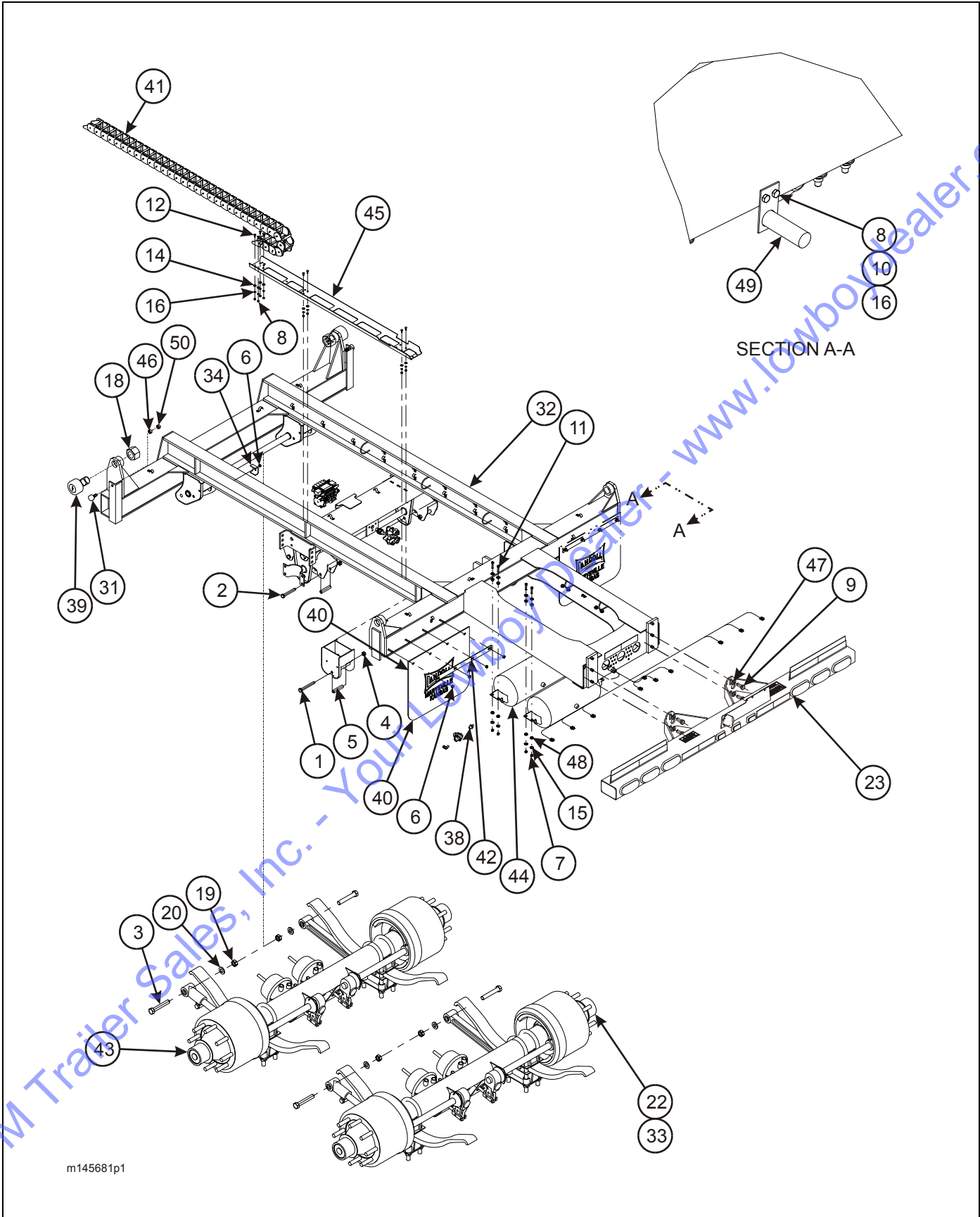
Figure 2-13: Undercarriage Assembly - Spring Ride (1 of 2)
