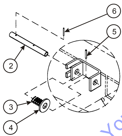
CATCH ASSEMBLY DETAIL
