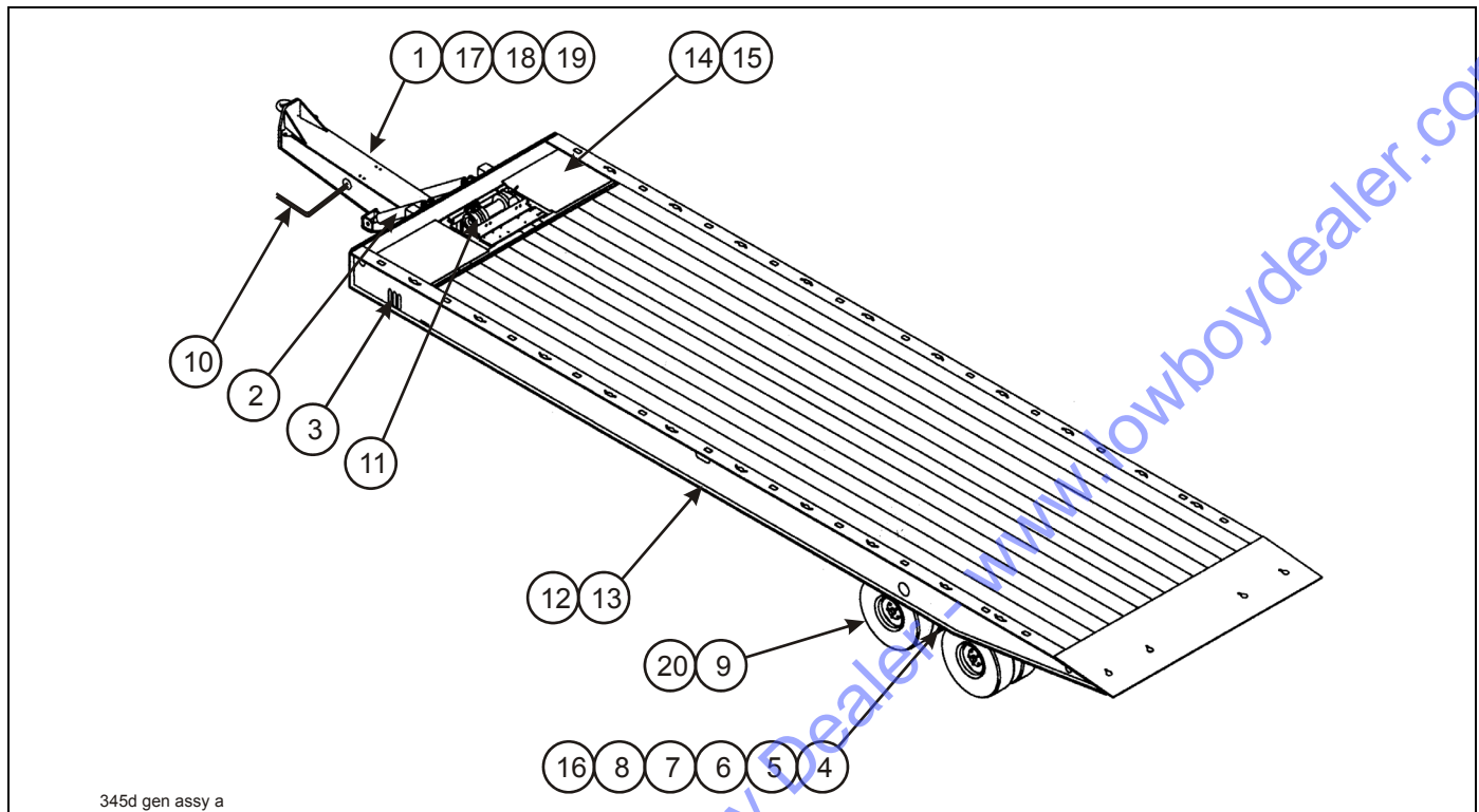
Figure 2-1: General Assembly
