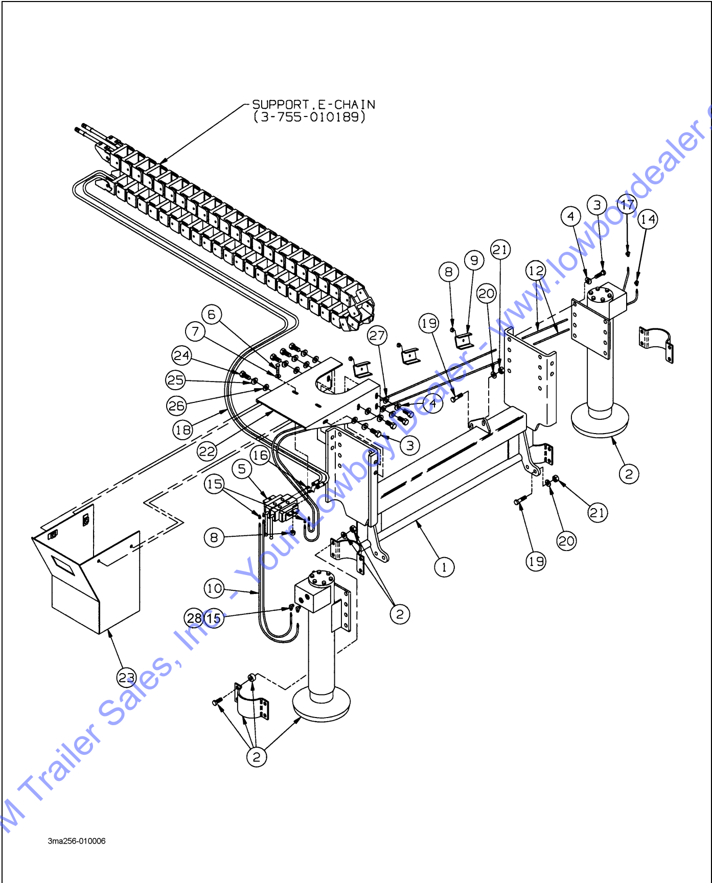
Figure 2-42: Dock Leveler Assembly
