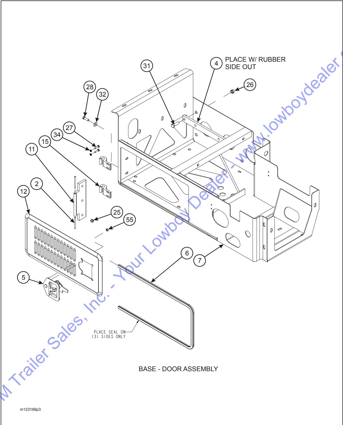
Figure 2-36: Engine Drive, 20 HP (3 of 4)
