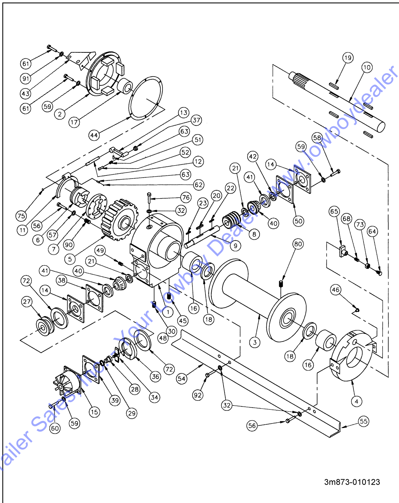
Figure 1-27 20,000# Winch Items
