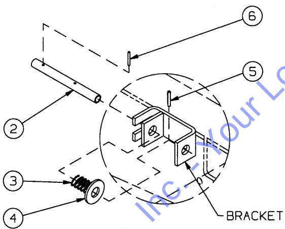
CATCH ASSEMBLY DETAIL
