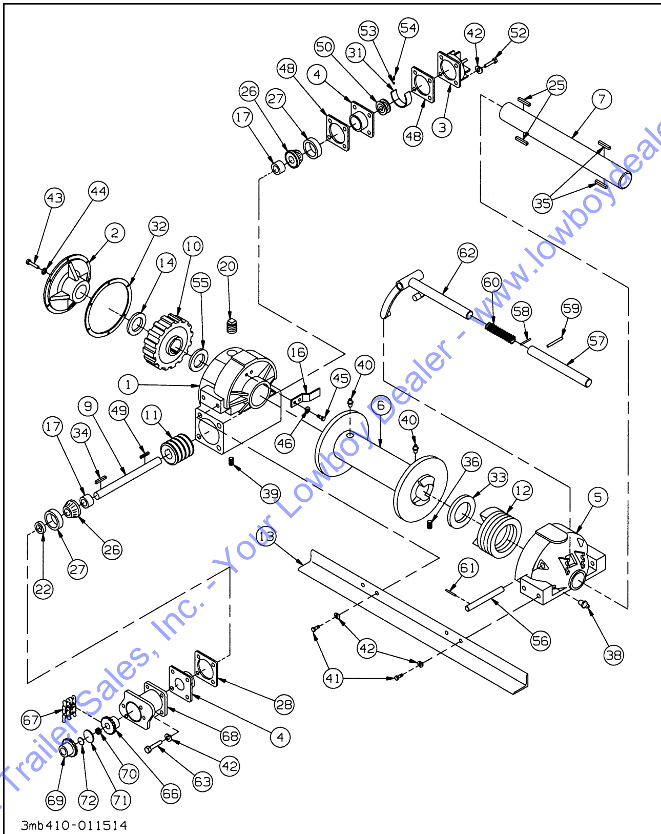
Figure 1-26 12,000 # Winch Items
