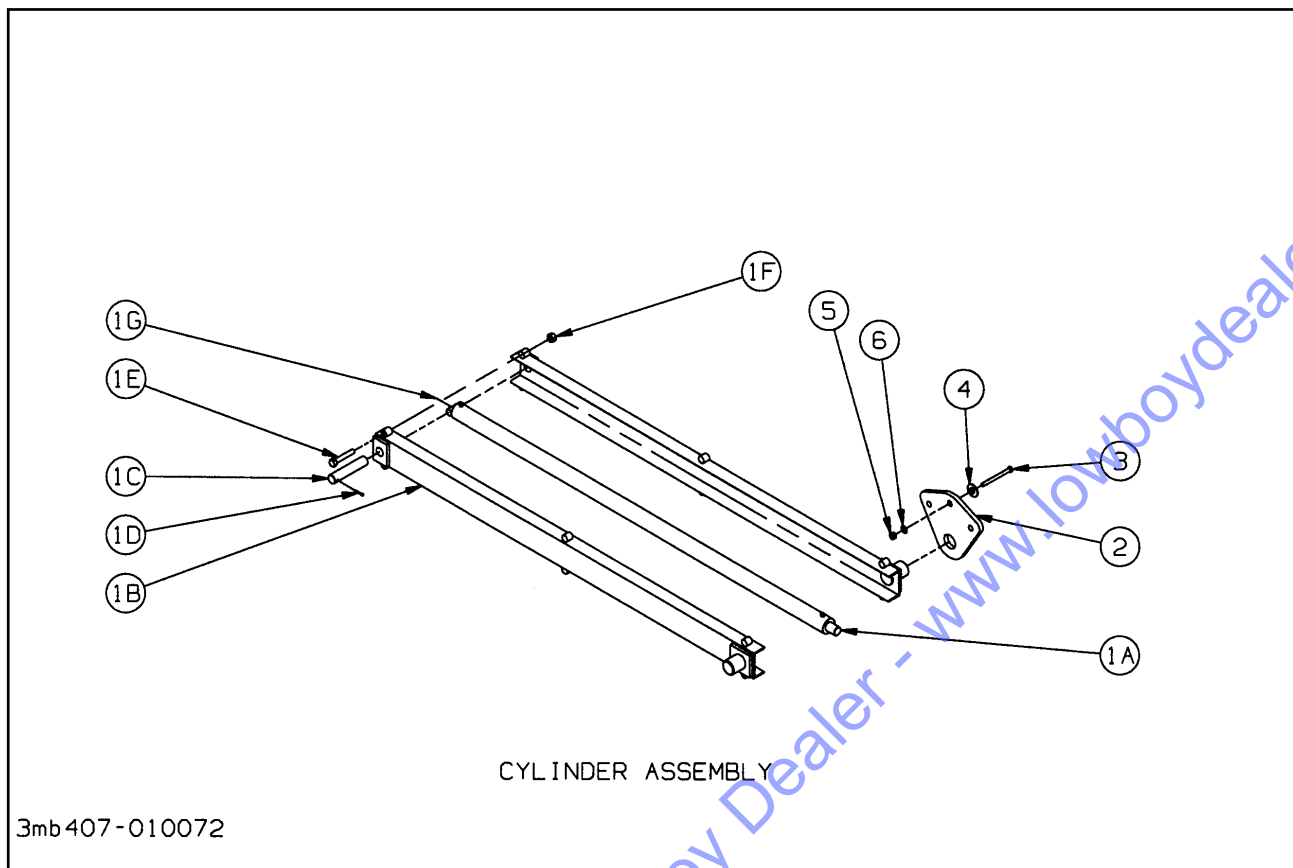
Figure 1-5 Hydraulic Assembly
