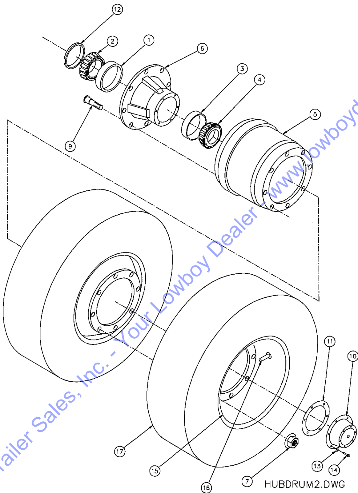
Figure 1-22 Outboard Hub and Drum Assembly
