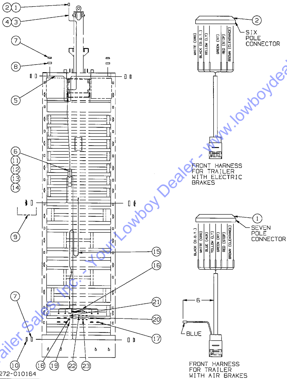
Figure 1-9 Electrical Assembly
