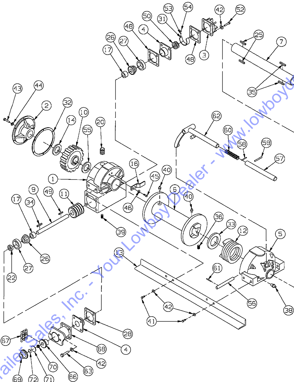
Figure 1-26 12,000 # Winch Items
