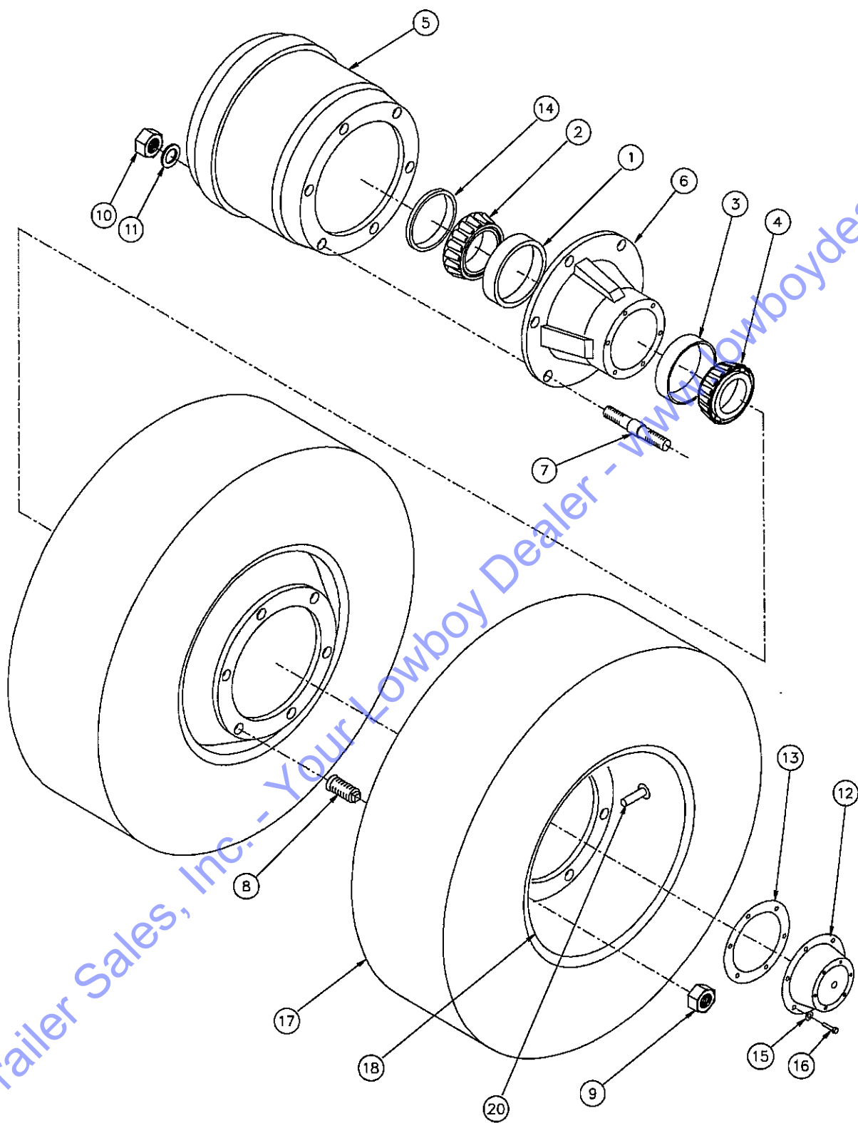
Figure 1-21 Inboard Hub and Drum Assembly
