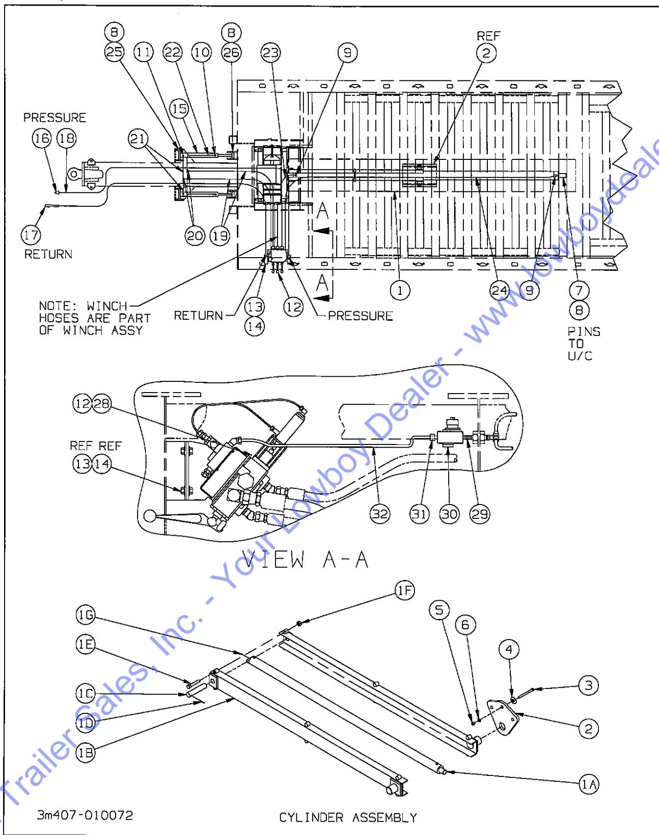
Figure 1-6 Hydraulic Assembly
