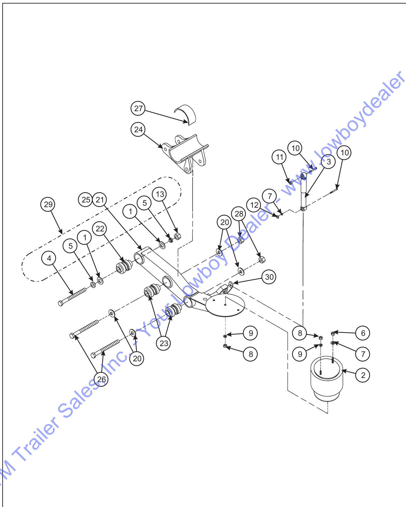
Figure 1-20: Suspension Hanger RLU-228
