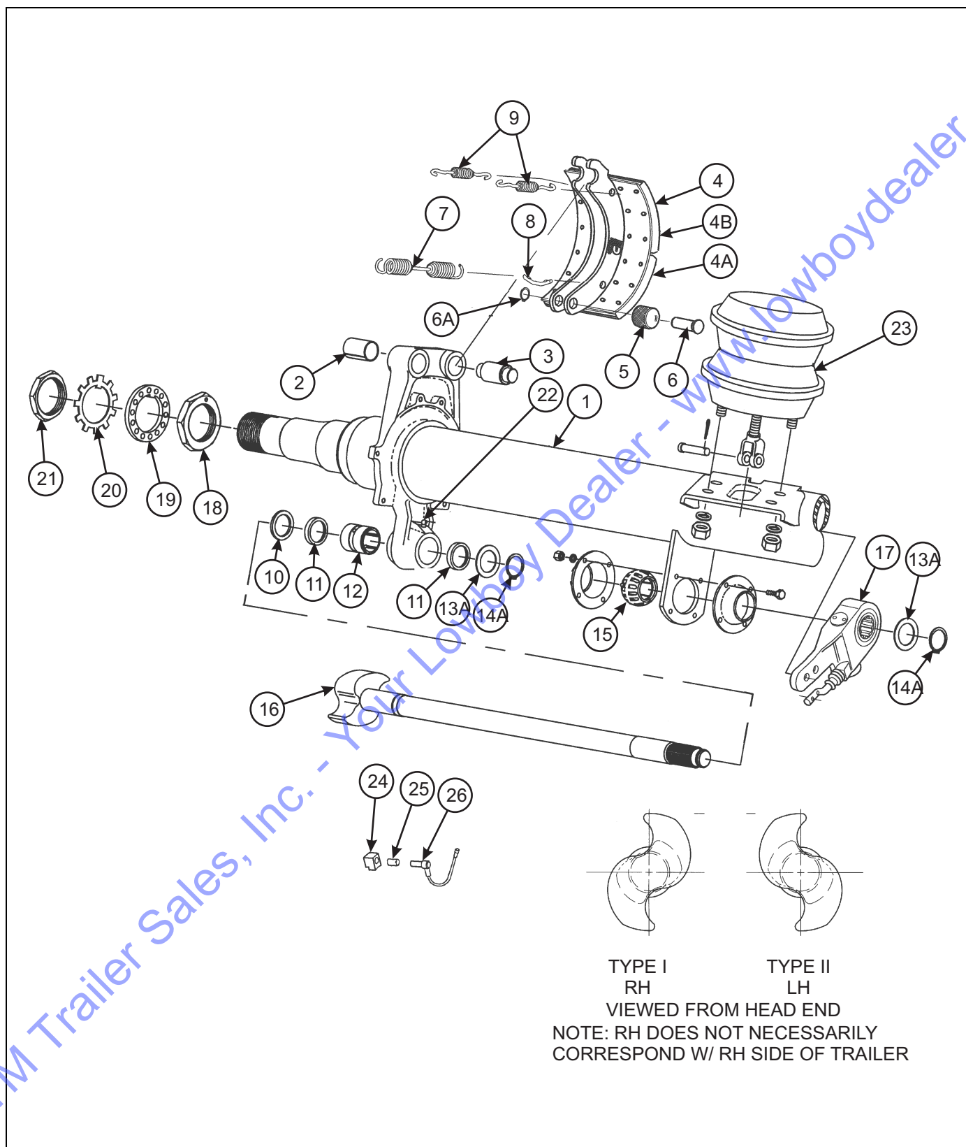
Figure 1-23: Axle and Brake Assembly - Dexter (12-1/4" X 7-1/2")
