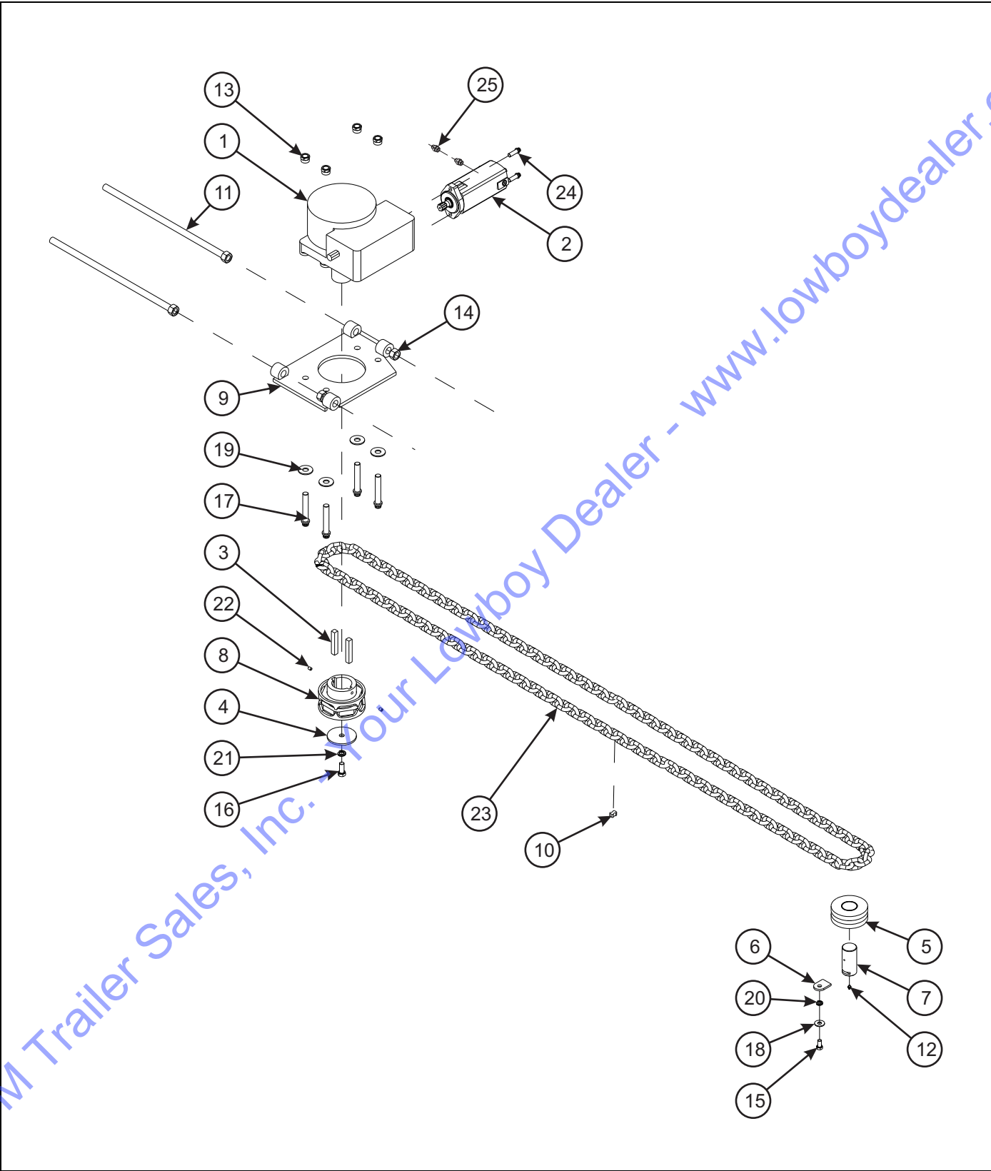
Figure 1-30: Gearbox Assembly
