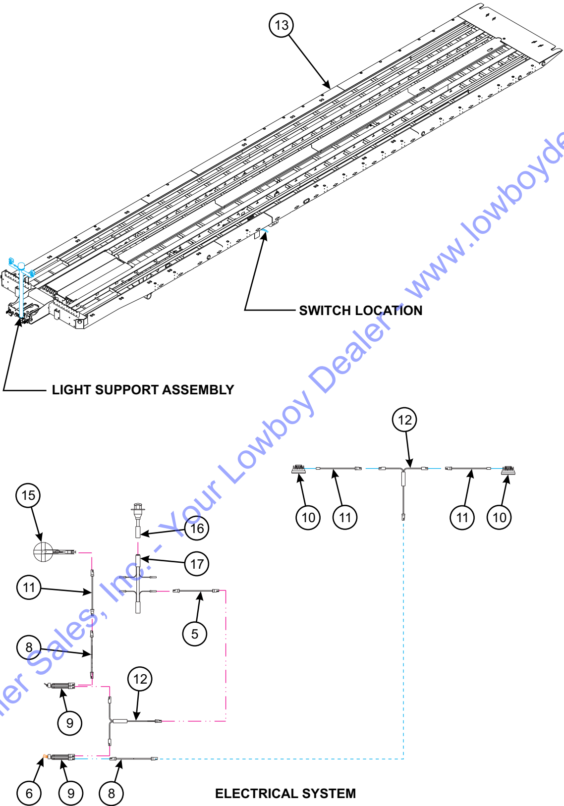
Figure 1-65: Light Strobe & Work Installation (1 of 2)
