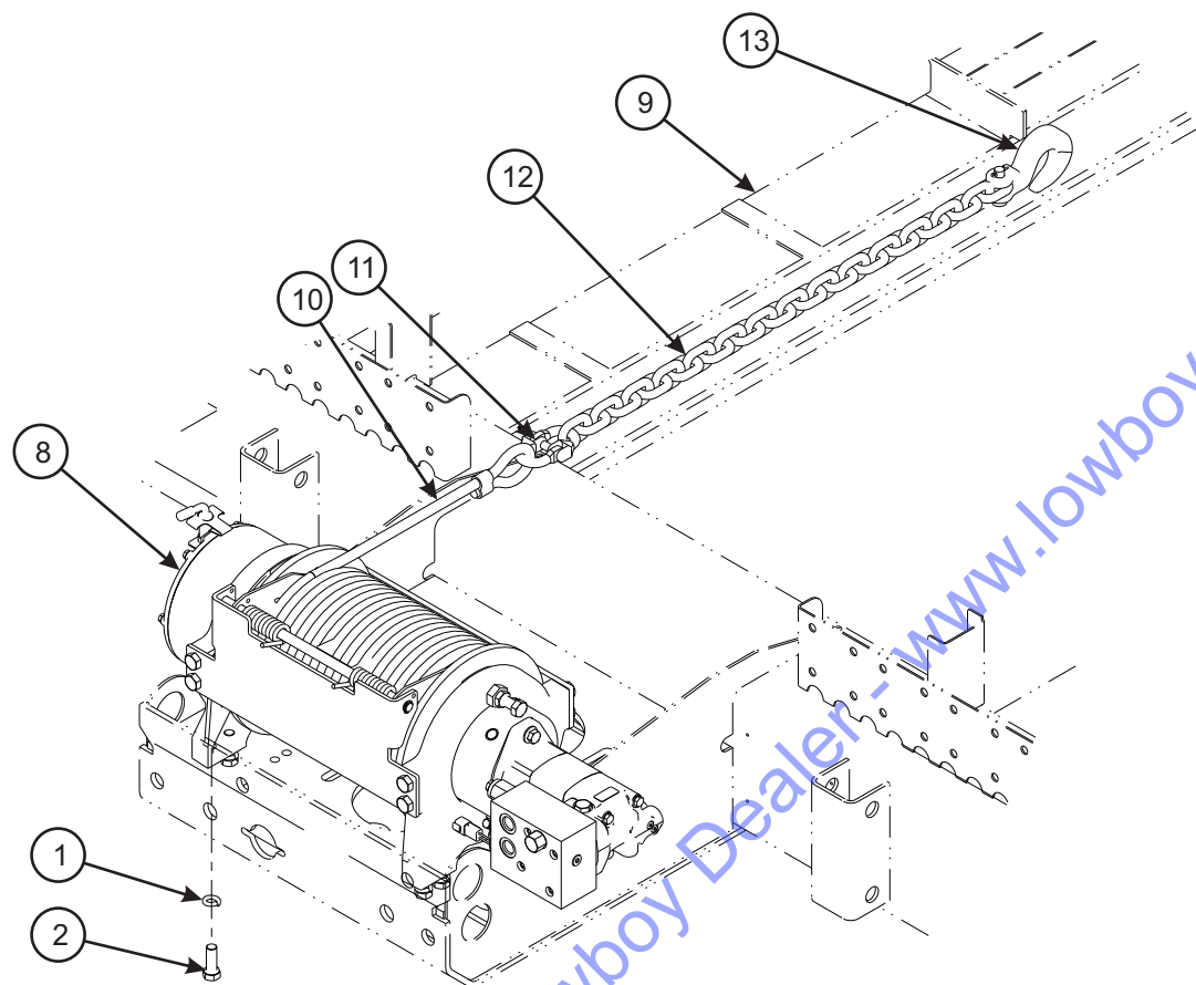
WINCH ASSEMBLY
