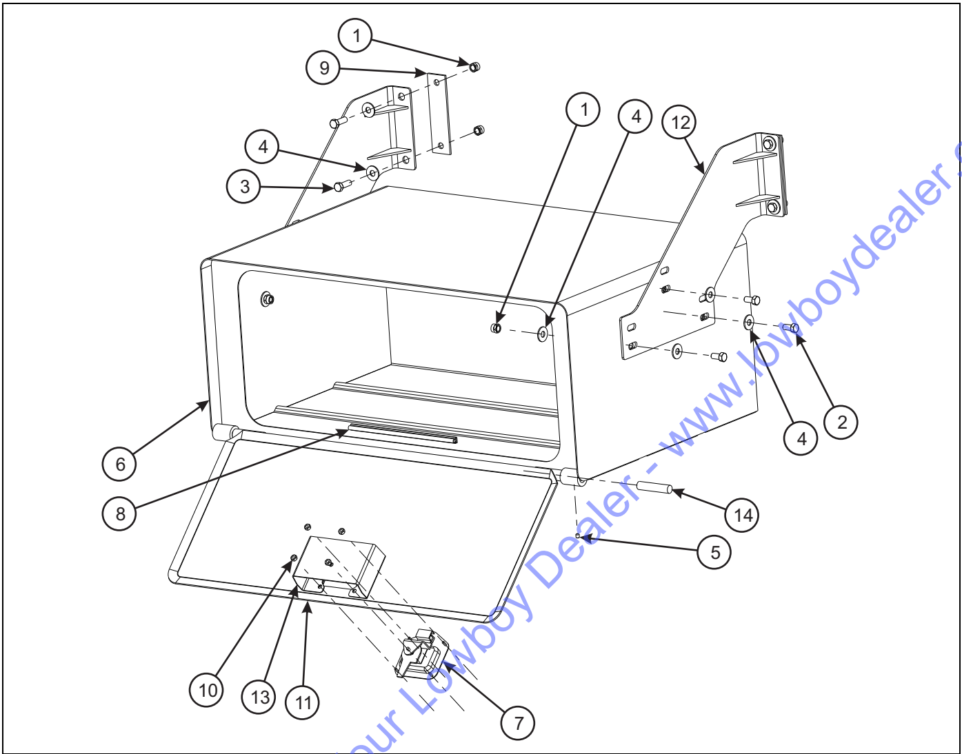
Figure 1-72: Tool Box Installation
