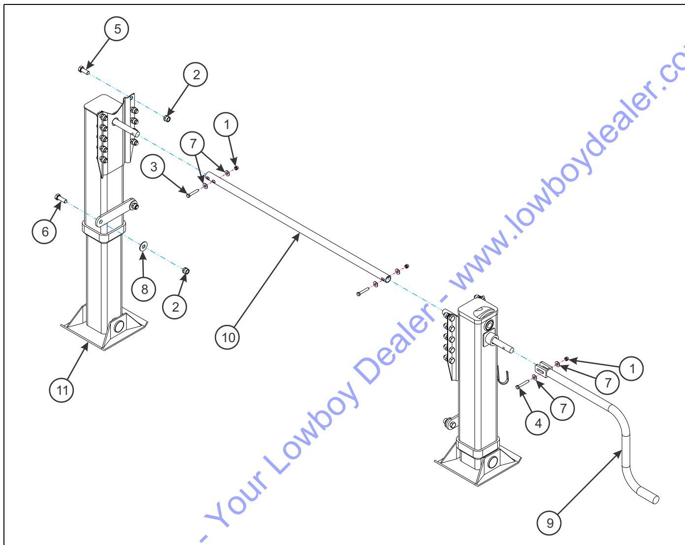
Figure 1-49: Landing Gear Installation - Jost 343
