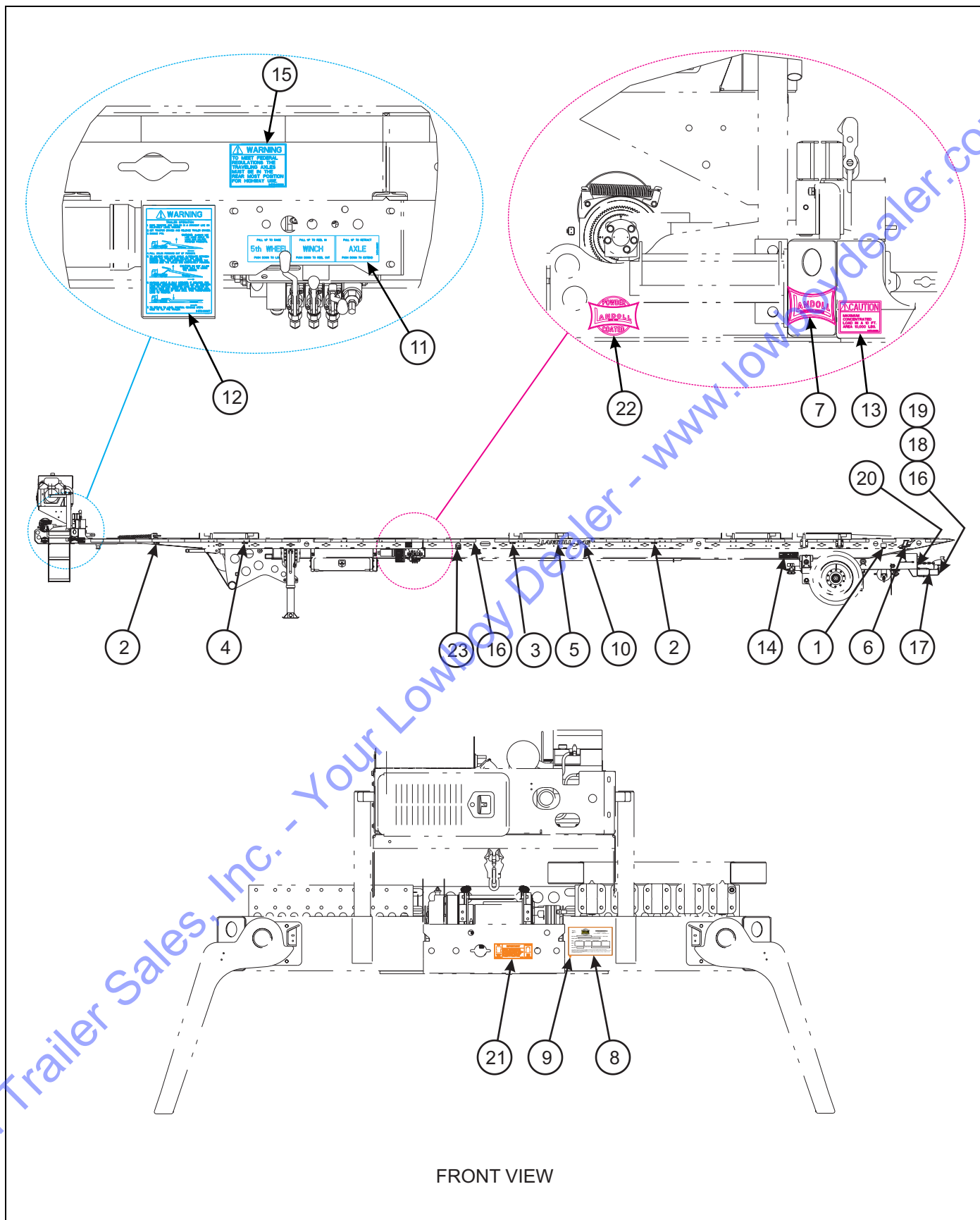
Figure 1-54: Decal Installation (2 of 2)
