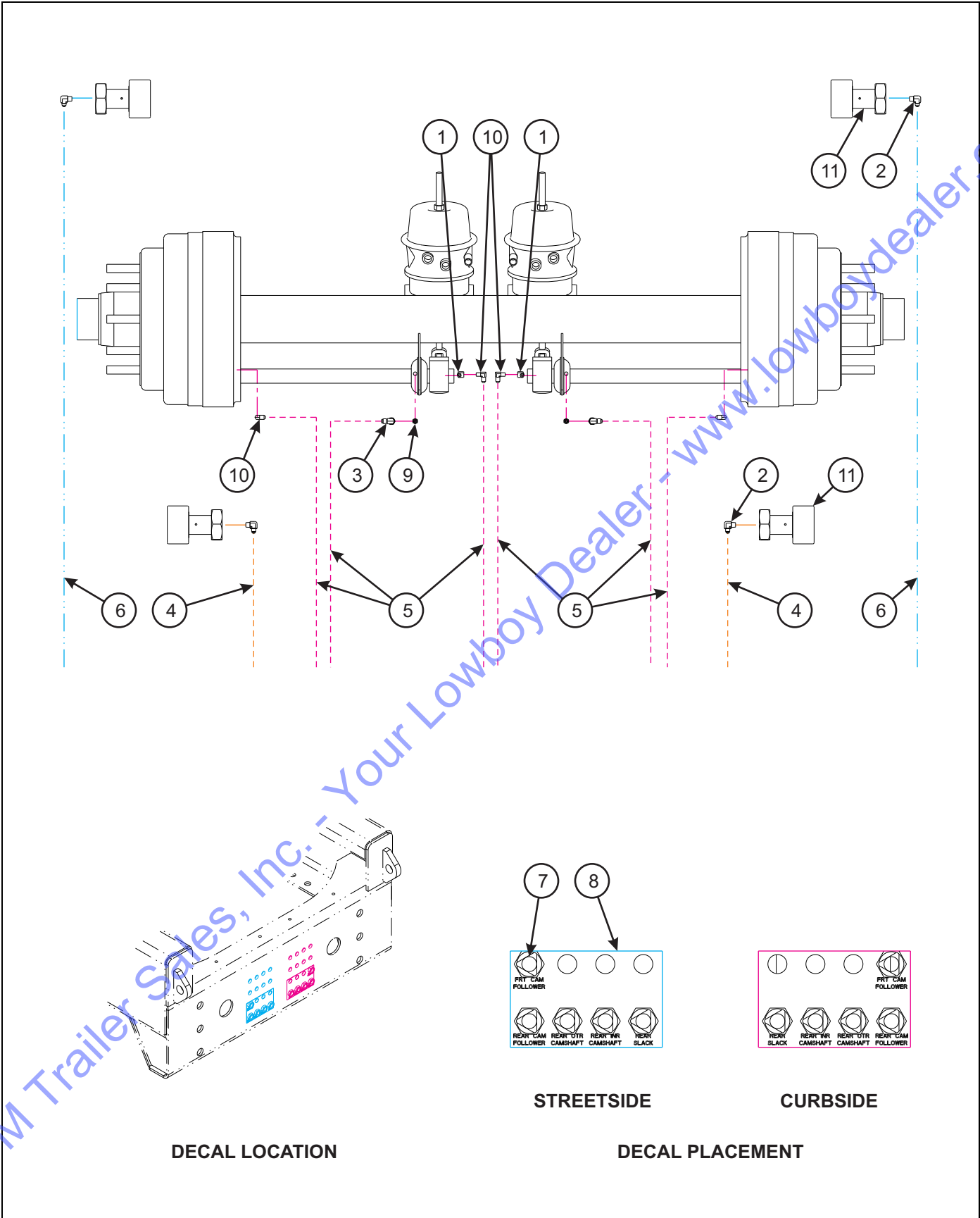
Figure 1-17: Grease System
