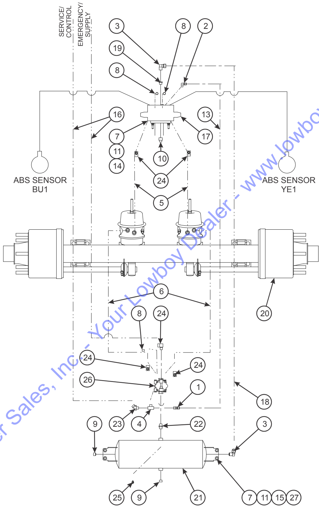
Figure 2-15: Air Brake System, Single Axle
