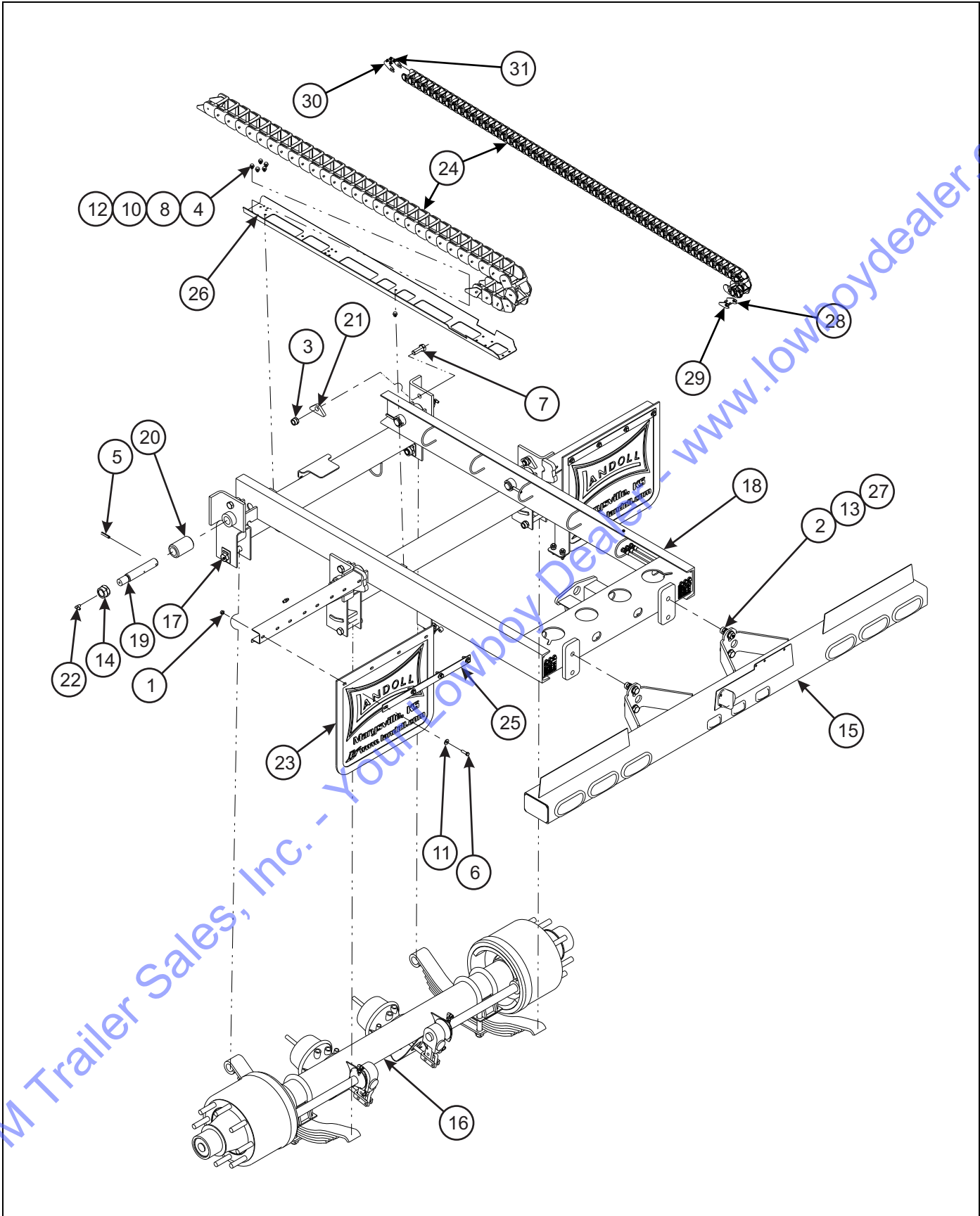
Figure 2-17: Undercarriage Assembly - Spring Ride Single Axle
