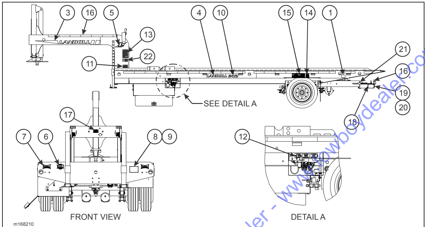
Figure 2-3: Decal Placement
