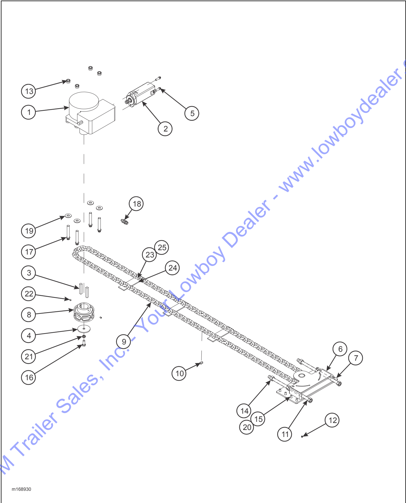
Figure 2-23: Gearbox Assembly (Chain Drive Model)
