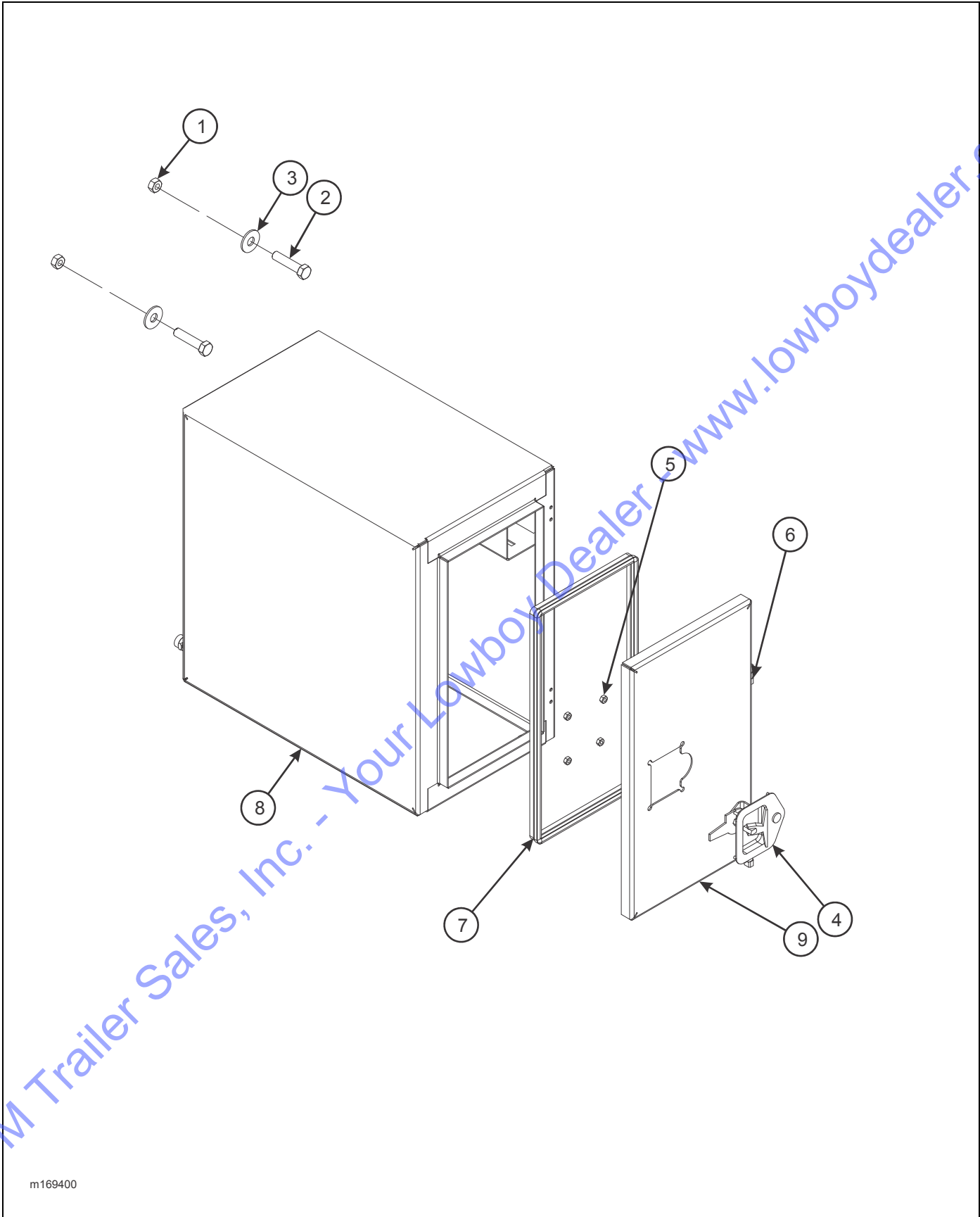
Figure 2-41: Tool Box Installation (Option)
