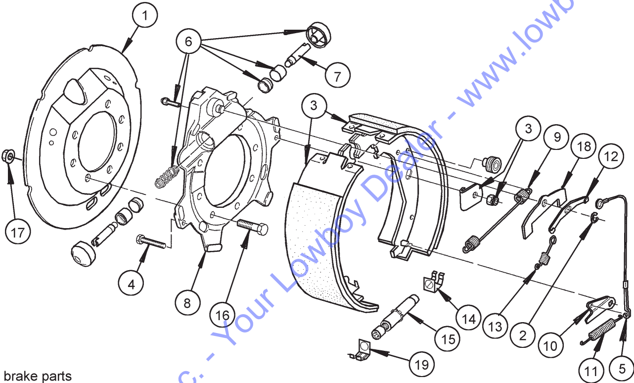
brake parts
