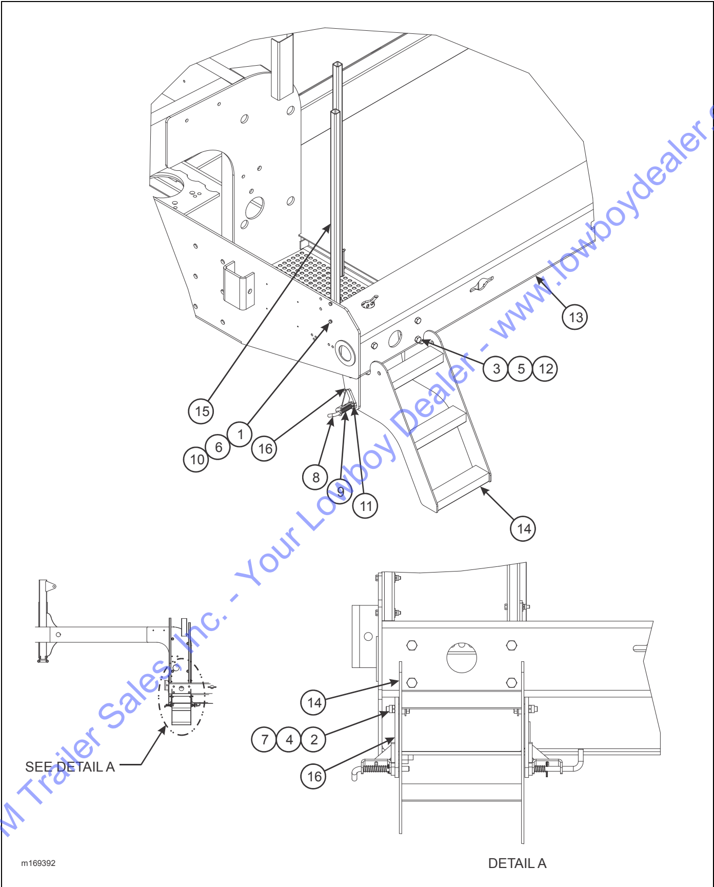
Figure 2-42: Ladder Assembly, Stow-Away Short (Option)
