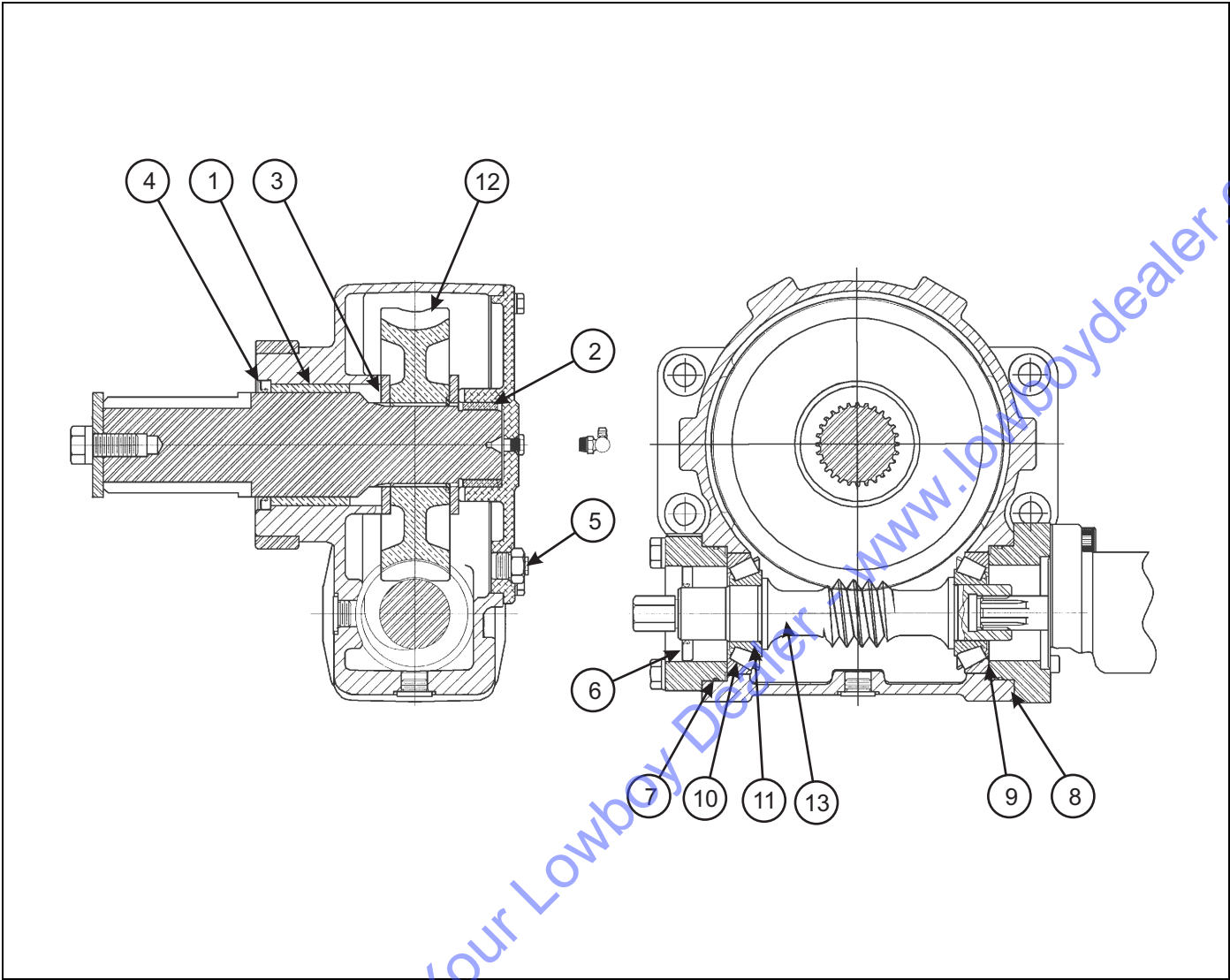
Figure 2-24: Gearbox Items
