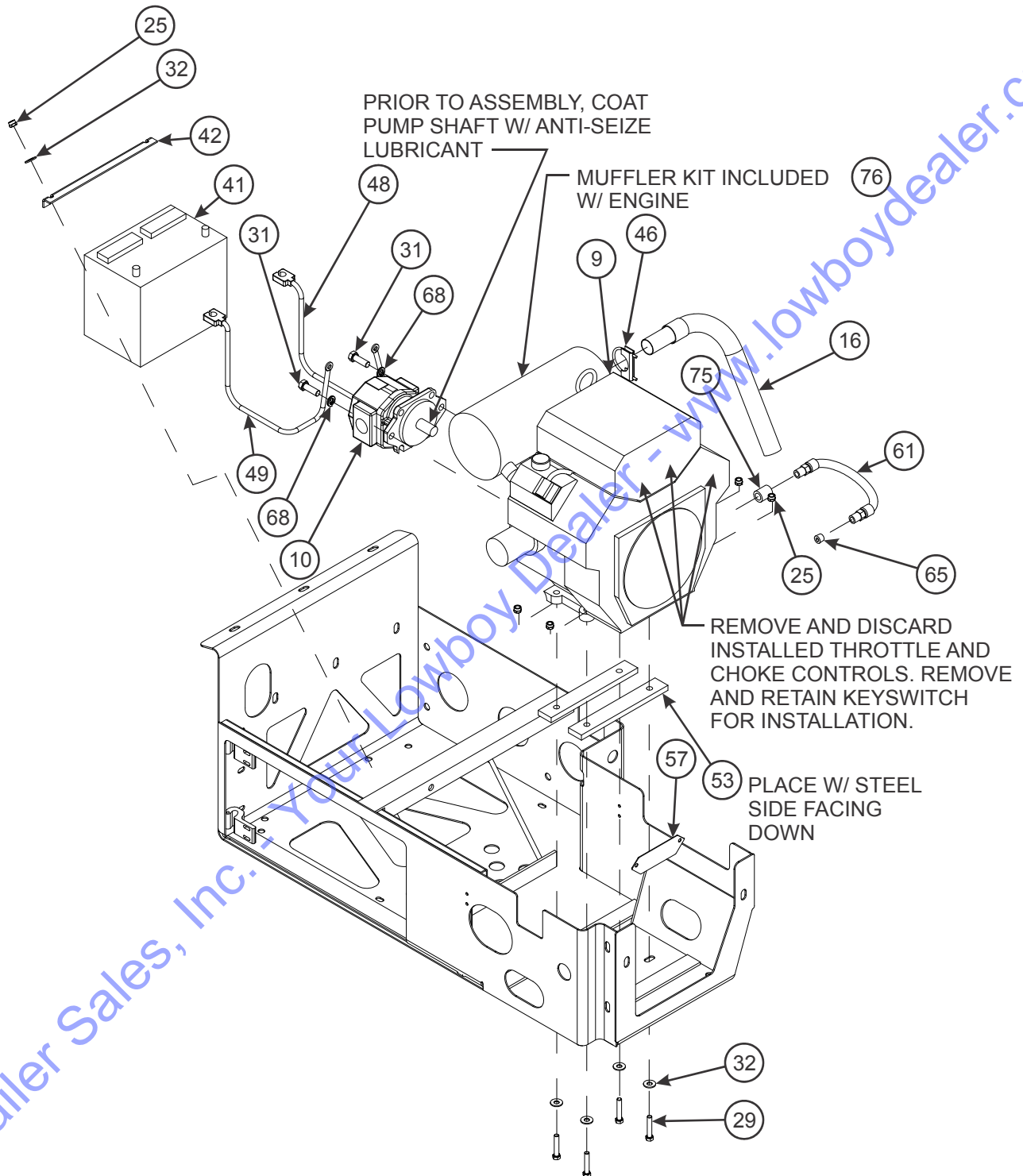
MOTOR - BASE ASSEMBLY
