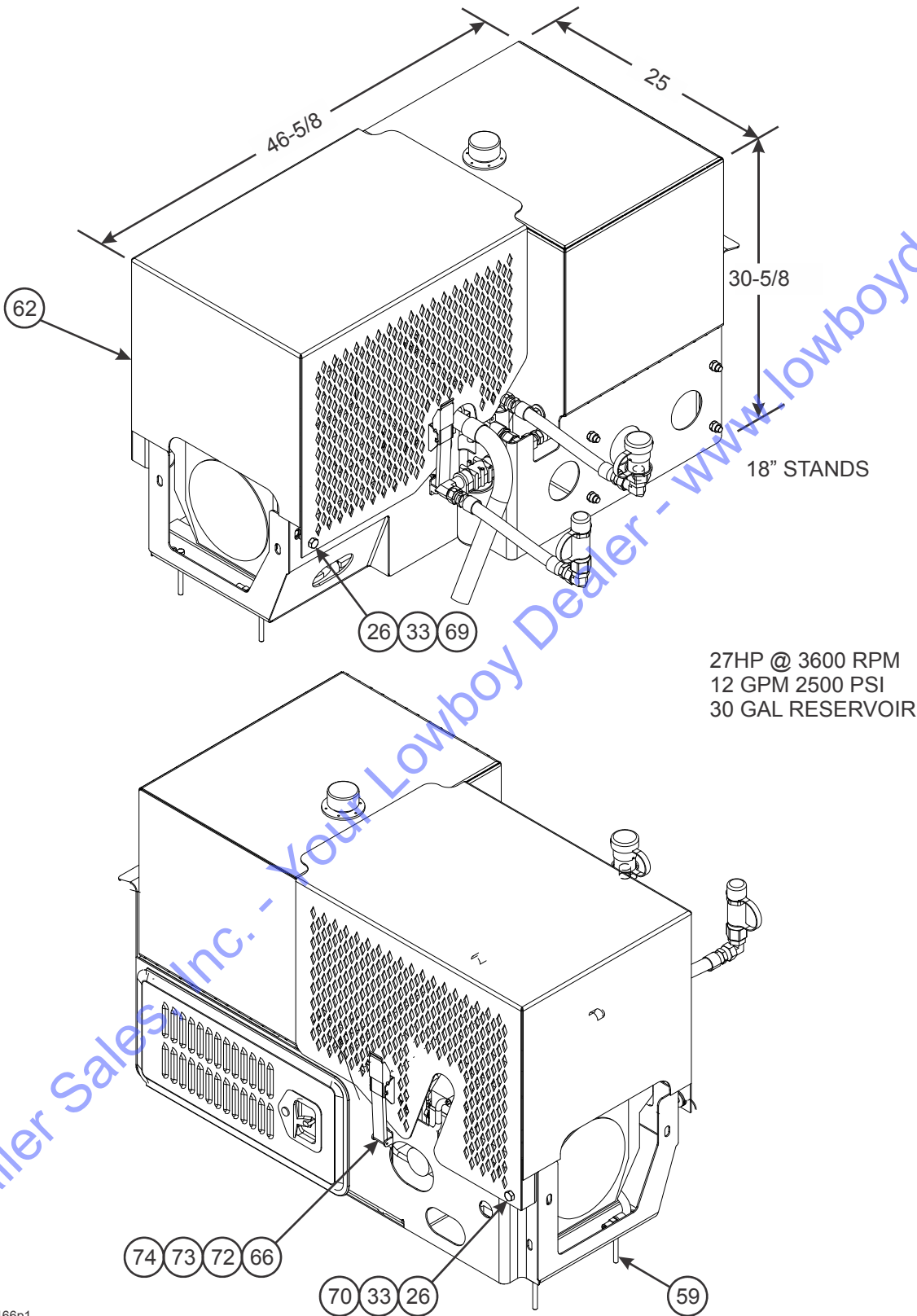
Figure 2-35: Engine Package, Front Mount (1 of 4)
