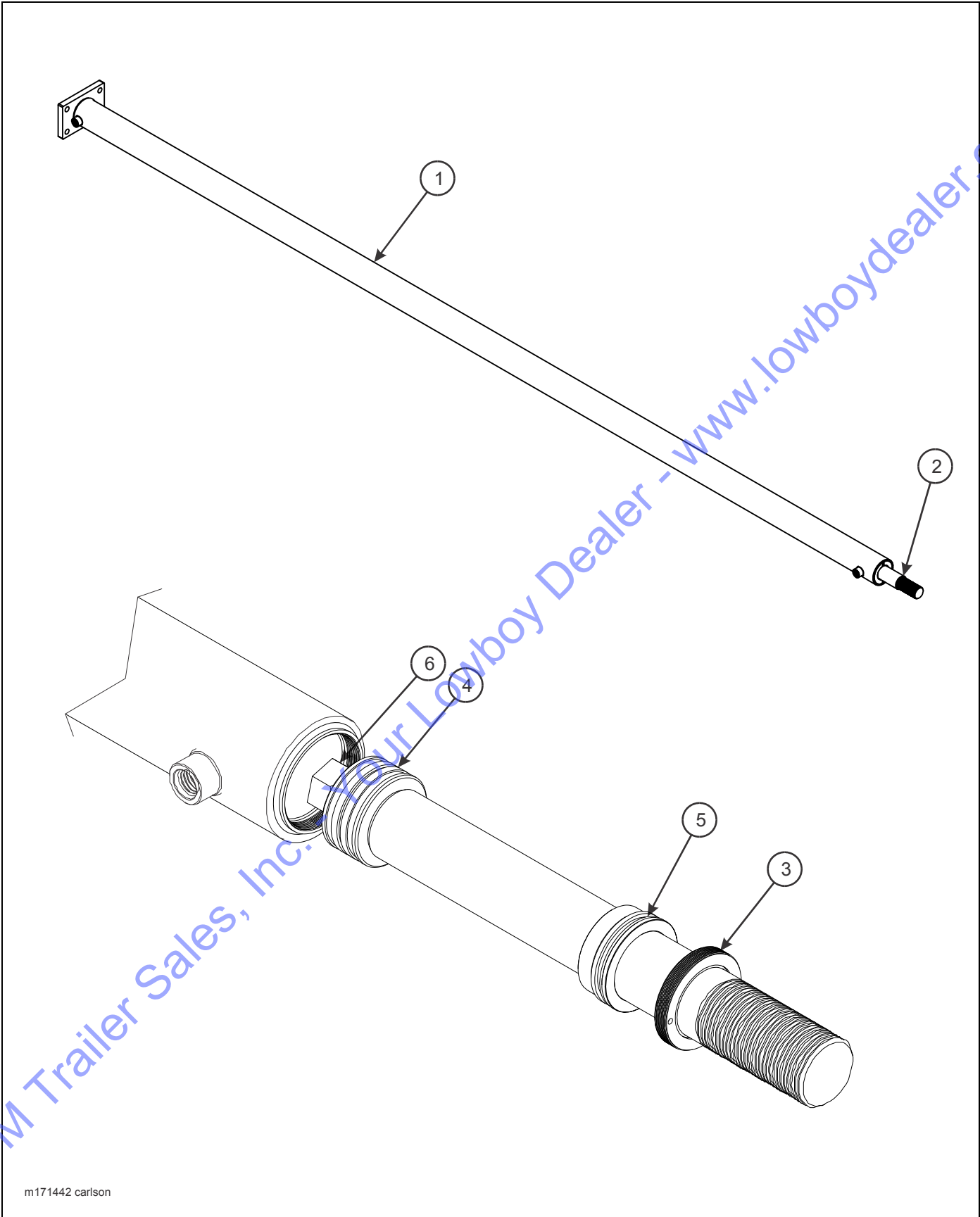
Figure 2-10: 3 X 117 Hydraulic Cylinder (Carlson)
