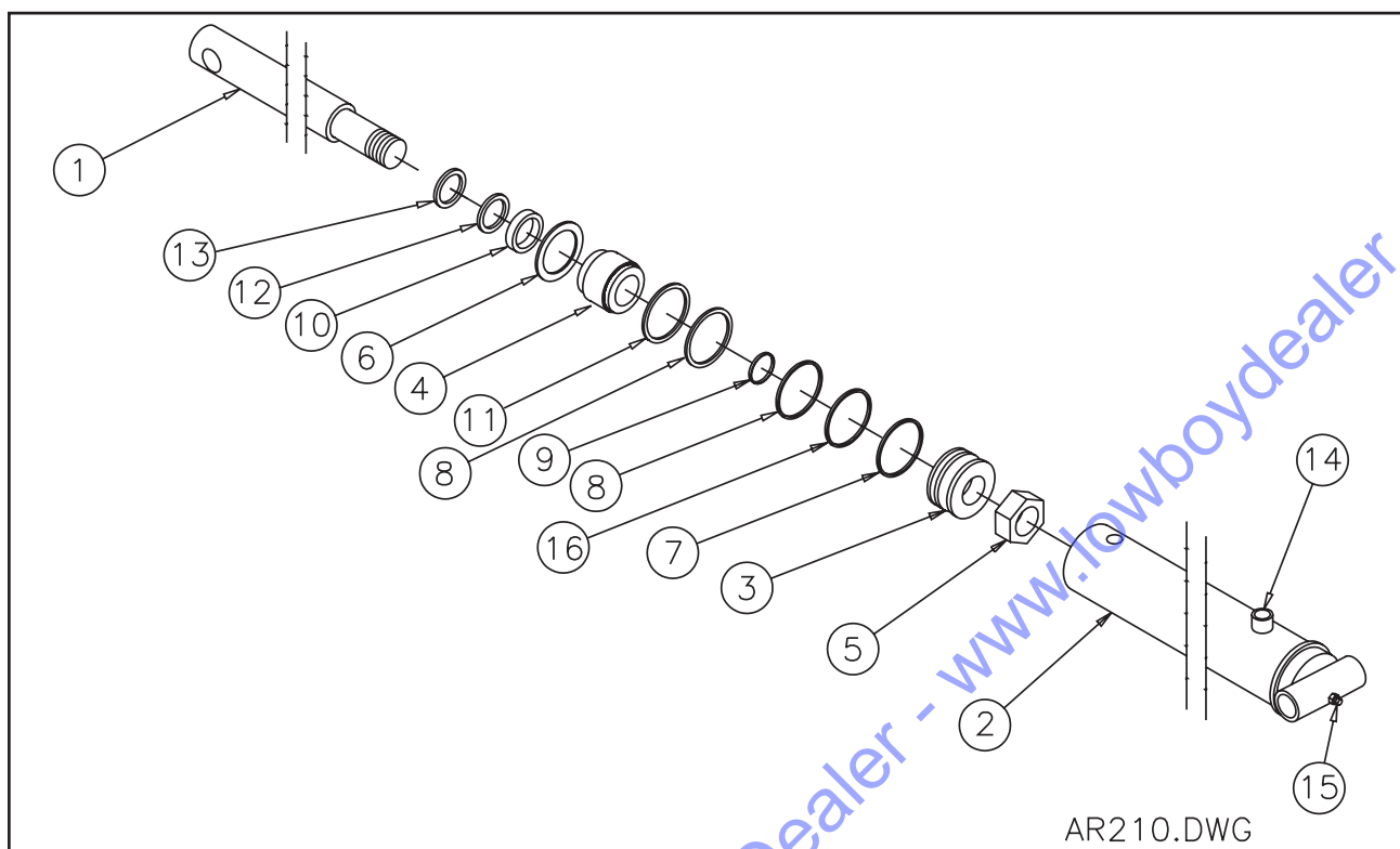
Figure 1-7 4" x 36" Hydraulic Cylinder Assembly
