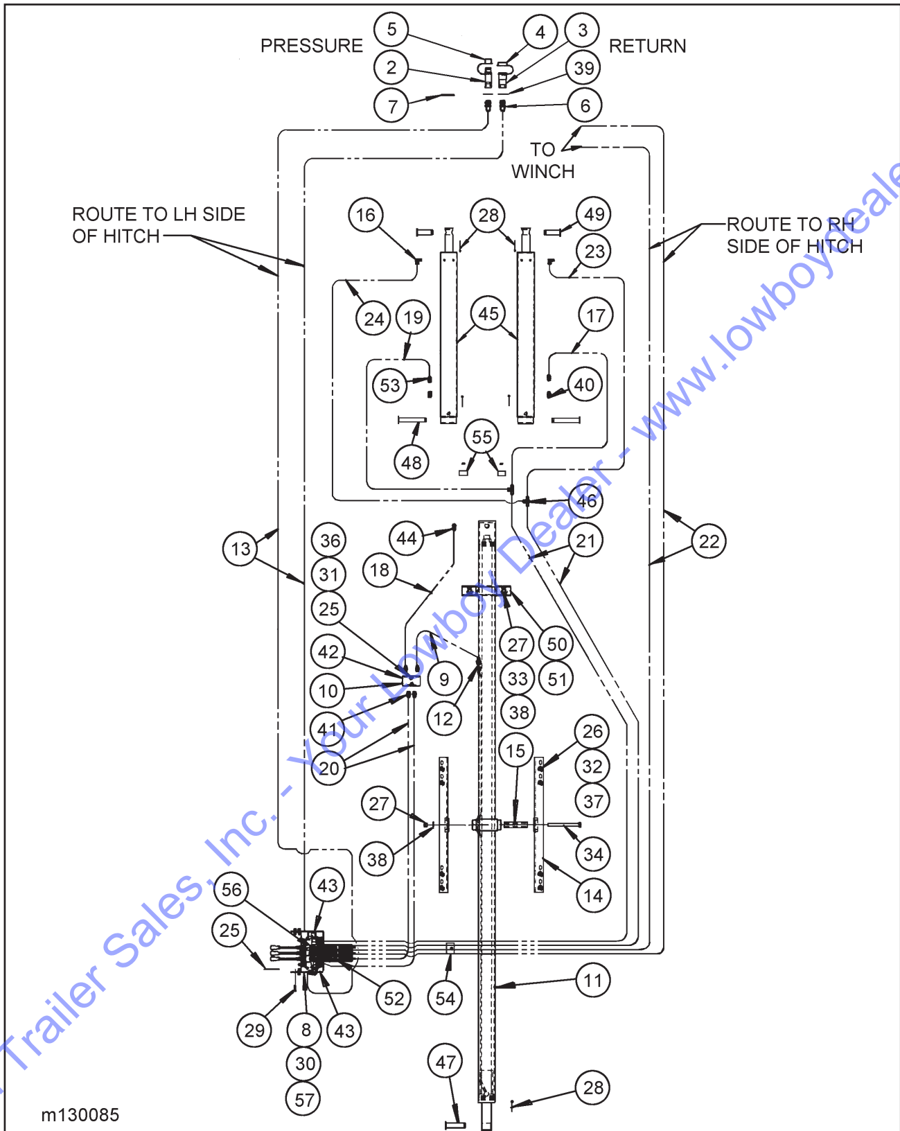
Figure 1-5 Hydraulic System
