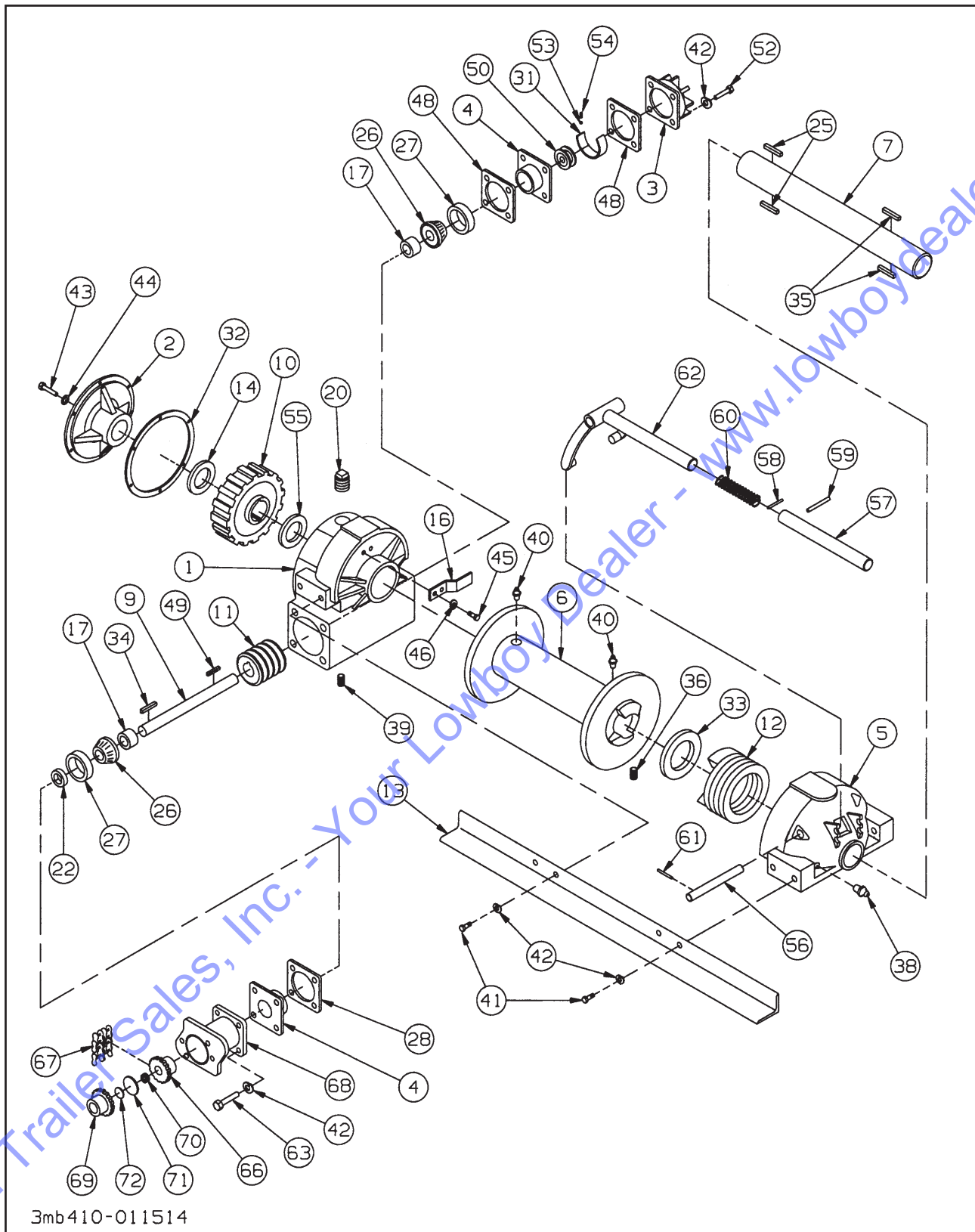
Figure 1-17 12,000 # Winch Items
