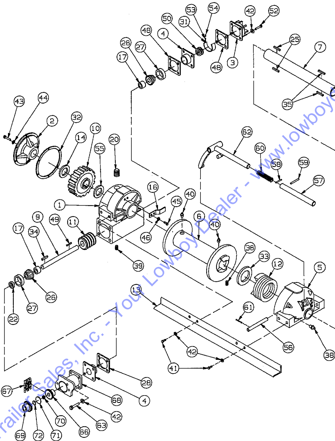
Figure 1-23 12,000# Winch Assembly
