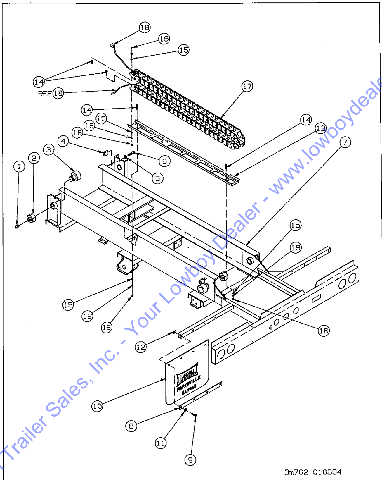
Figure 1-10 Undercarriage Assembly
