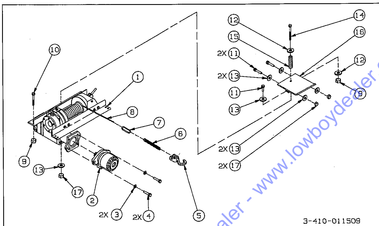
Figure 1-22 Winch Installation
