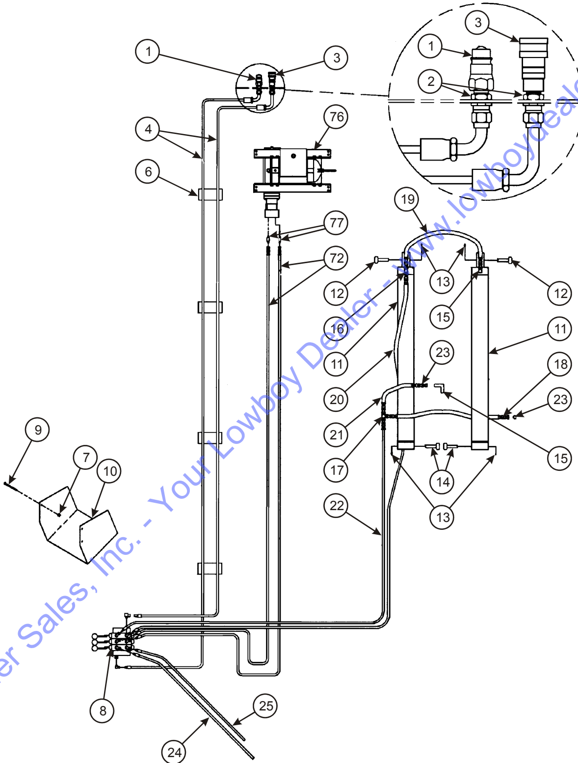
Figure 2-6: Hydraulic System (1 of 3)
