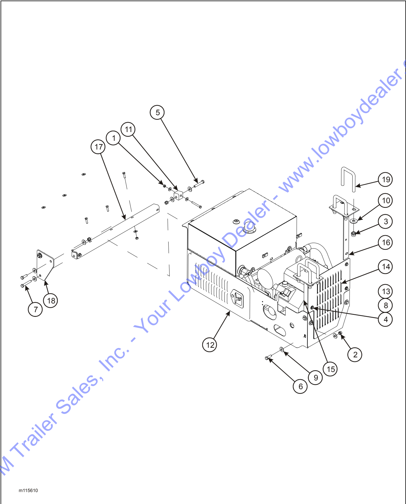
Figure 2-59: Underslung Engine Package Installation
