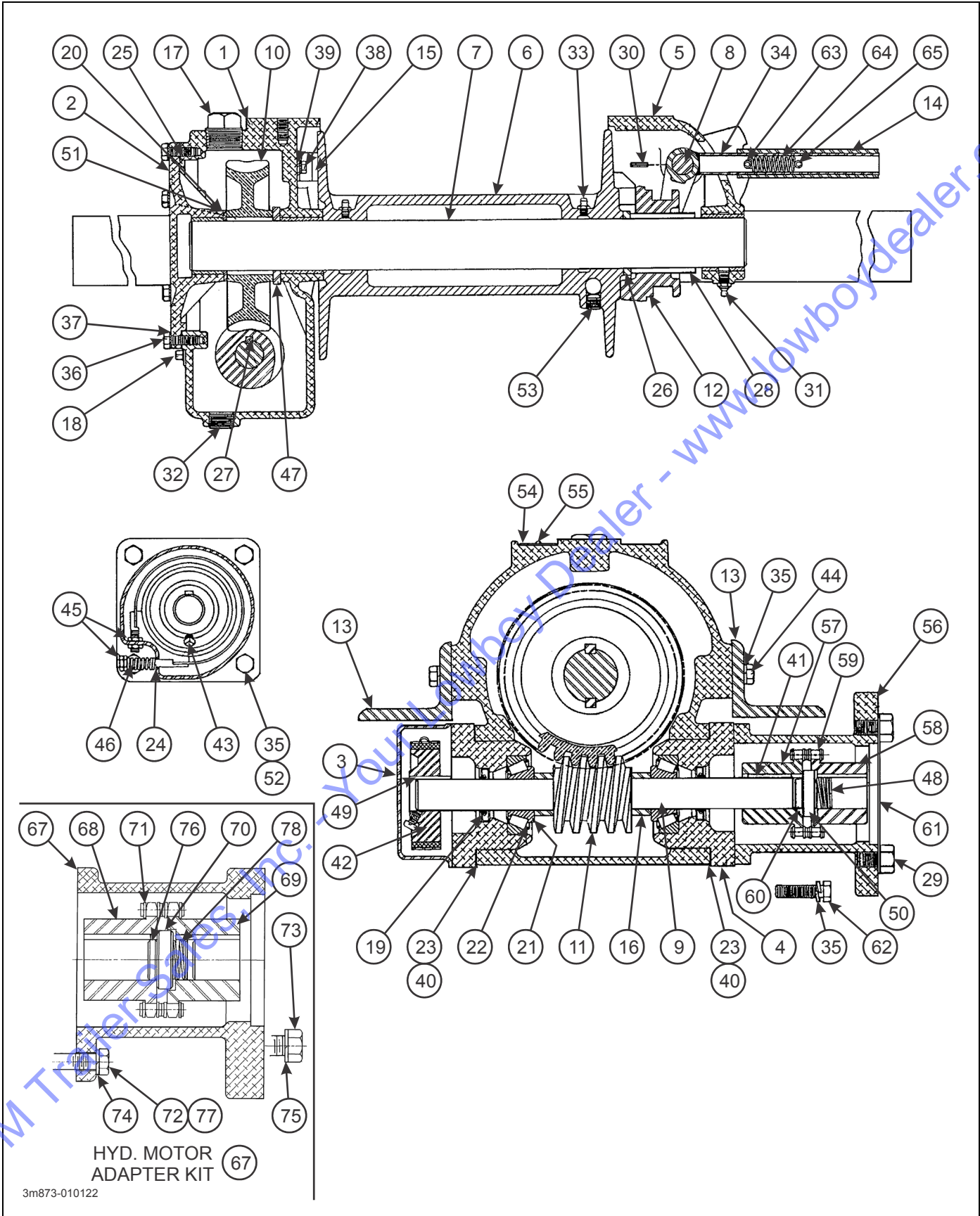
Figure 2-38: 12,000 Lb. Winch Items
