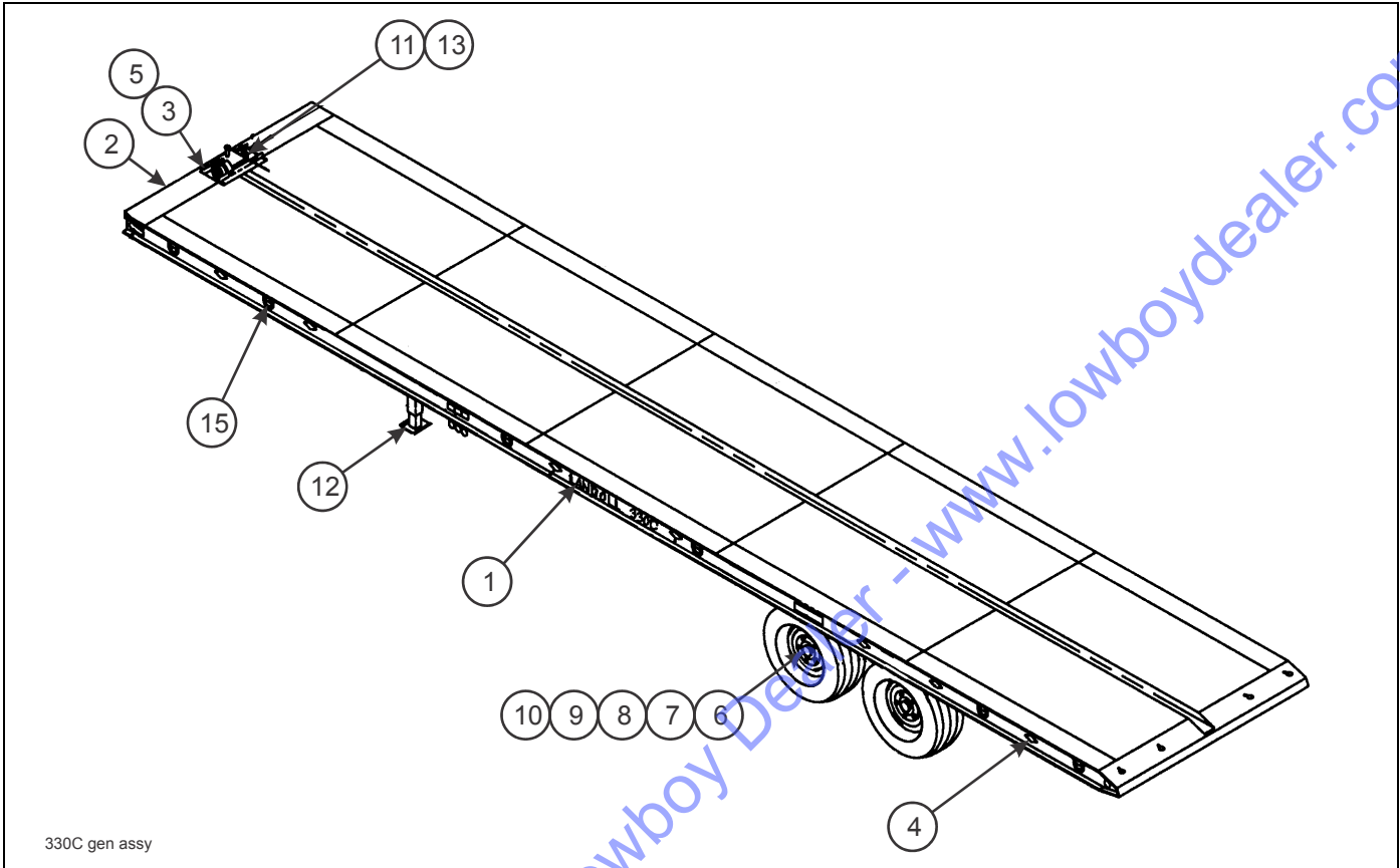
Figure 2-1: General Assembly
