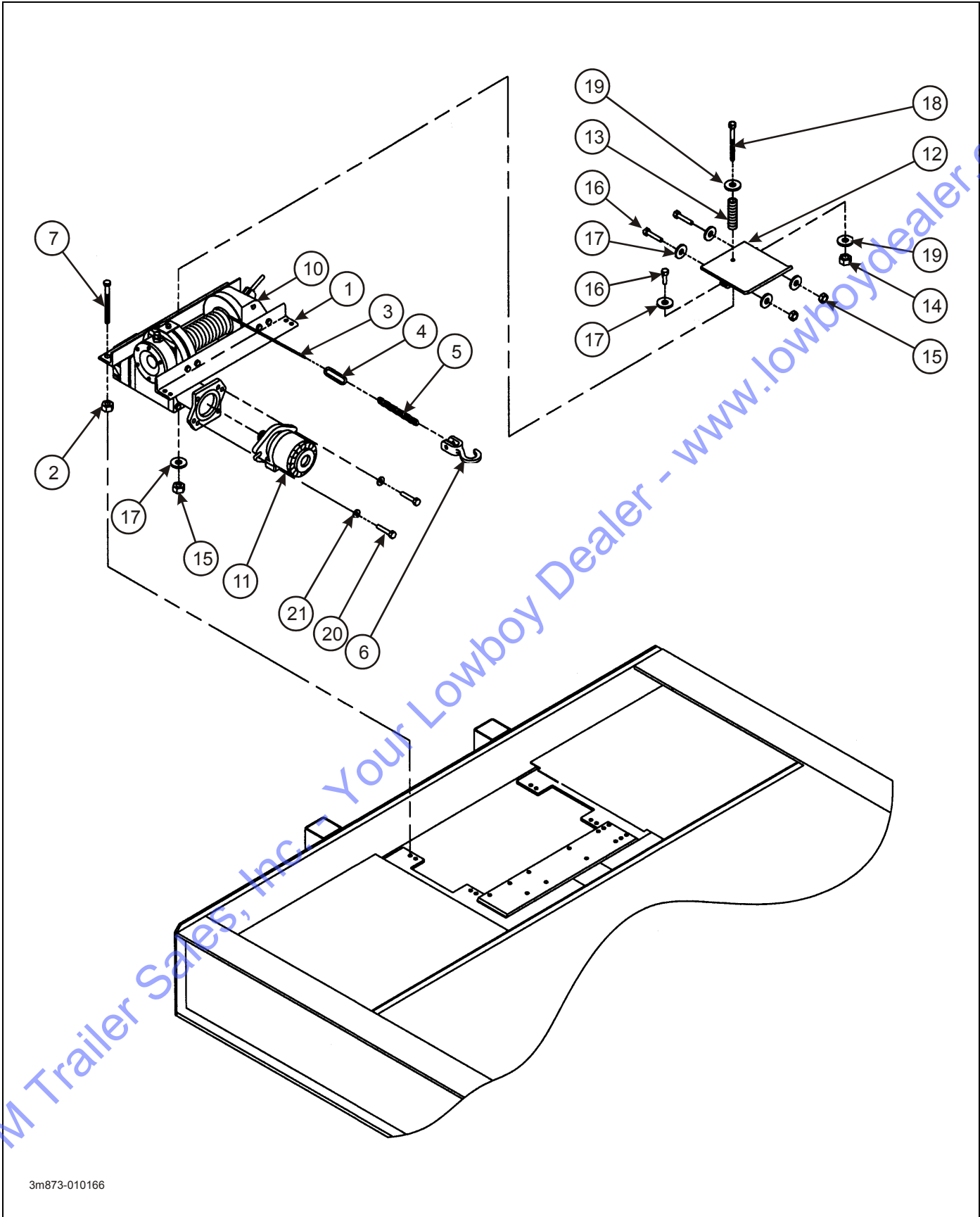
Figure 2-37: Winch Installation
