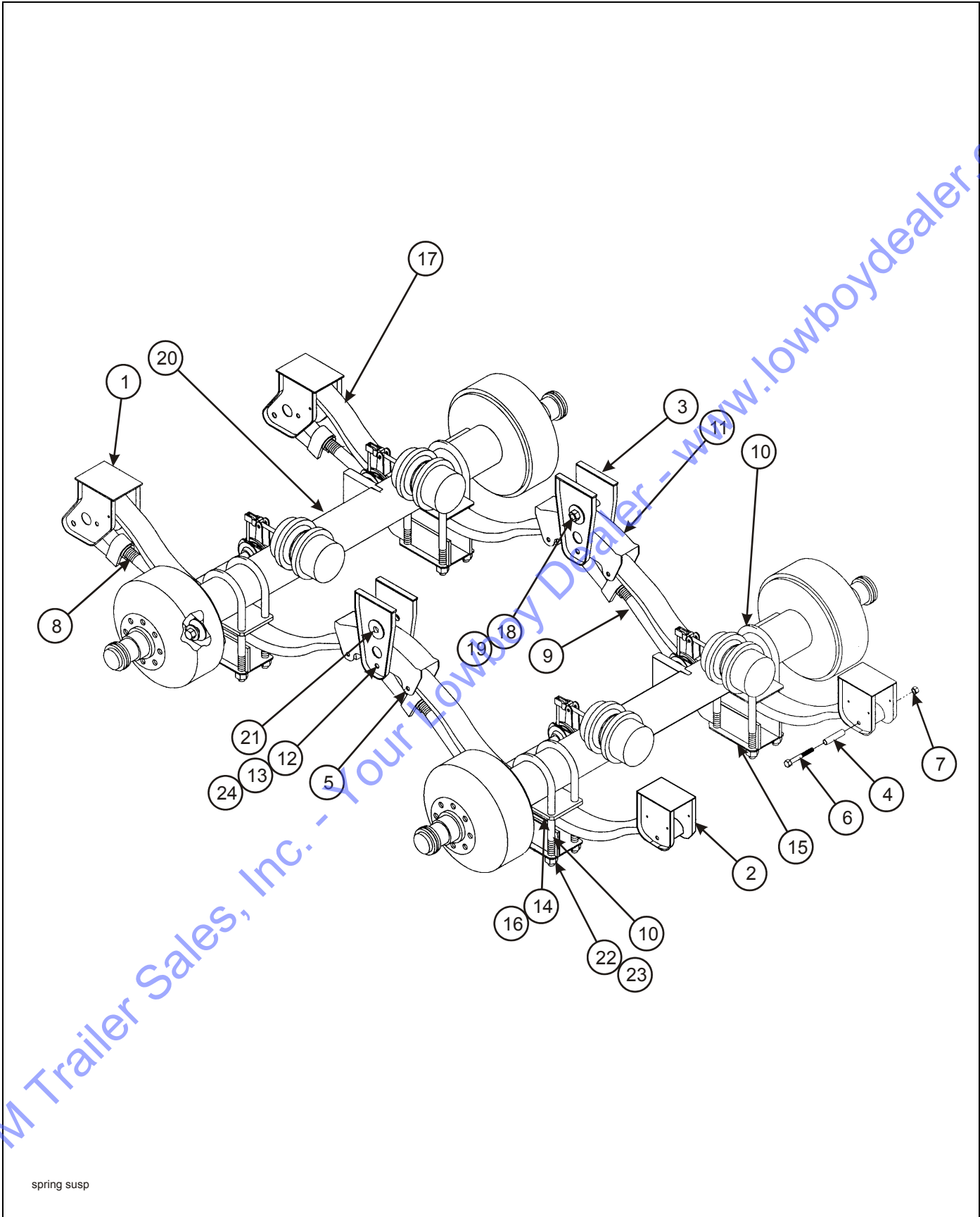
Figure 2-25: Single Leaf Spring Suspension (Tandem Axle Shown)
