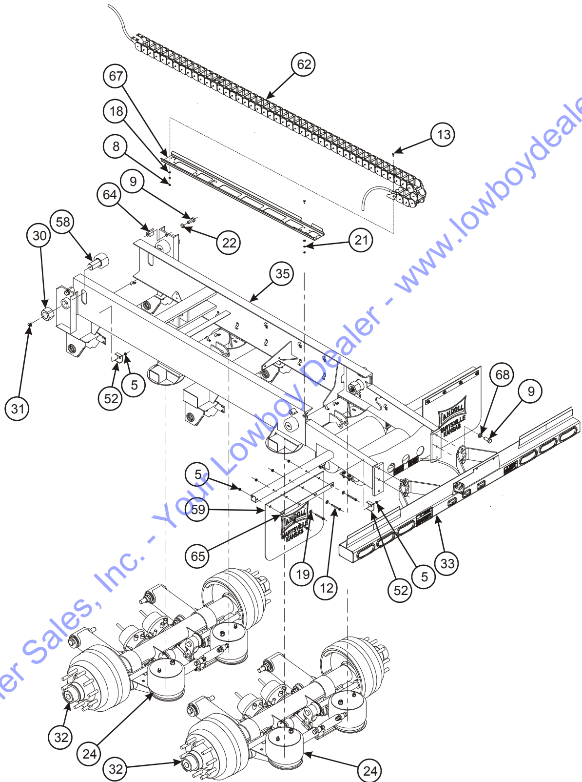
Figure 2-27: Undercarriage Assembly, Air Ride Tandem Axle
