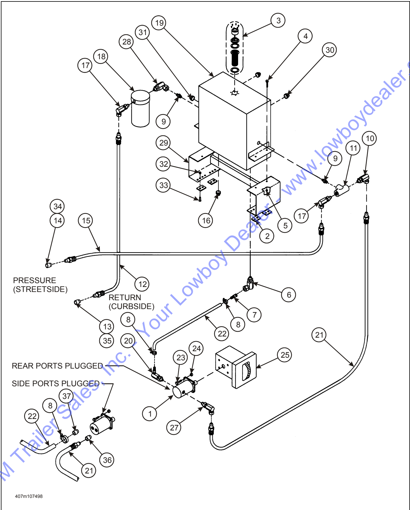
Figure 2-56: Hydraulic Wet Kit Assembly (Option)
