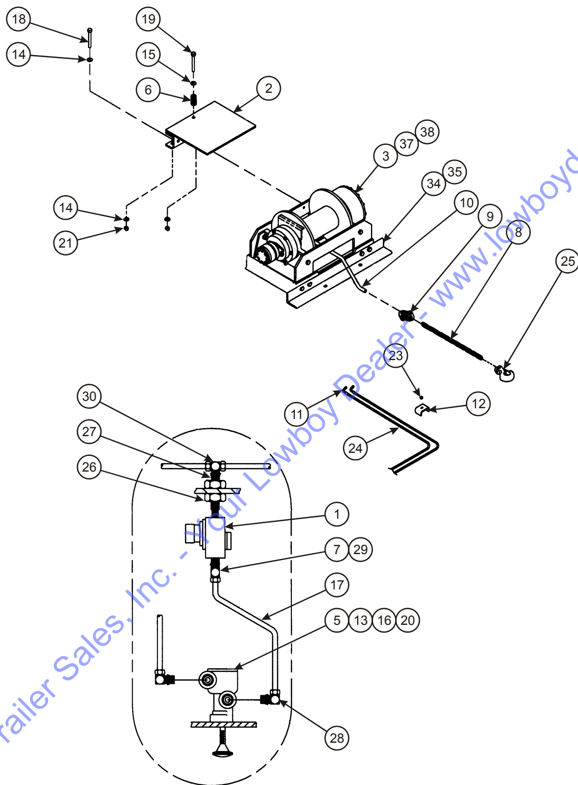
Figure 2-46: Winch Installation, 30,000 Lb. (DP)
