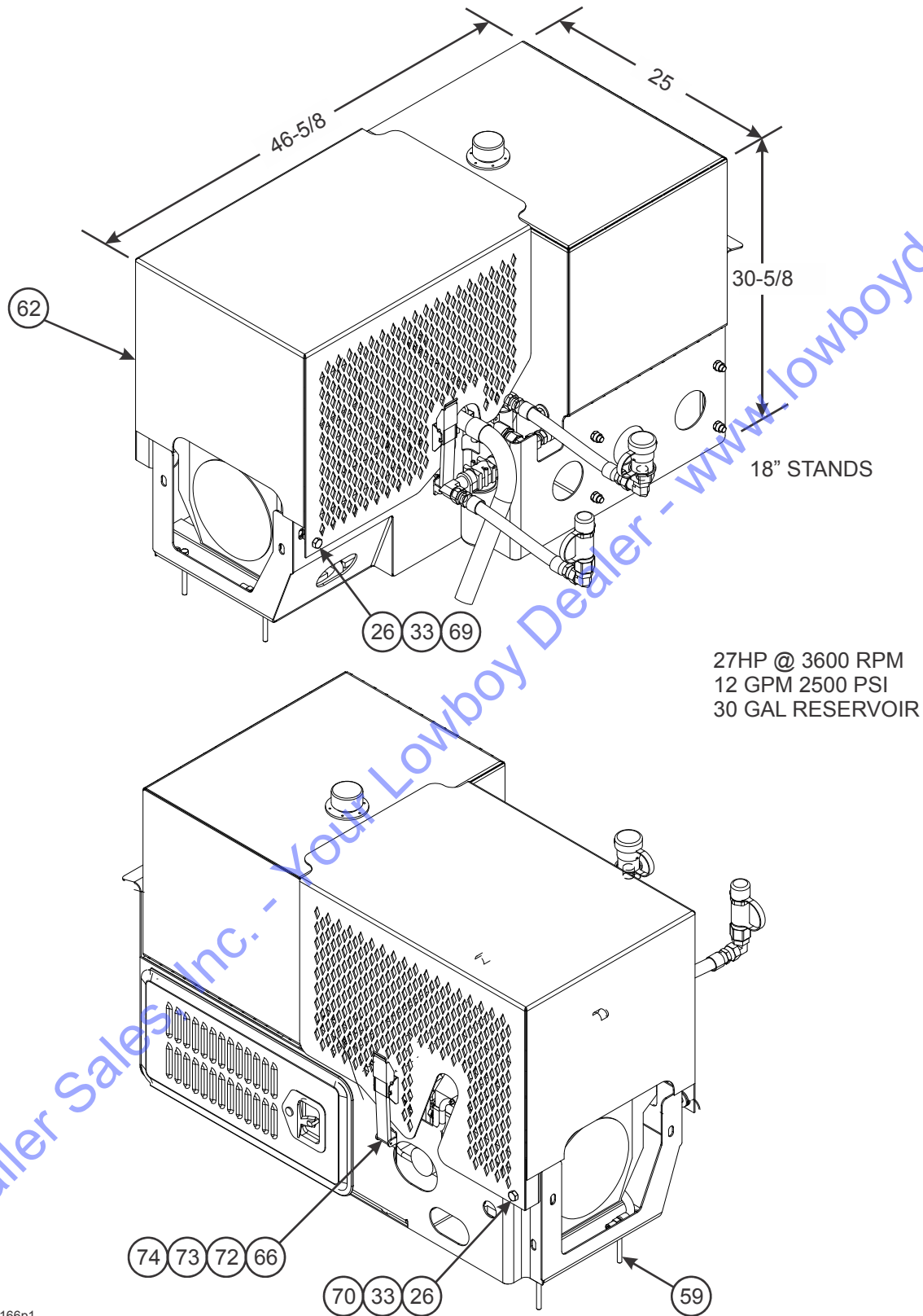
Figure 2-60: Engine Package, Front Mount (1 of 4)
