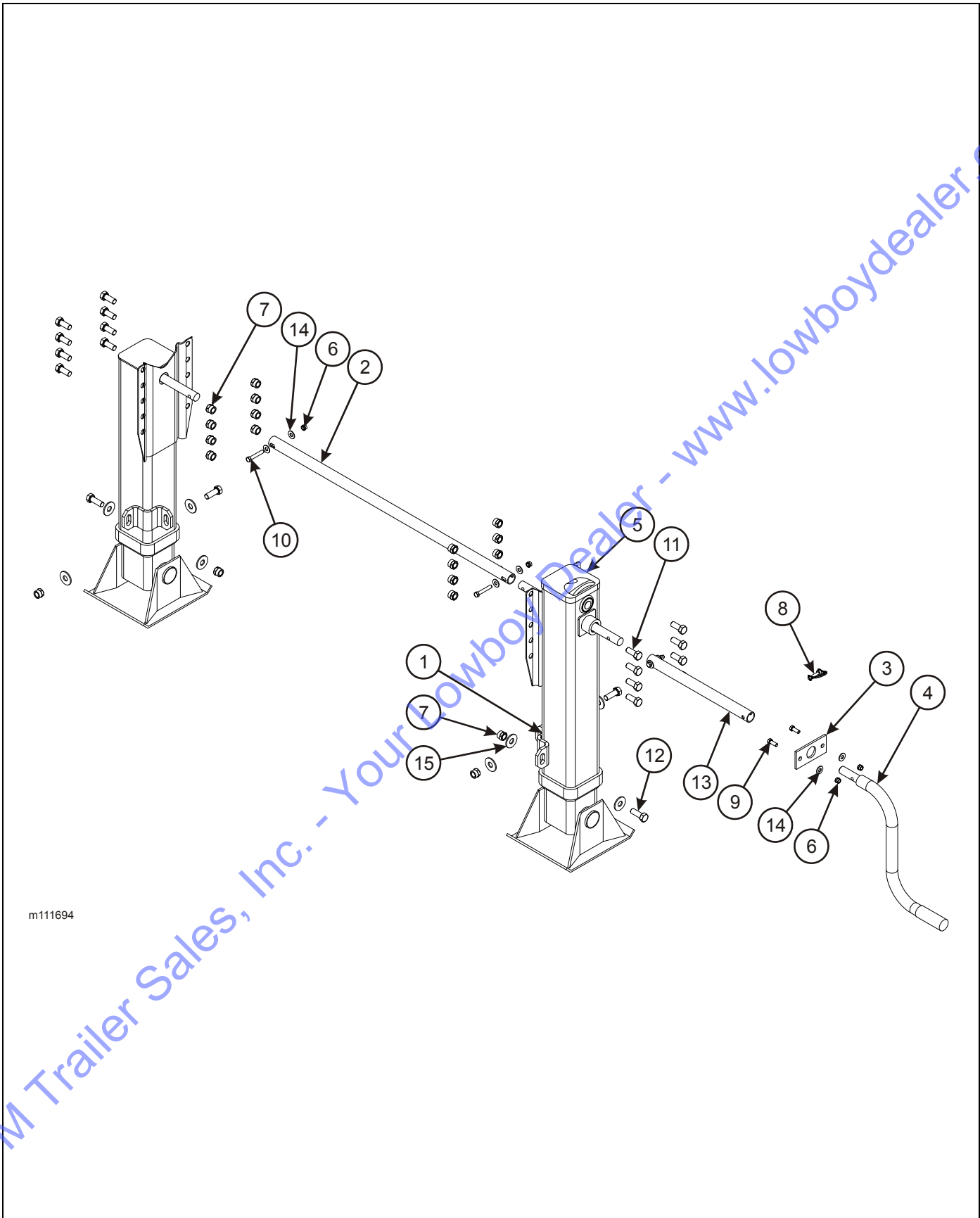
Figure 2-54: Landing Gear Installation
