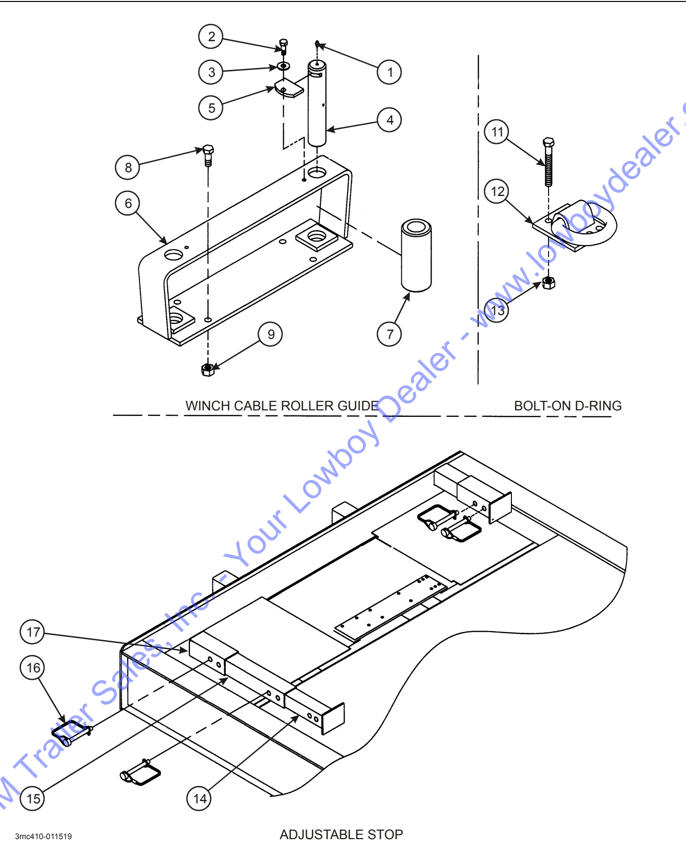
Figure 2-48: Winch Cable Roller Guide (Option)
