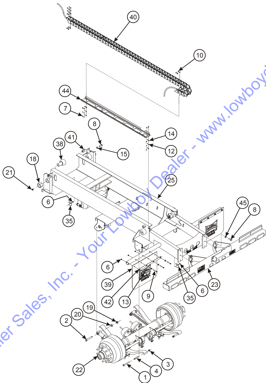
Figure 2-21: Undercarriage Assembly, Spring Ride Single Axle
