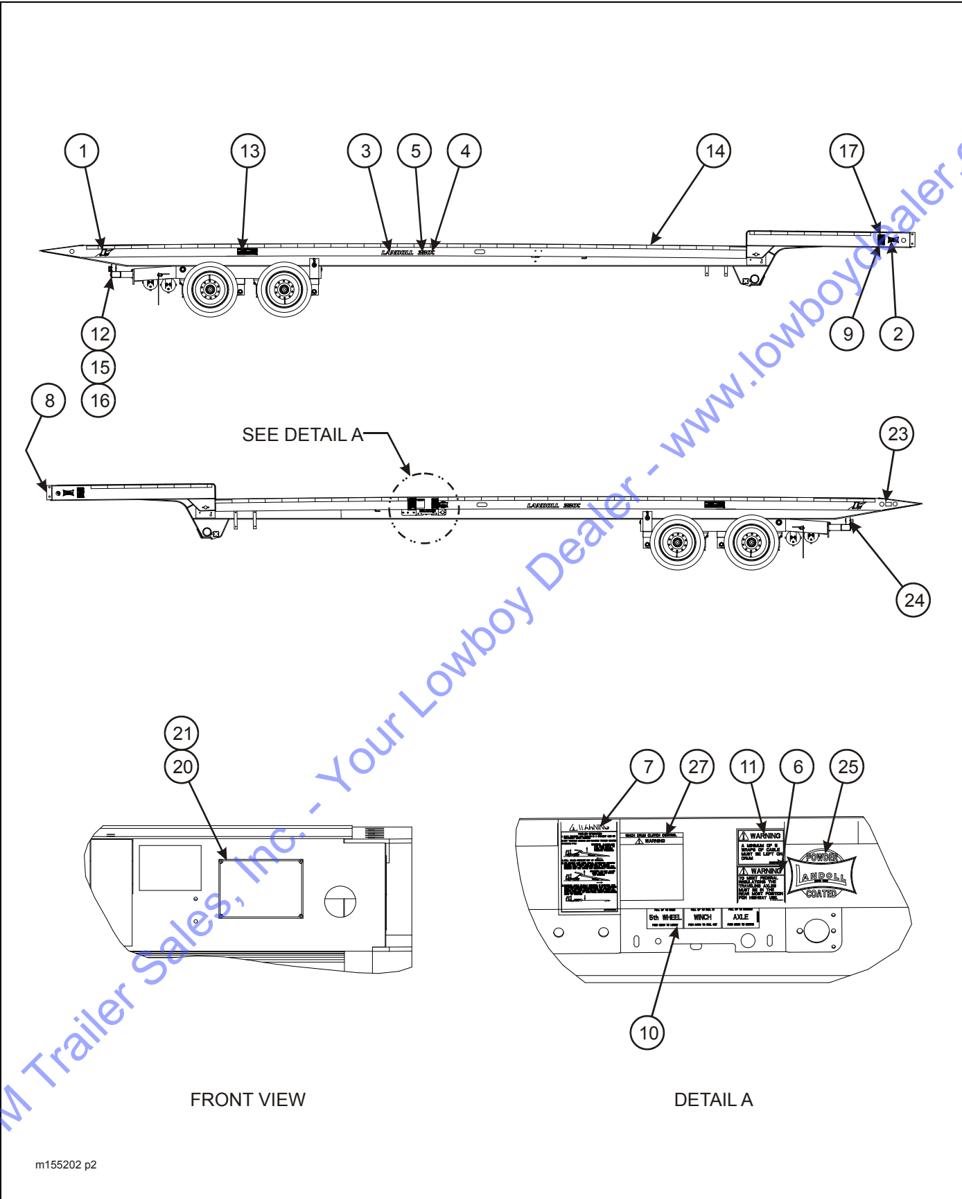
Figure 2-4: Decal Placement, Tandem Axle
