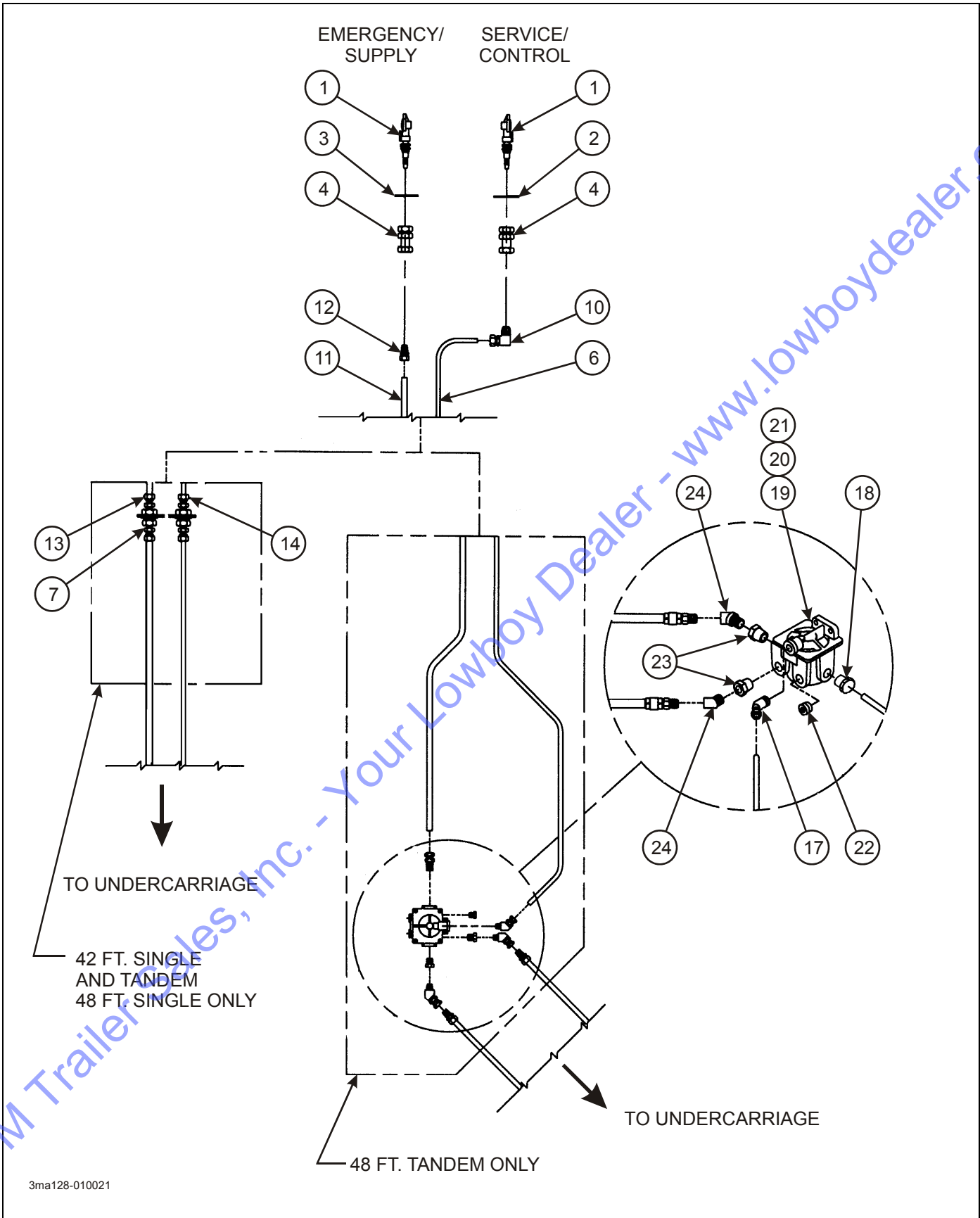
Figure 2-16: Air System
