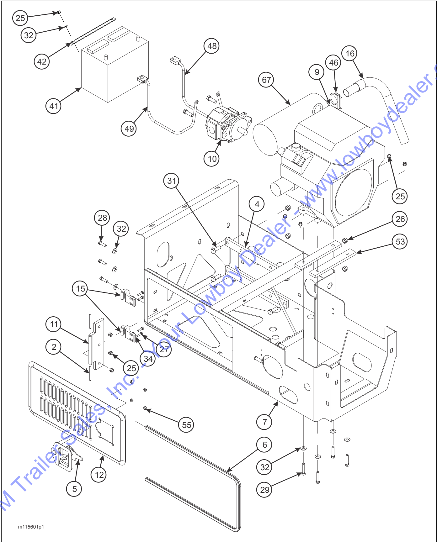
Figure 2-57: Engine Package, Front Mount (1 of 2)
