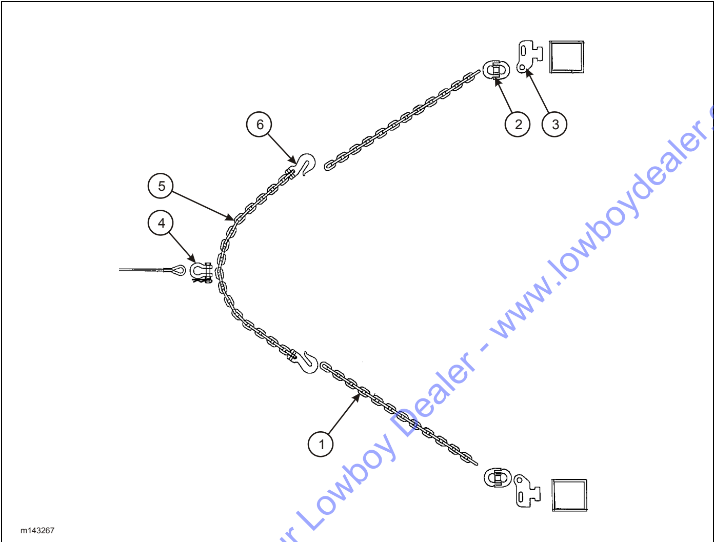
Figure 2-52: Container Chain and Bridle Assembly (Option)
