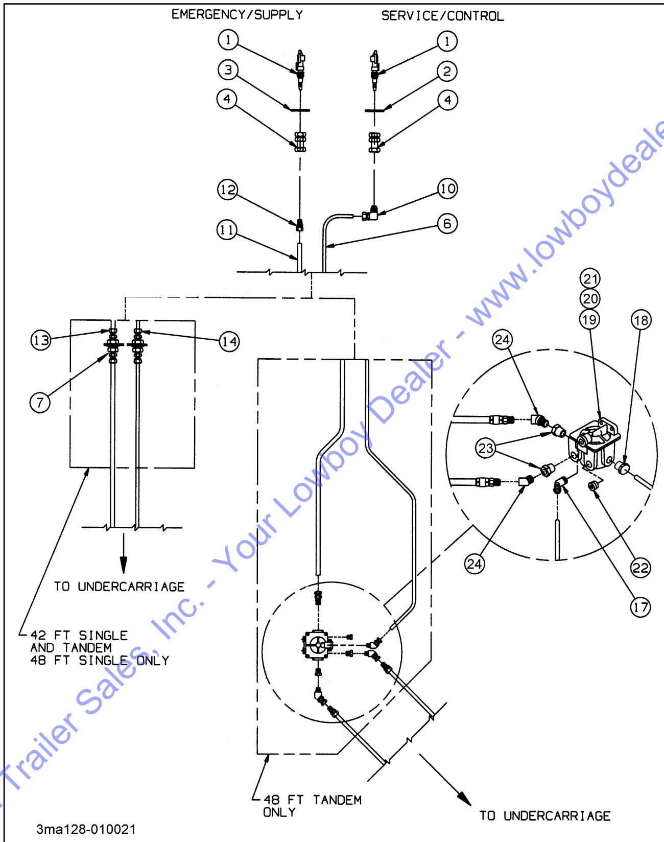
Figure 1-30 Air System
