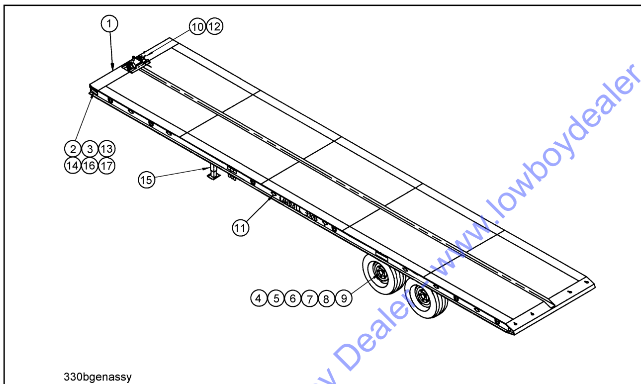
Figure 1-1 General Assembly
