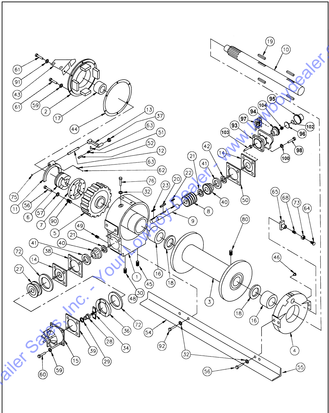
Figure 1-33 20,000# Winch Assembly
