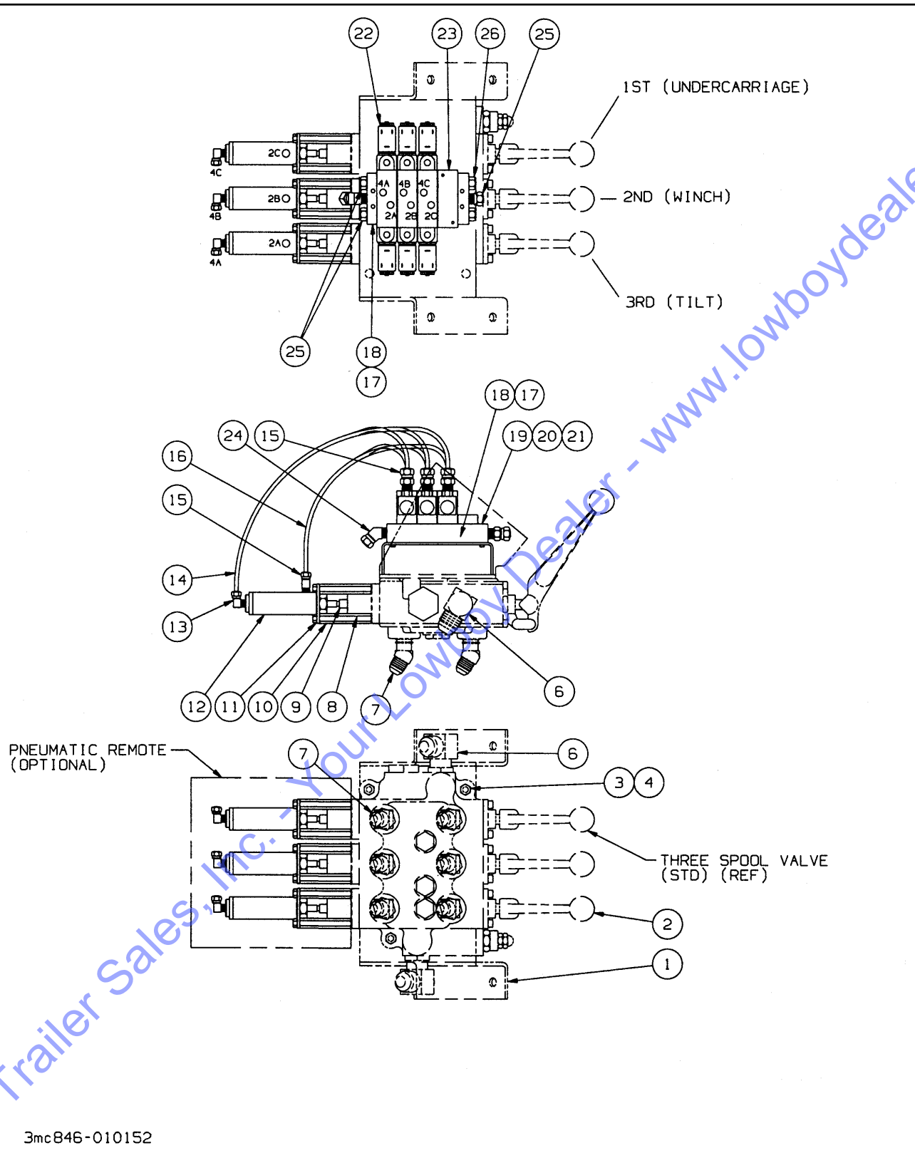
Figure 1-8 Valve Assembly, Three Spool
