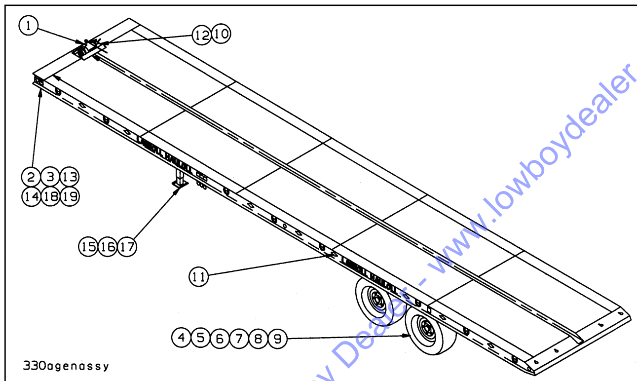
Figure 1-1 General Assembly
