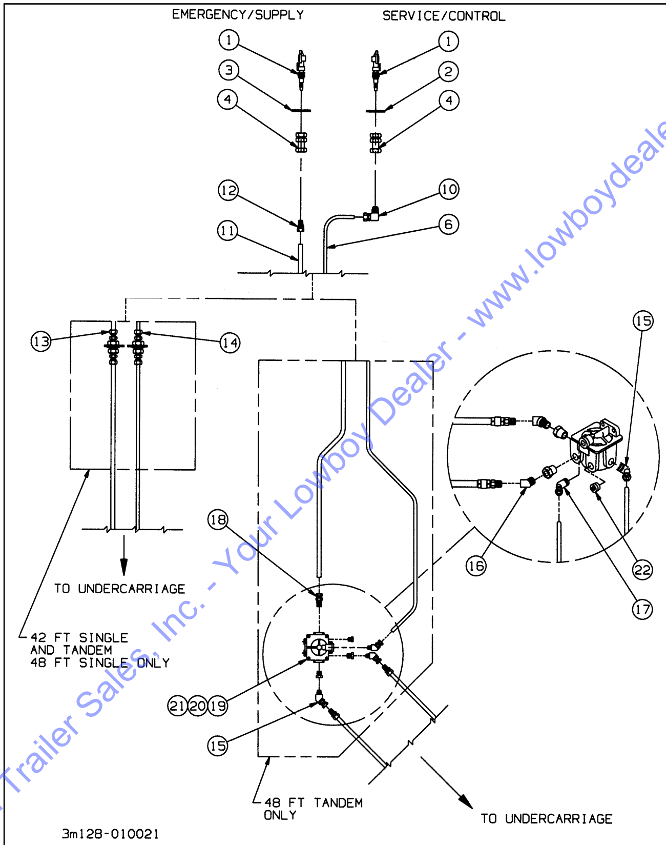
Figure 1-29 Air System
