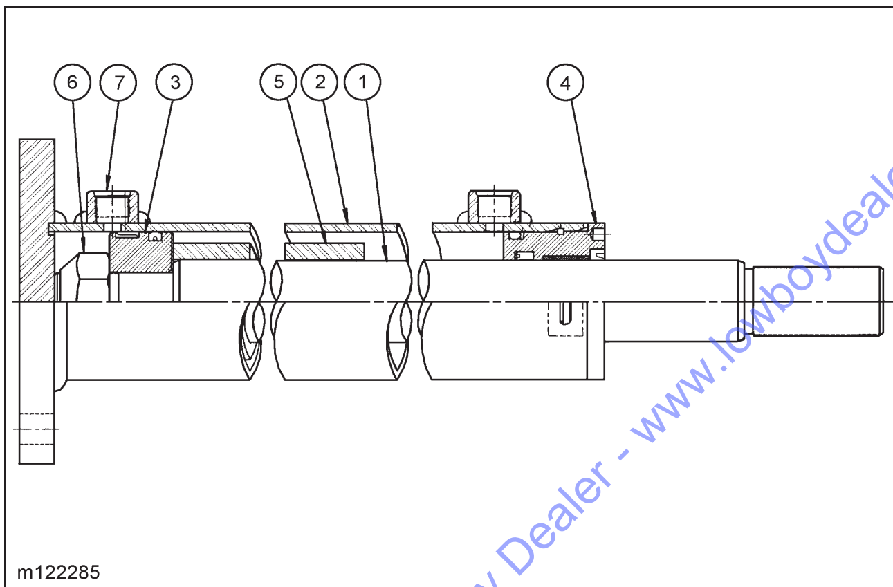
Figure 1-5 3 x 108 Hydraulic Cylinder Assembly
