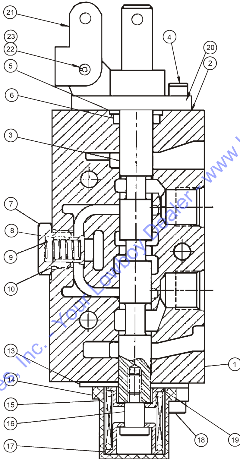
Figure 1-8 Six Spool Valve, Work Section
