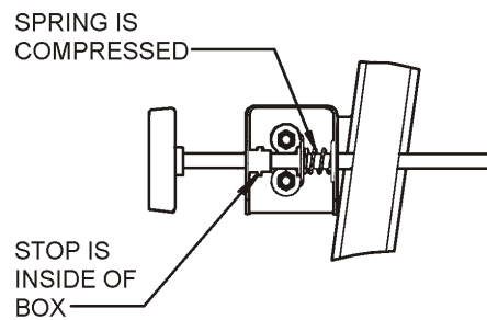
DISENGAGED VIEW
