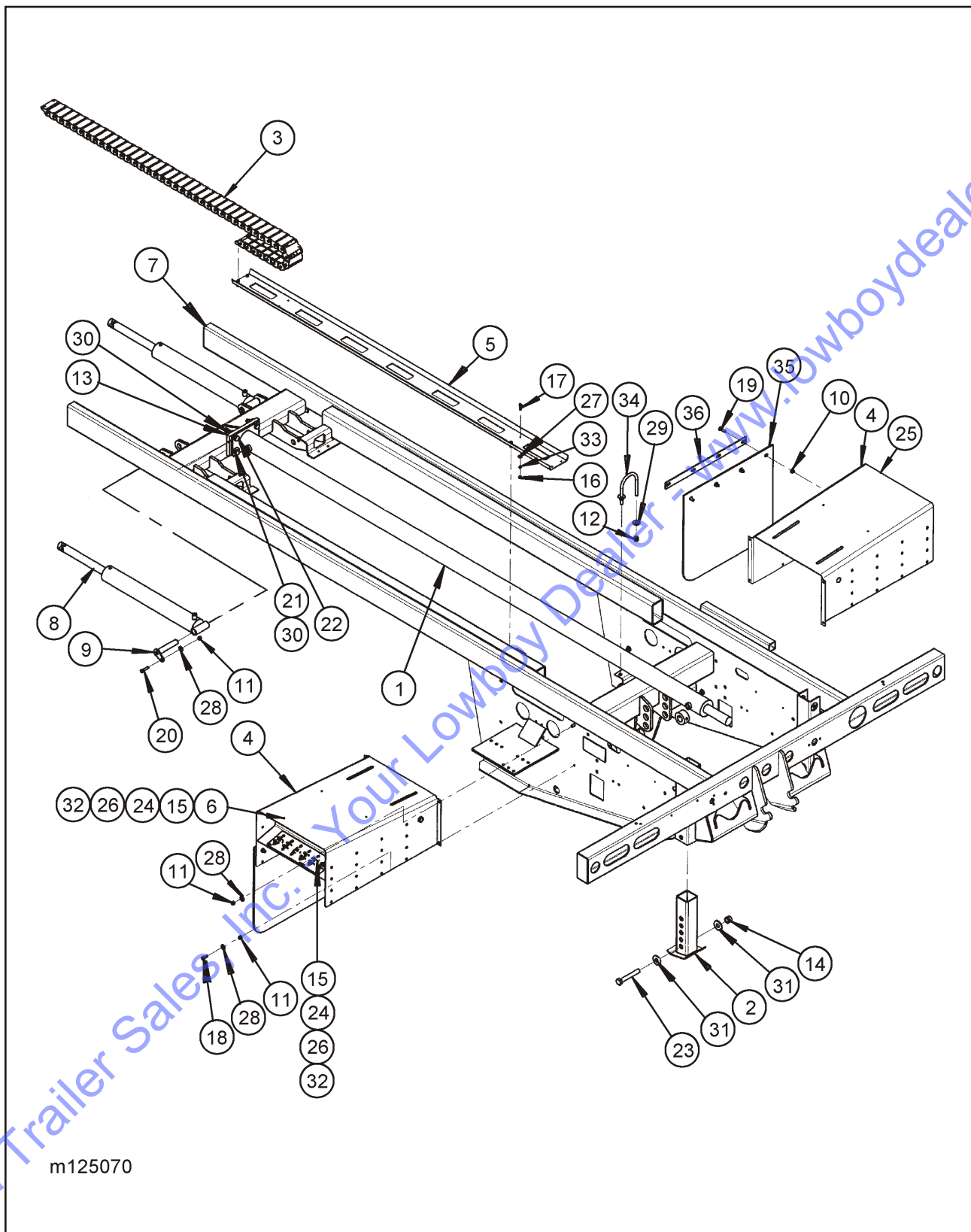
Figure 1-2 Frame Assembly
