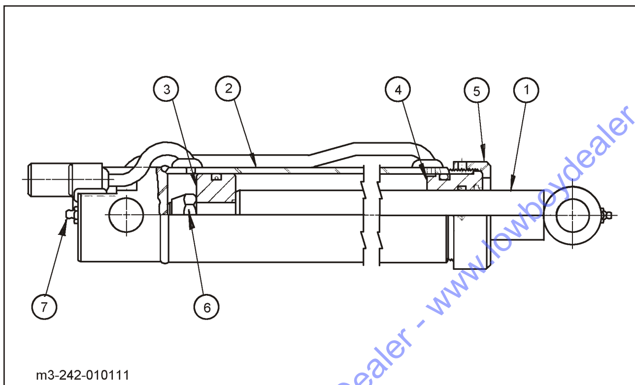
Figure 1-17 2-1/2 x 63 Hydraulic Cylinder Assembly
