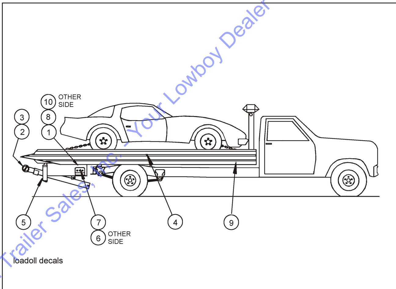
Figure 1-36 Decal Placement
