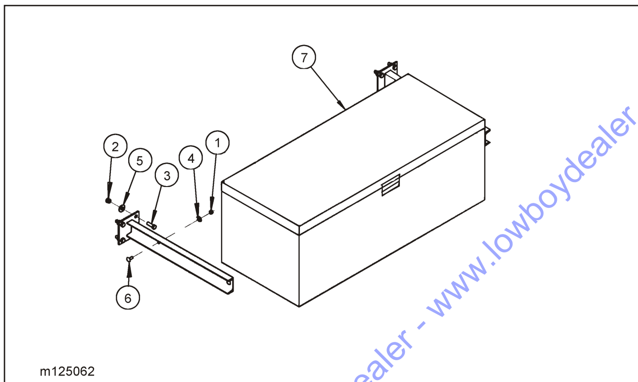
Figure 1-33 Toolbox Assembly
