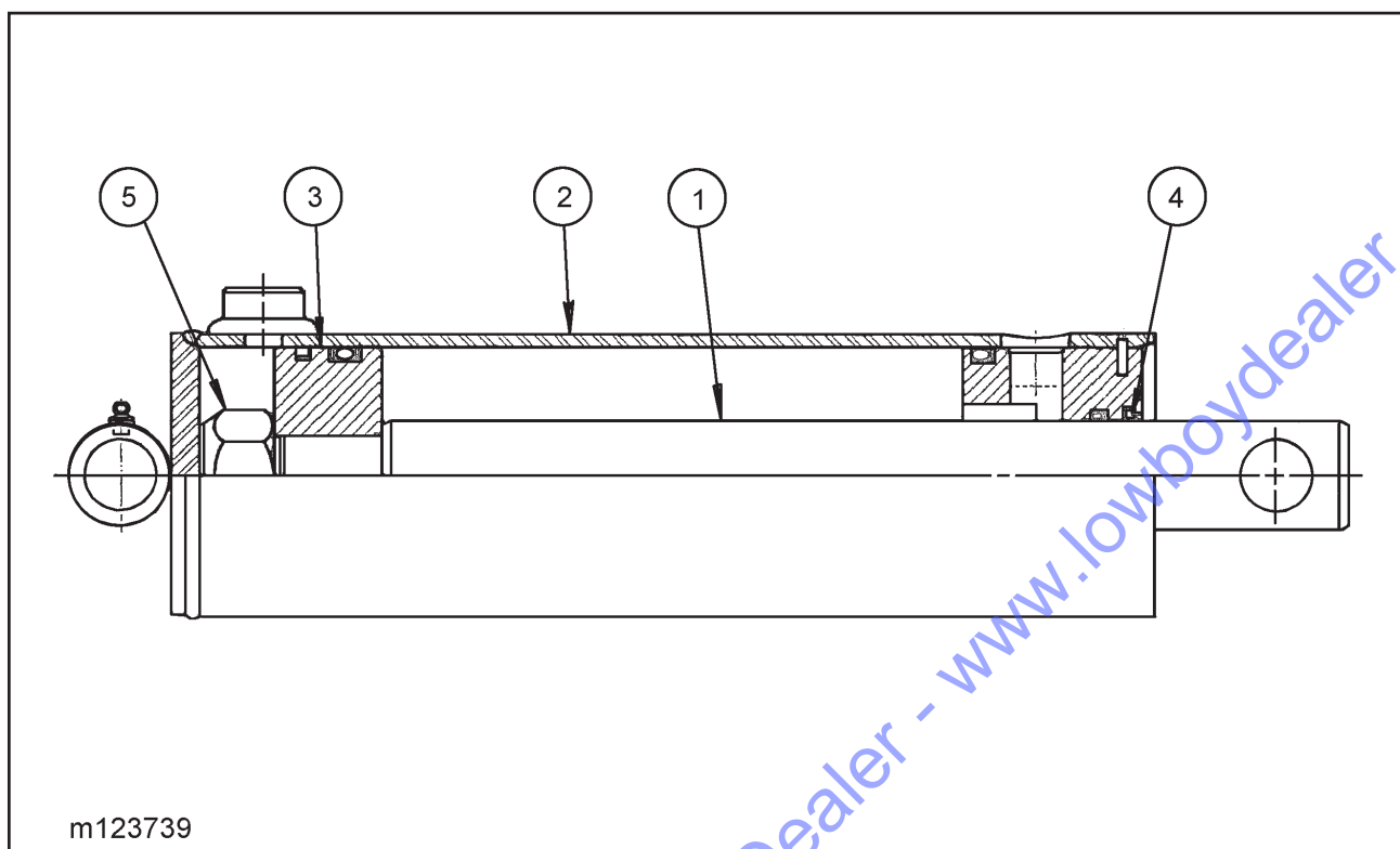
Figure 1-6 4 x 20 Hydraulic Cylinder Assembly
