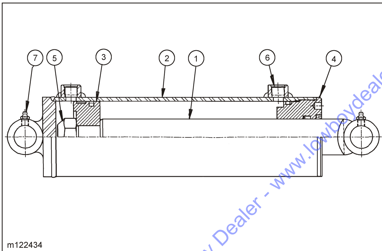
Figure 1-16 4 x 10 Hydraulic Cylinder Assembly
