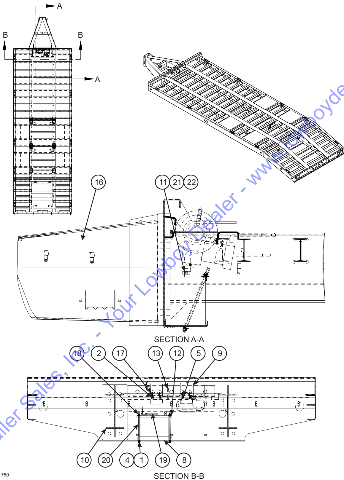
Figure 1-22 Winch Assembly
