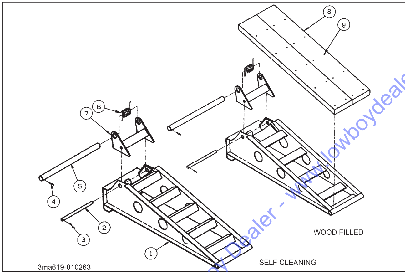
Figure 1-14 Ramp Assembly
